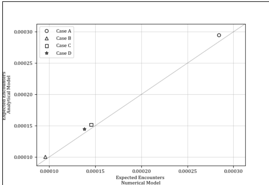
Figure 13. Comparison between the analytical and numerical models Expected number of encounters along a 1-km route segment. Four cases were evaluated, differentiated by the relative speeds or sizes of the vessel and animal. For all cases, animal density was assumed to be 0.003 animals per square kilometer, and the relative heading of the animal and vessel was 90^\circ . Parameters corresponding to the four cases are summarized in Table 4 . A 1:1 trendline is plotted for comparison.
