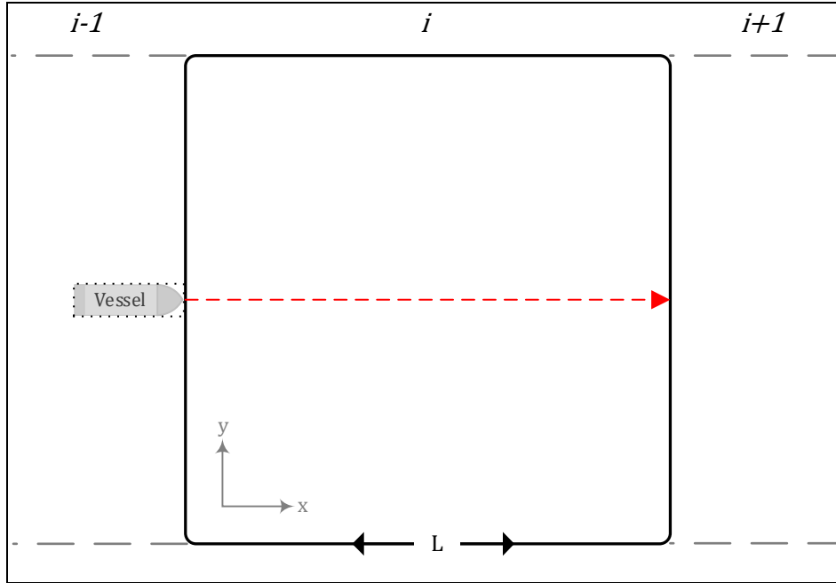
Figure 4. Plan view diagram of the L \times L square domain (shown in black) centered about a single ( i^{th} ) segment of the vessel route
