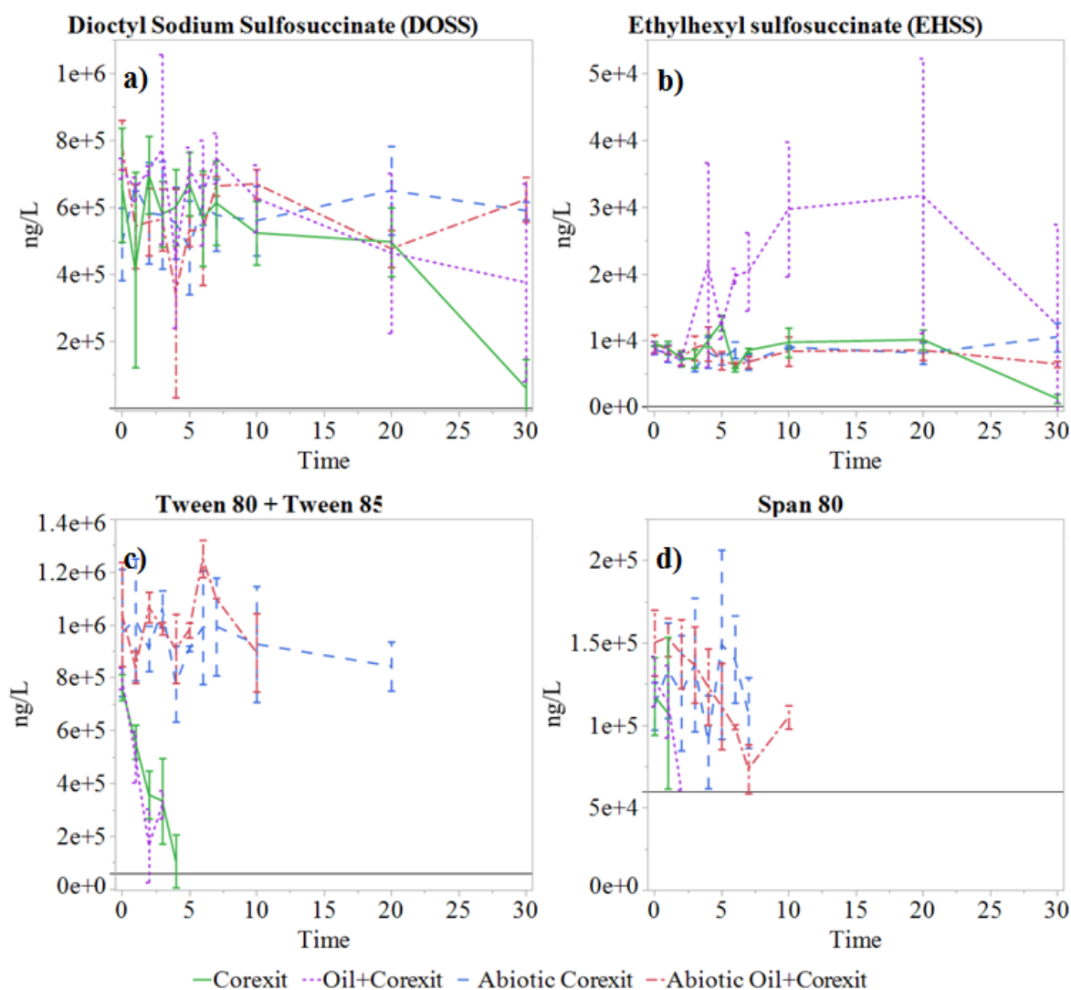
Figure 4. Corexit surfactant component loss in seawater incubations. Mean ( n=3 ) concentrations in subsampled 6-L mesocosms over time of Corexit constituents or suspected metabolites a) DOSS, b) EHSS, c) Tweens 80 and 85, and d) Span 80. The error bars denote one standard deviation from the mean, and the horizontal lines in each panel represent the limit of quantitation for that analyte (200 ng/L for DOSS and EHSS, 60,000 ng/L for the Tweens and Span 80).
