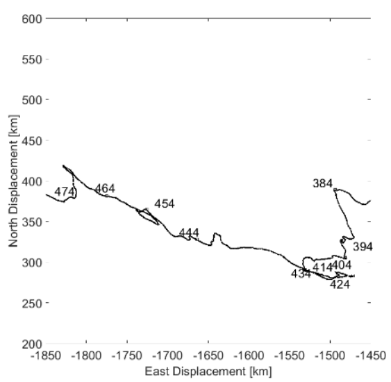
Figure 59. Progressive vector diagrams created through integration of the ice velocity time-series for M4 over the full 2017–2018 deployment
