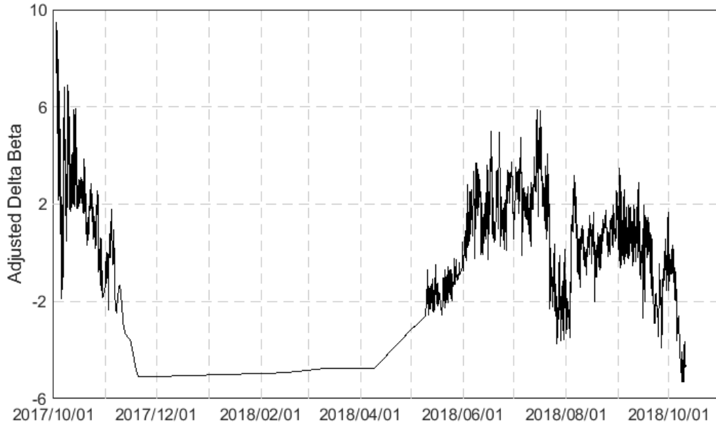
Figure 11. Adjusted delta beta curve correcting sound speed at M4 (above)
