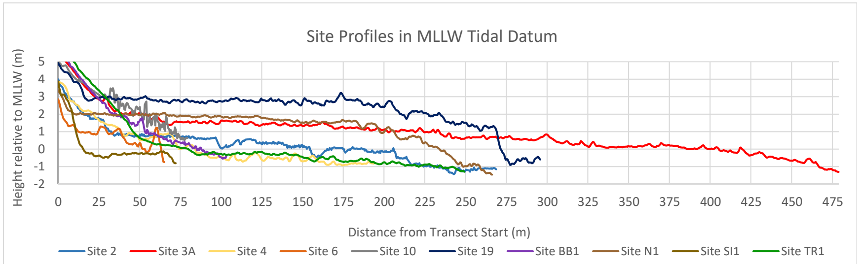
Figure 3.2.2.2. Vertical range and profile along intertidal transects at each of the 10 non-reef sites in MLLW tidal datum. Note the exaggerated vertical axis. Vertical measurements were taken to create a digital elevation model at each site and measurements often extended above the estimated Mean Higher High Water (MHHW). An unofficial tidal datum conversion factor was not available until after data analysis was conducted. This figure is provided to give additional context to each site relative to a datum used commonly by researchers in the intertidal zone.
