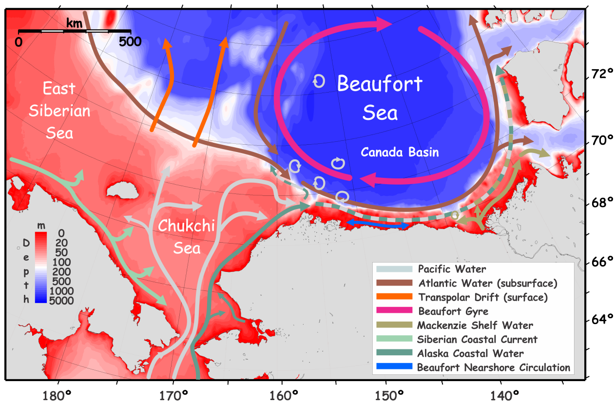
Figure 1: Idealized schematic of the circulation in the Chukchi and Beaufort seas. Nominal flow pathways are colored based on water properties, origin and/or function.
