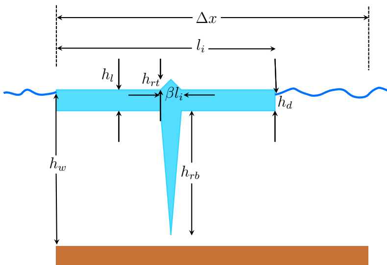
Figure 3: Cartoon of an ice floe with a deep keel. Variables are defined in table 2
