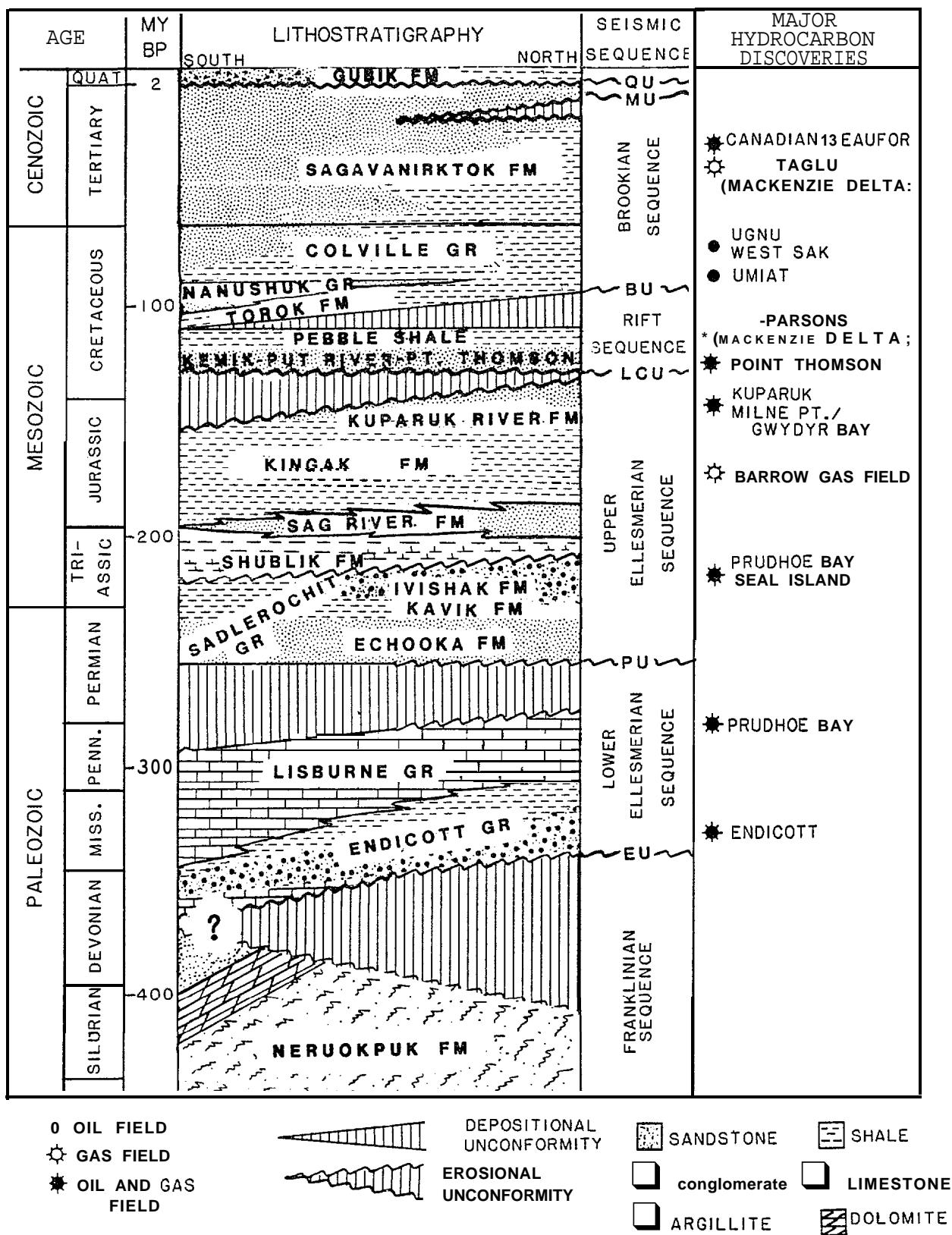
Figure 4. Generalized Lithostratigraphic Column of the Alaskan North Slope (Craig et al., 1985).
