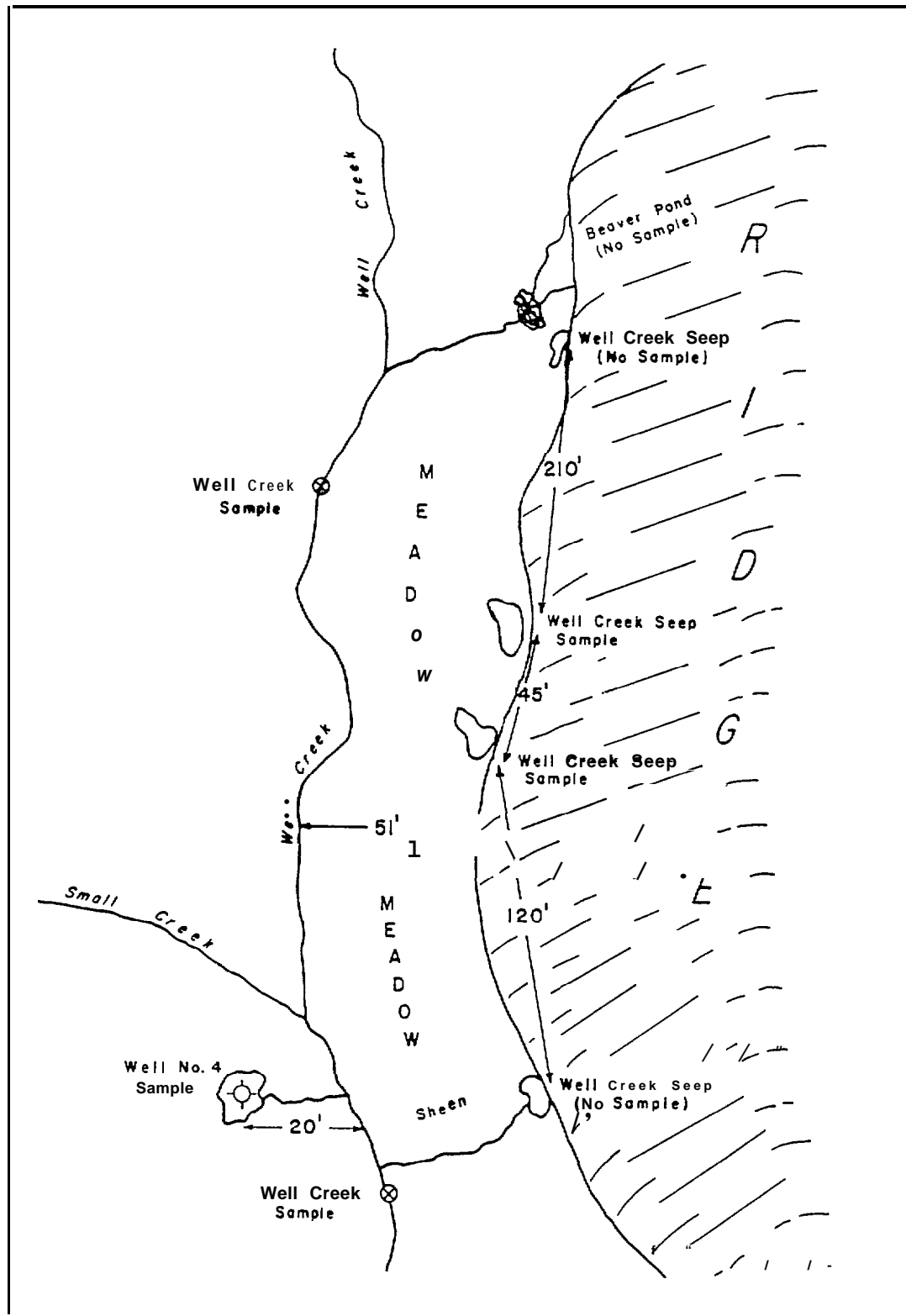
Figure 15. Oil Seeps on Well Creek, Innskin Peninsula, (From Blasko, 1976d)
