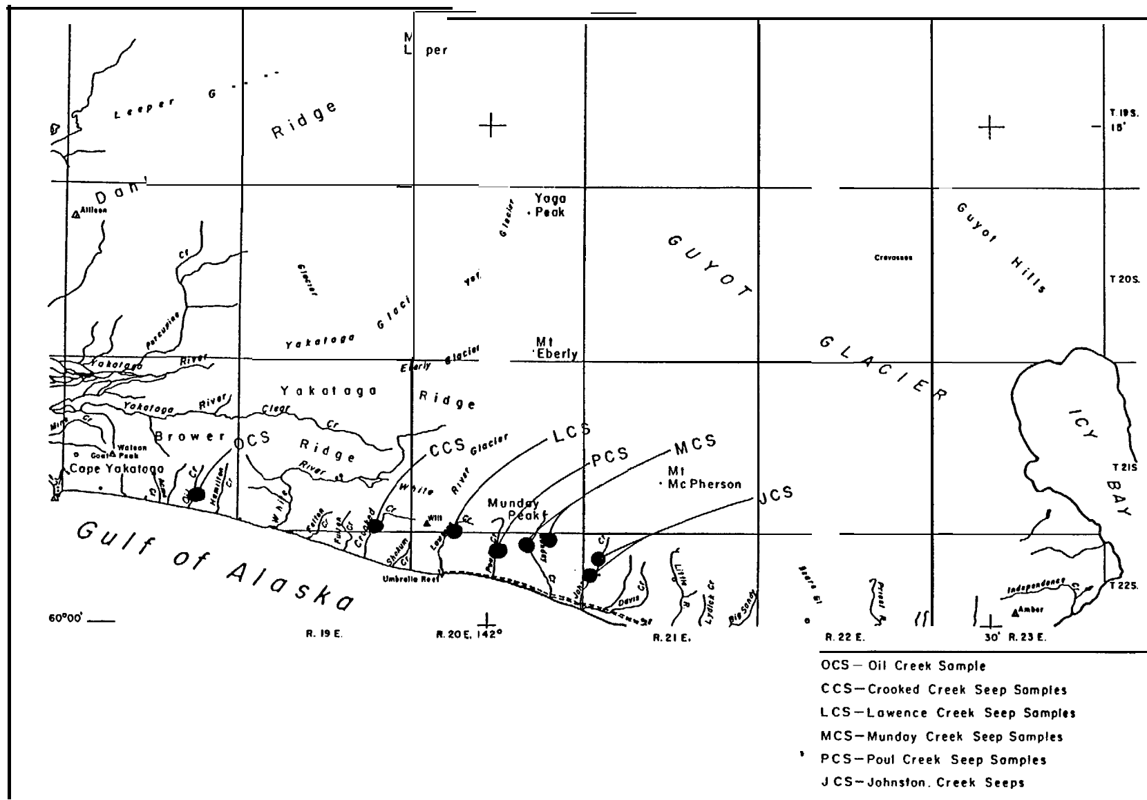
Figure 21. Stream Sampling Locations, Yakutat Oil Seepage Area. (From Blasko, 1976c)
