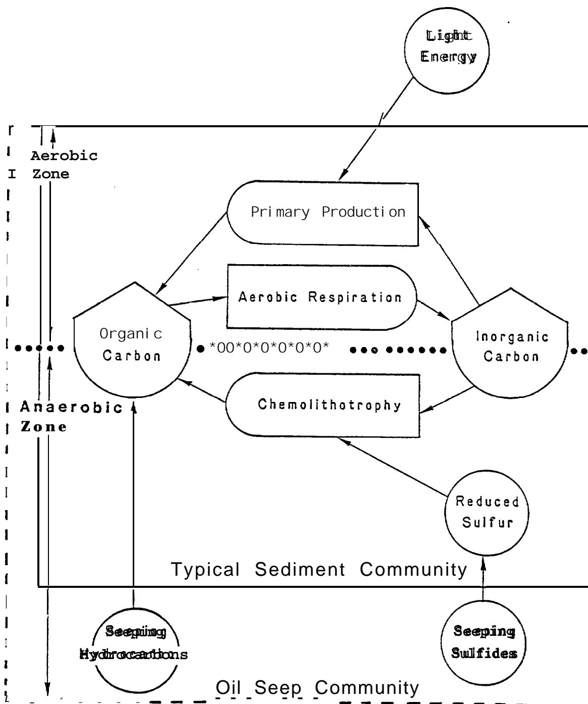
Figure 30. Model of sediment trophic-dynamics. The model demonstrates trophic enrichment by carbon and sulfide additions, via seepage, to the benthic community. The vertical zonation of oxygen and sulfide gulates decoupling of carbon and energy flow in anaerobic zone. (Montagna et al. , personal communication)
