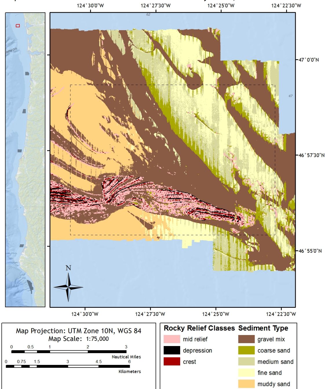
Figure 18. Seabed substrates at Grays Bank, WA
