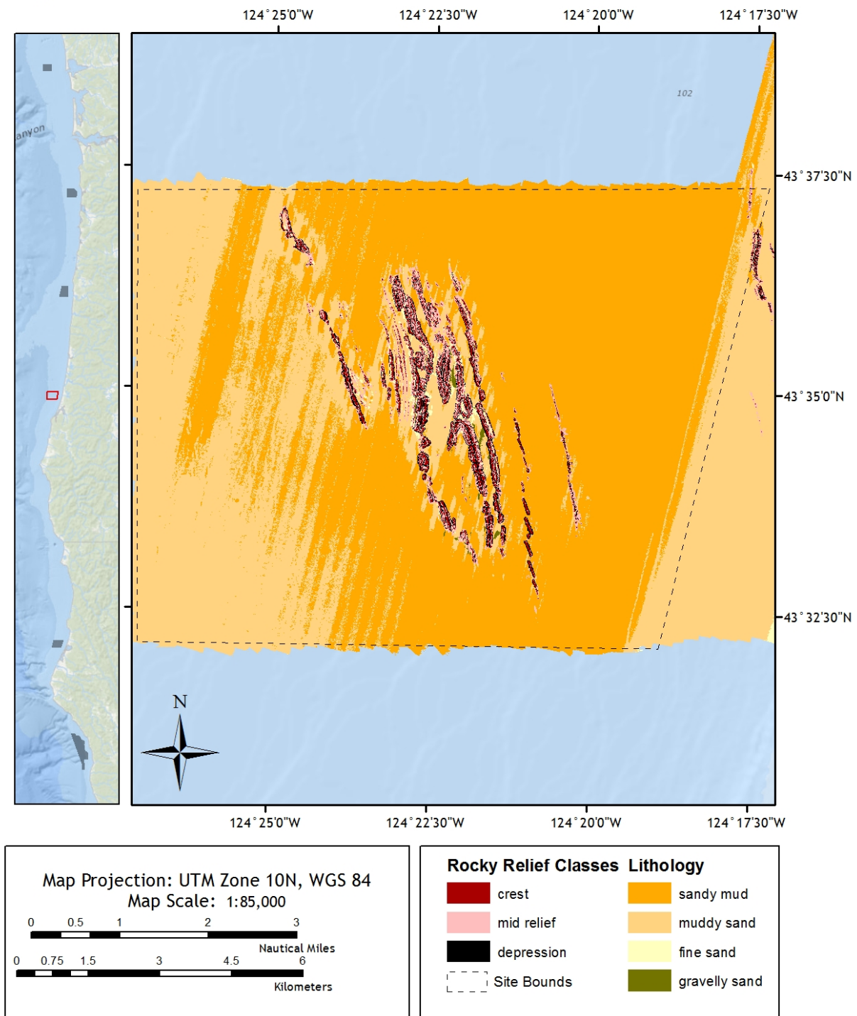
Figure 73. Seabed substrates at Siltcoos, OR
