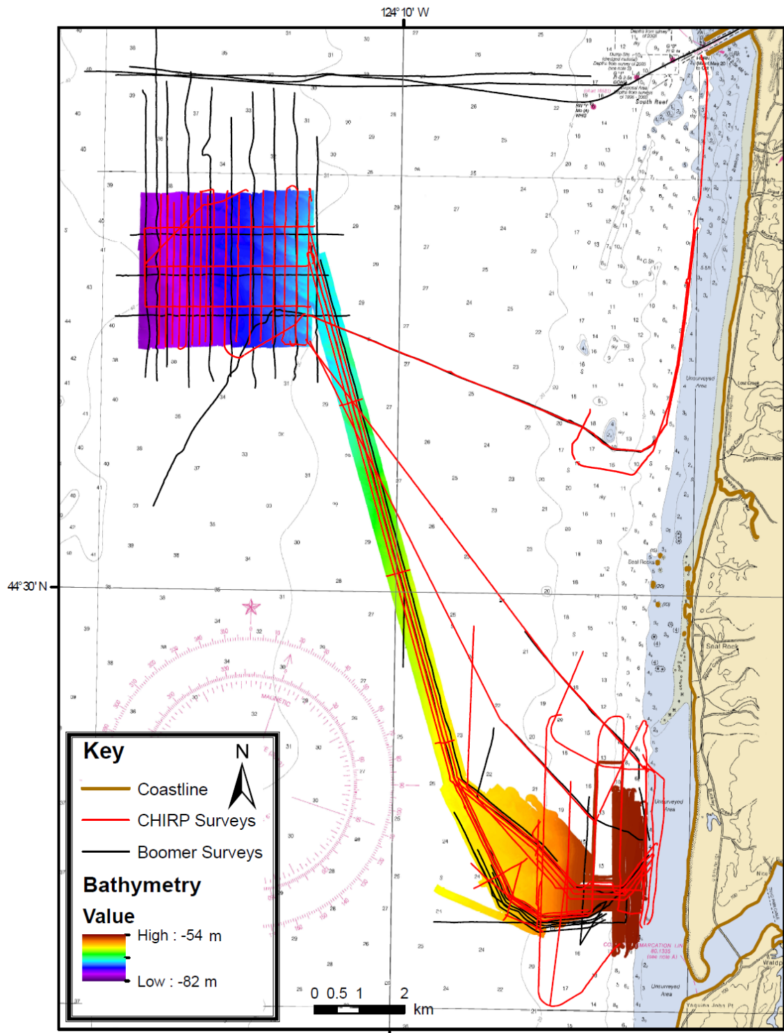
Figure 26. SETS survey area bathymetric data and geophysical tracklines near Seal Rock, OR
