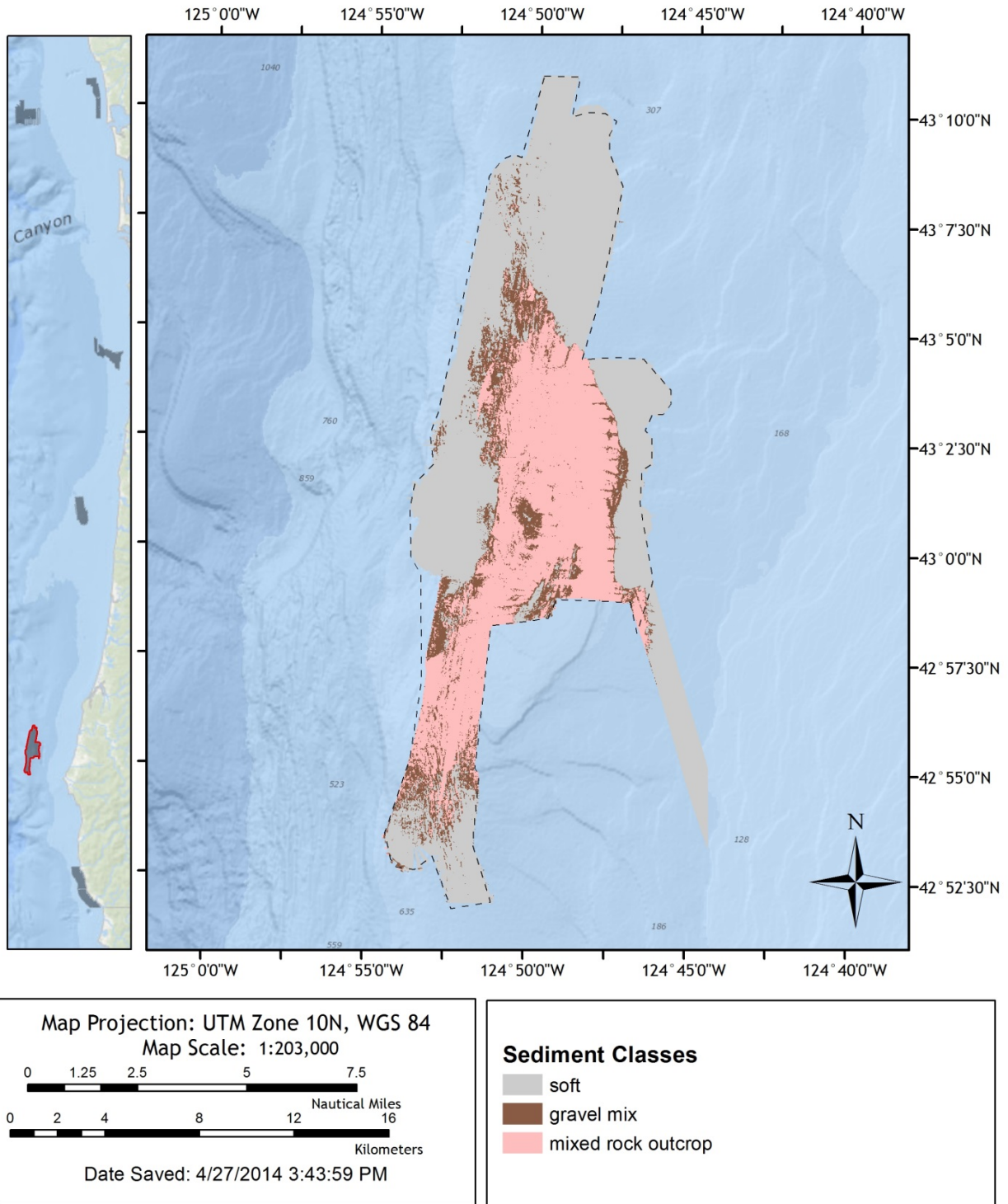
Figure 85. Seabed substrates at Coquille Bank, OR
