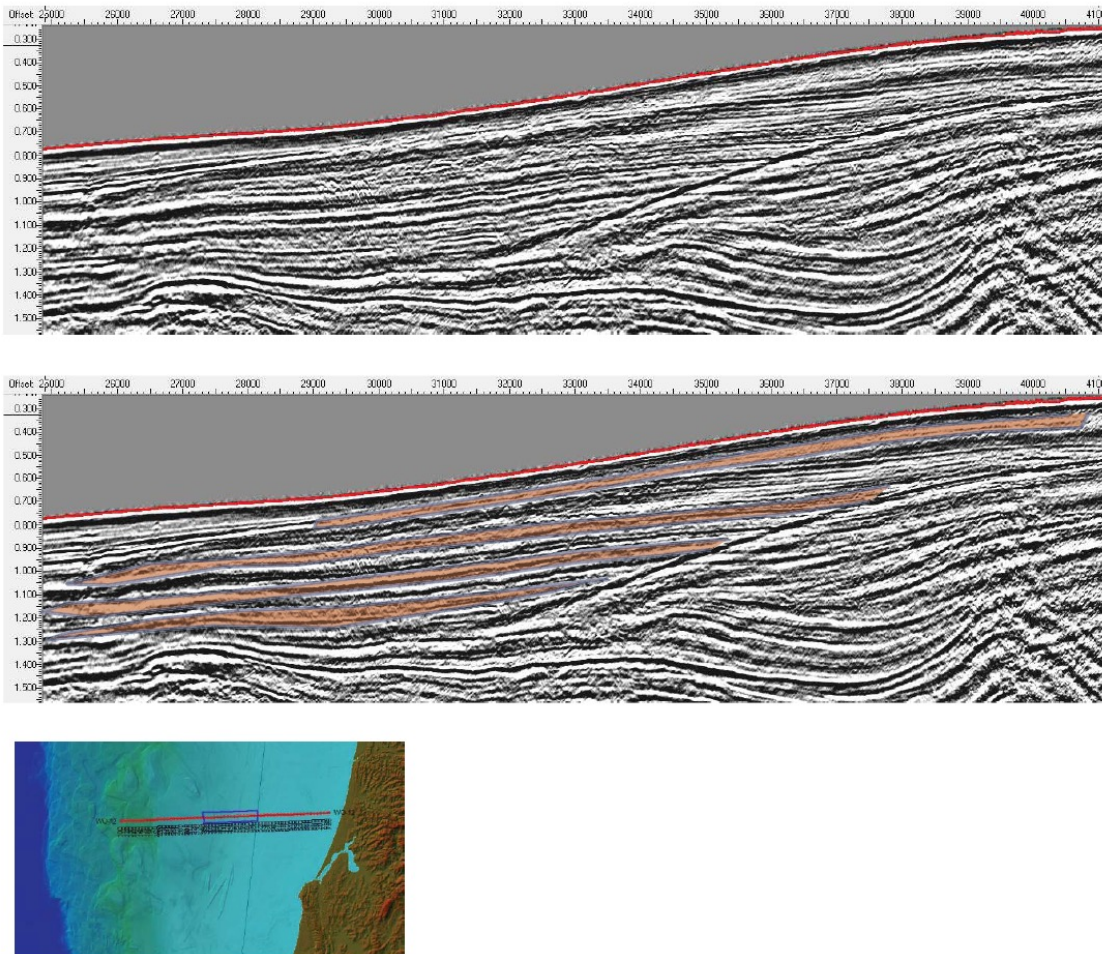
Figure 56. Multichannel profile WO-12, Coos Basin, OR
