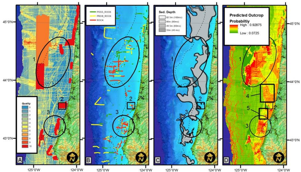
Figure 54. Map products predict seabed character
