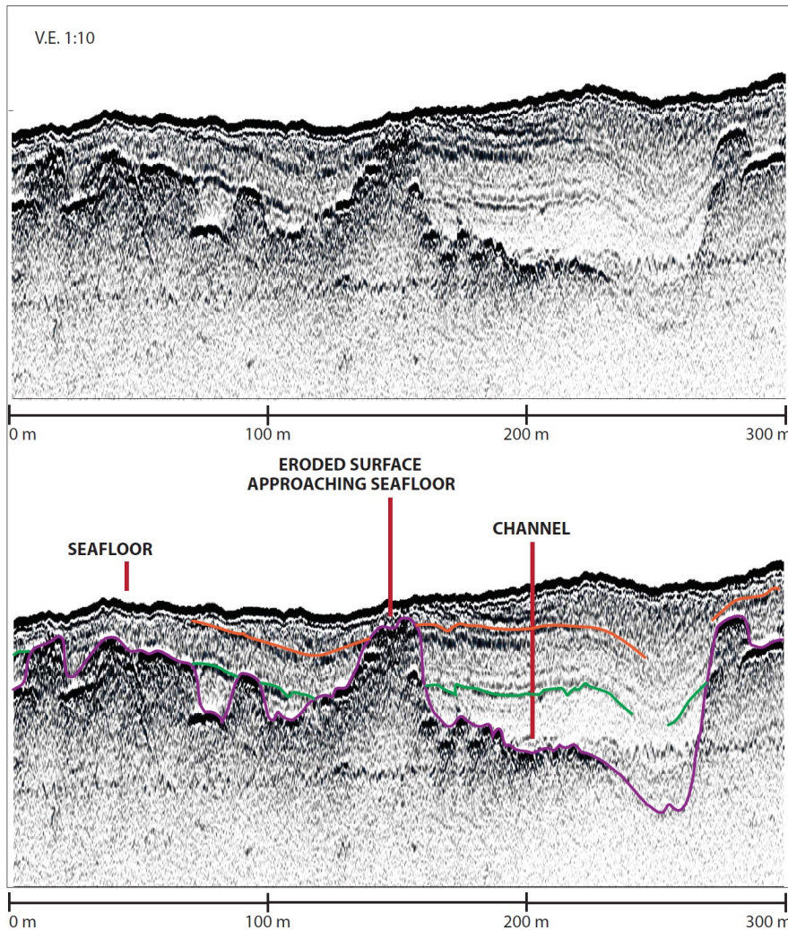
Figure 33. Chirp profile, SETS test berth site
