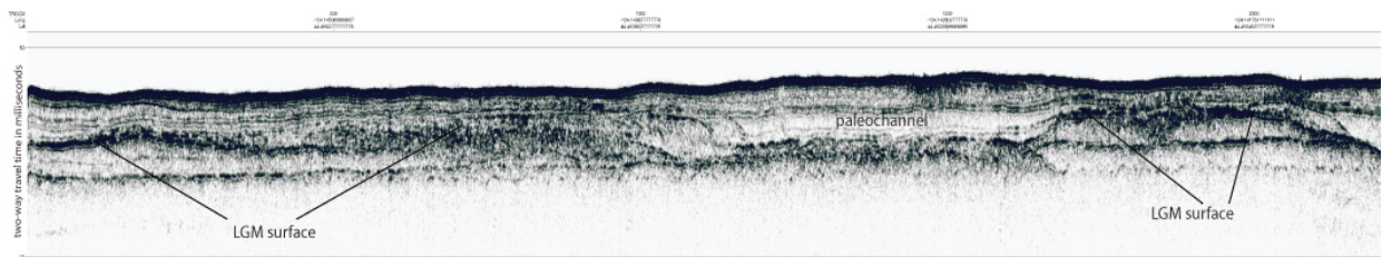
Figure 4. Chirp subbottom profile in the vicinity of Newport, Oregon
