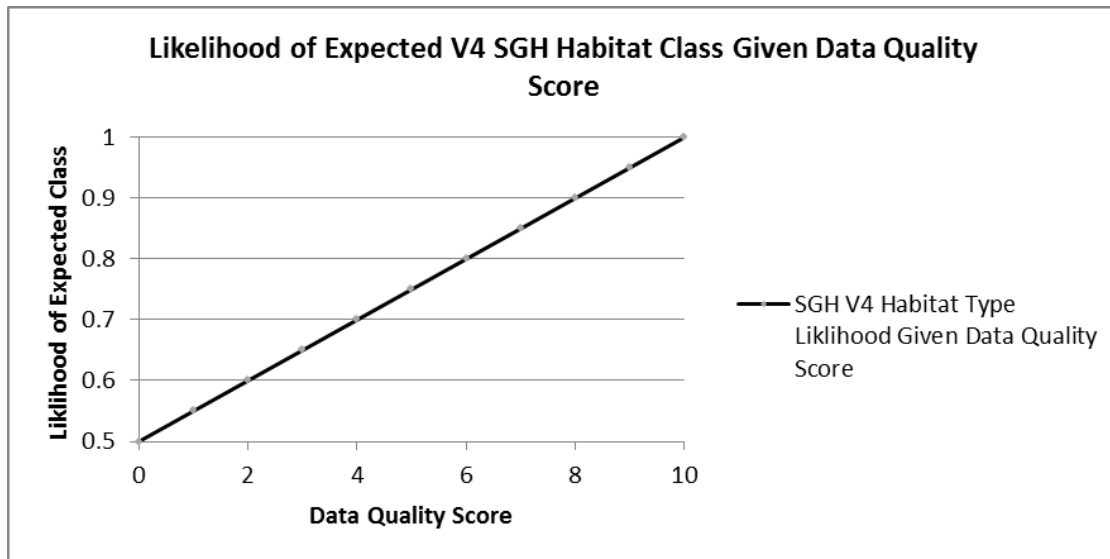
Figure 13. The relationship between Data Quality Score and the likelihood of observing the expected SGH habitat class. A linear relationship between data quality score and likelihood of habitat type is expertly defined and applied to the model at the ProbOfOutcropSGH node.
