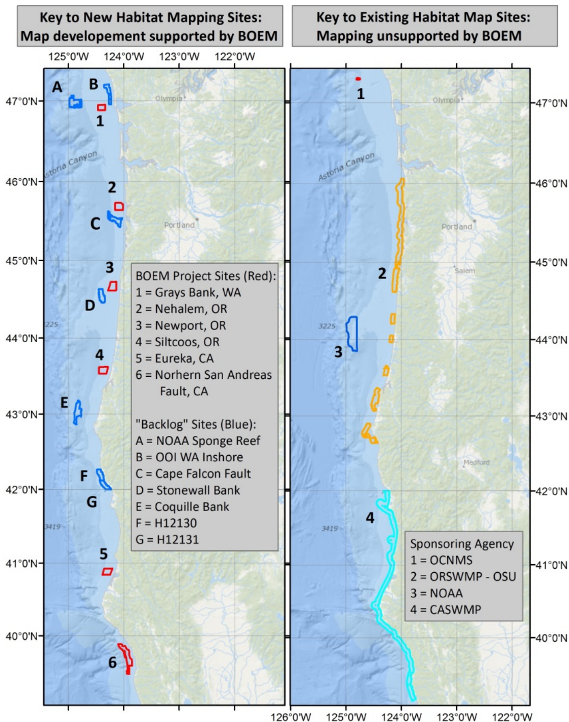
Figure 10. New and existing data for habitat maps Overview of local sites both newly mapped (new data acquisition) and existing, used to update the SGH Map Version 4.0. The left panel shows locations where BOEM supported the development of habitat maps; either interpretation of “backlog” data (blue color) or both the data acquisition and interpretation (red color) of habitat maps. The right panel shows existing maps developed external to the BOEM project.
