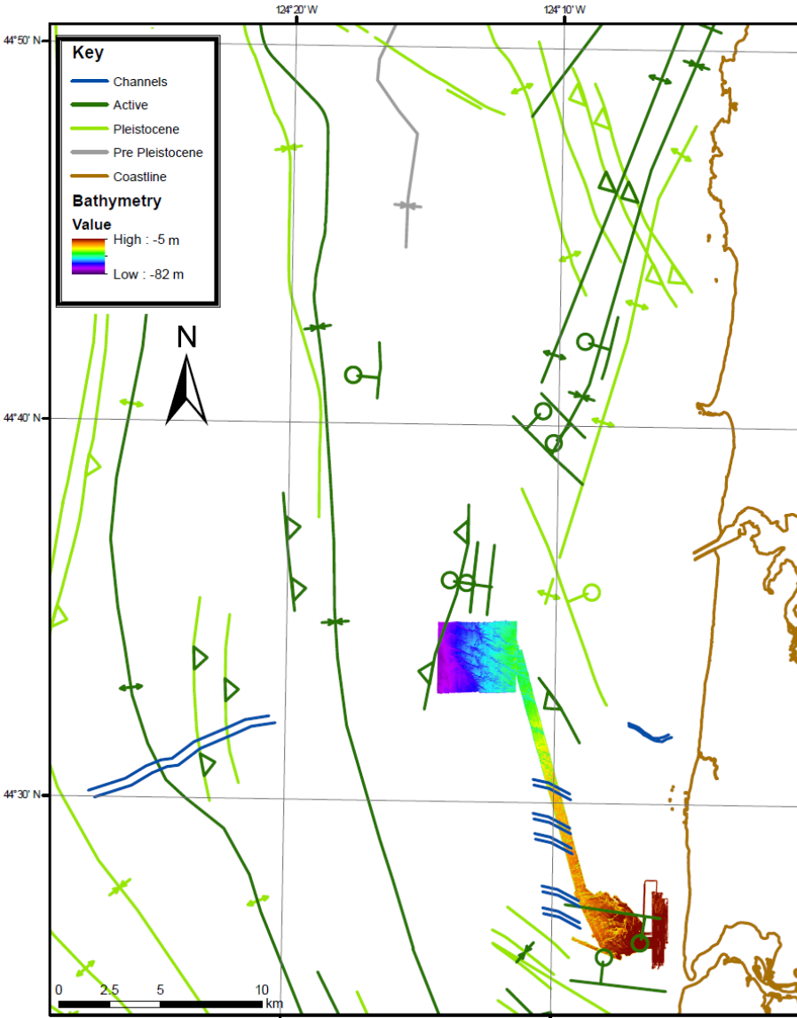
Figure 27. Major structures of the inner shelf off Newport, OR
