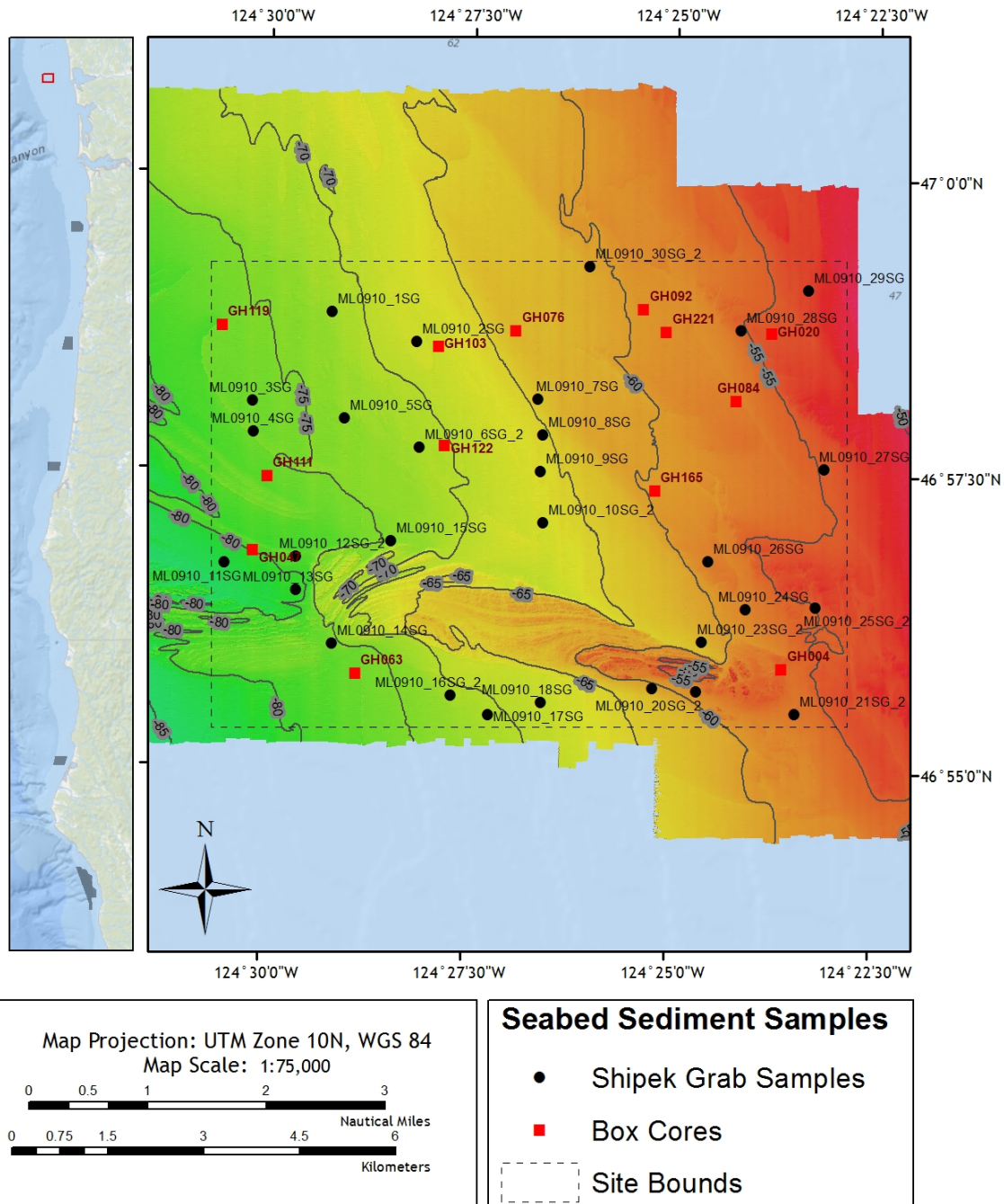
Figure 16. Color shaded-relief multibeam bathymetry data collected at Grays Bank, WA Sediment sample stations plotted over the Reson 8101 (240 kHz) multibeam.
