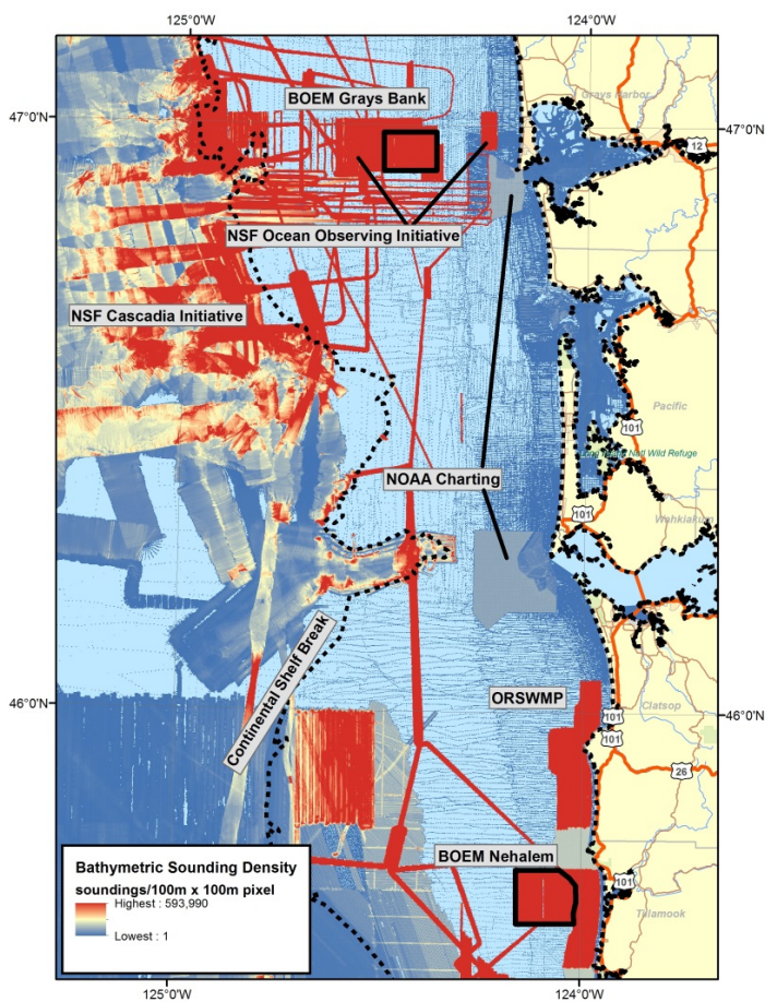
Figure 15. Bathymetric data density Map showing the density of bathymetric soundings on the continental shelf and slope of the Oregon-Washington border. Note that over shelf environments new data contributions have come from varied sources.
