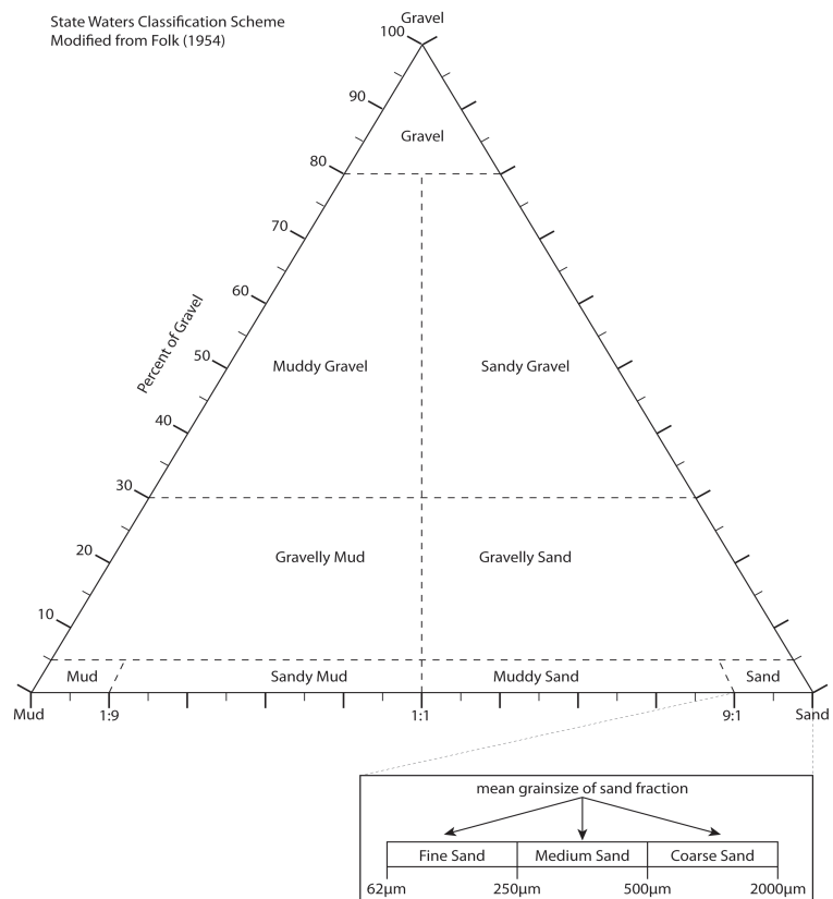
Figure 9. Ternary diagram showing basis for the textural classification of sediments collected under this project The textural classification illustrated here was also the basis for the sedimentary habitat types of local-scale mapping products.
