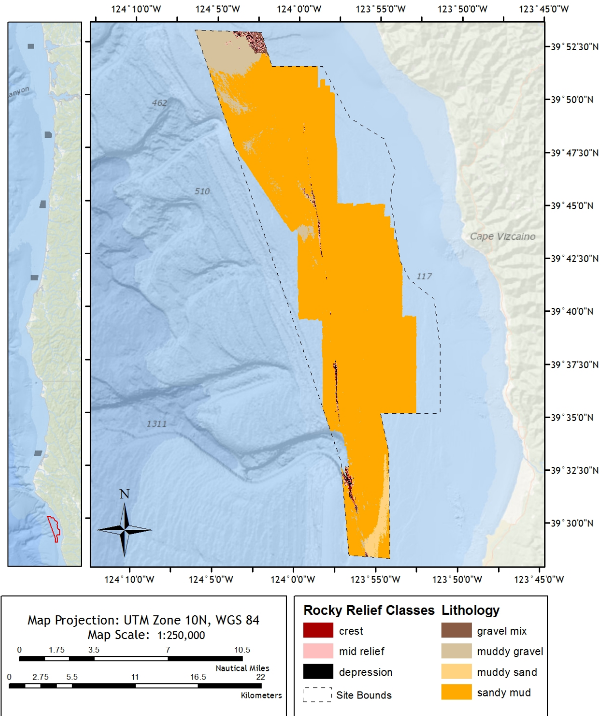
Figure 80. Seabed substrates at Northern San Andreas Fault (NSAF), CA
