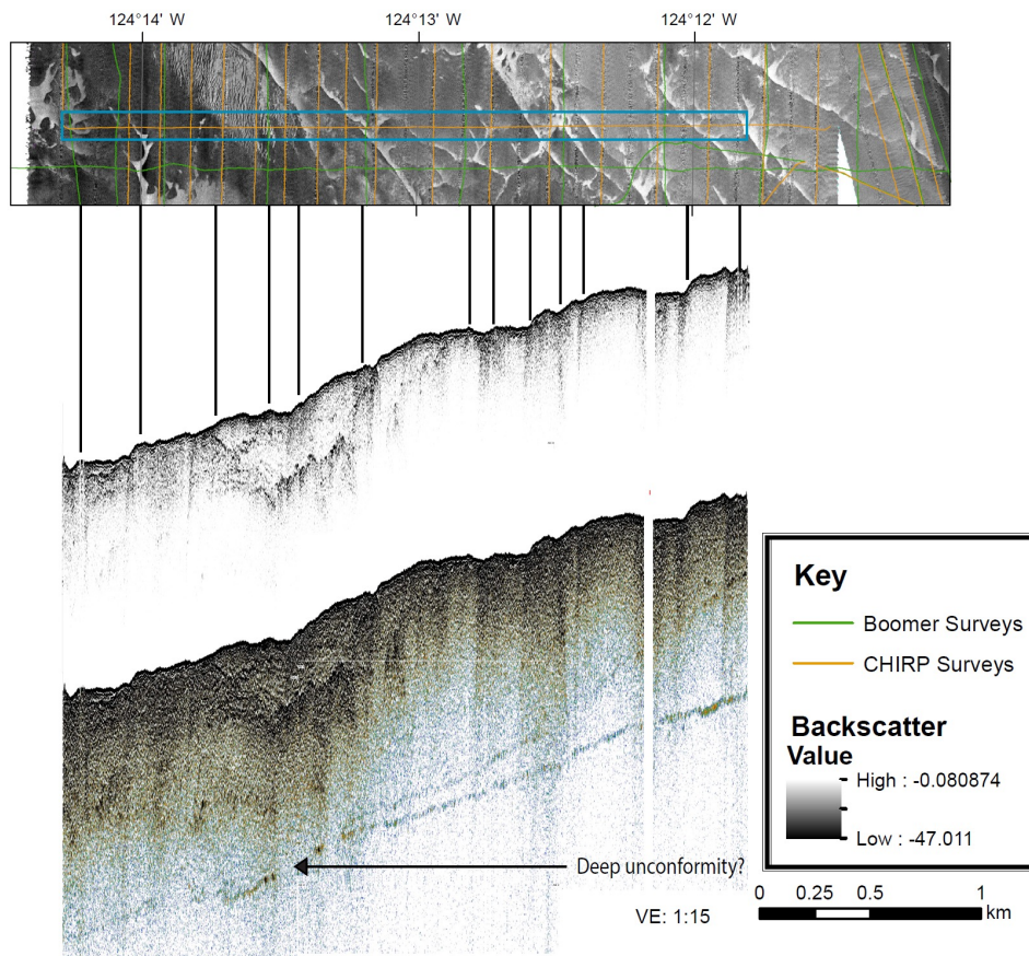
Figure 30. CHIRP profile and corresponding backscatter across possible paleodunes, SETS test berth
