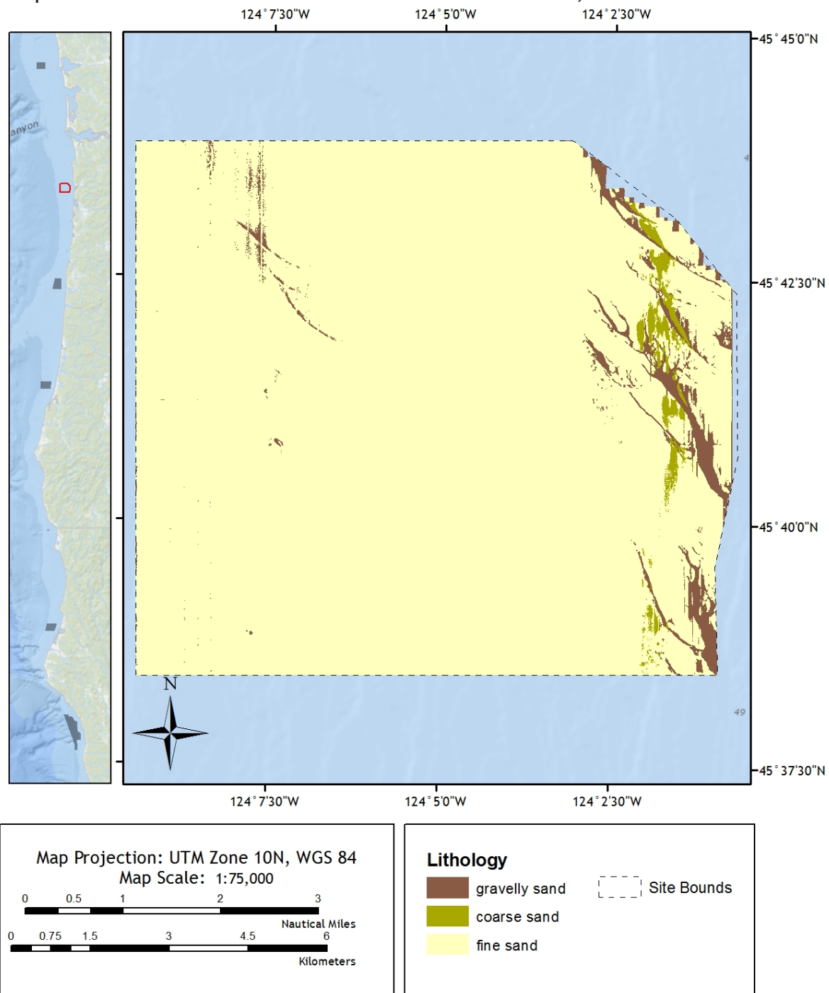
Figure 22. Seabed substrates at Nehalem, OR
