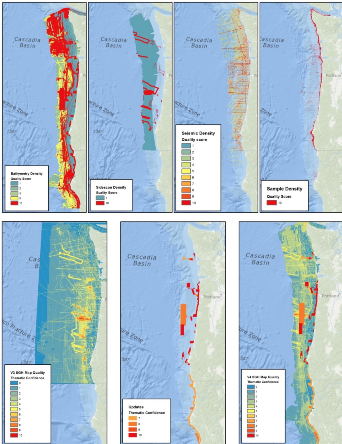
Figure 45. Version 4.0 Data Quality map series
