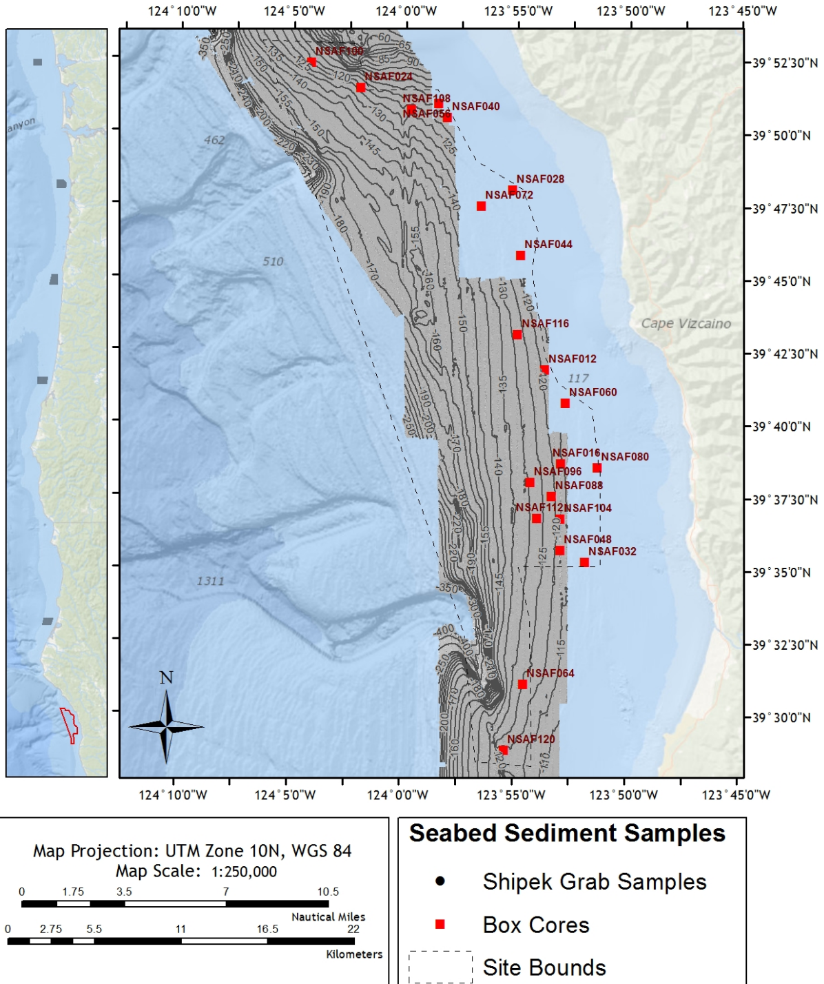
Figure 77. Multibeam bathymetry data collected at Northern San Andreas Fault (NSAF), CA Sediment sample stations plotted over the Reson 8101 (240 kHz) multibeam data.
