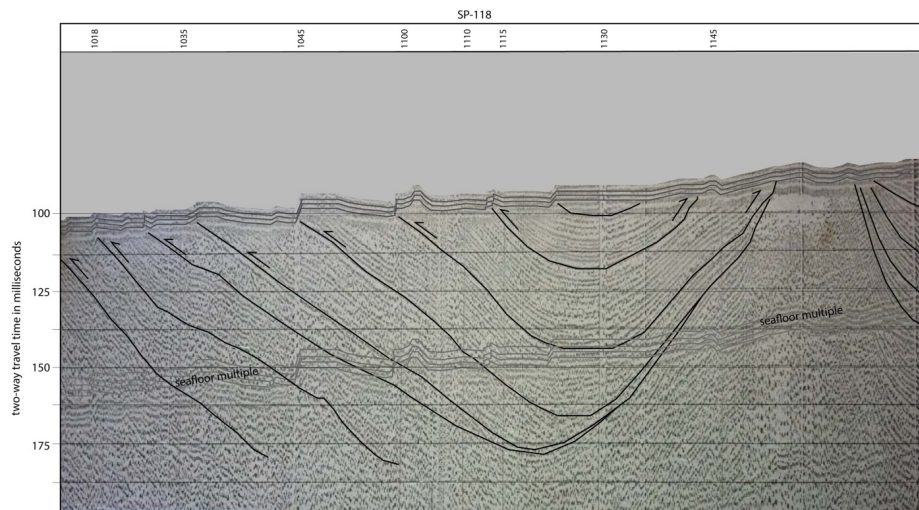
Figure 3. An example of typical flexural slip faulting style ubiquitous on the mid to inner shelf in the study area
