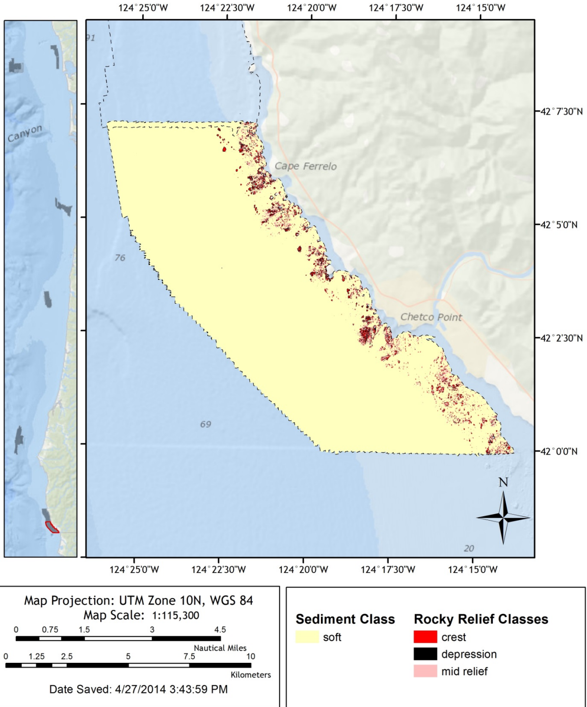
Figure 87. Seabed substrates at H12131 Survey Sheet, OR Sediment classes are not predicted due to lack of seabed samples. Rocky relief classes are predicted by analysis of bathymetric data.
