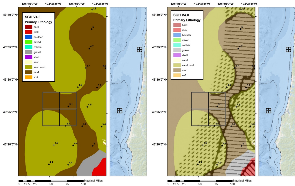
Figure 55. SGH Map Version 4.0 in the vicinity of the Wind Float site, southern Oregon Wind float site shown by subdivided square. Original interpretation of the “mud line” (Kulm et al., 1975) overlaid (hatch pattern) in right panel.
