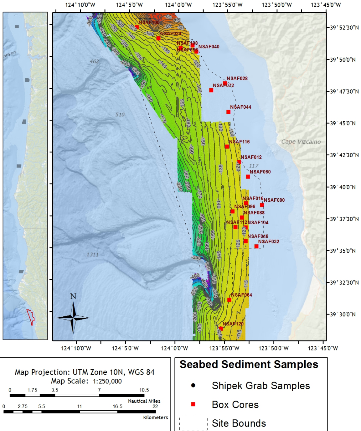
Figure 41. Color shaded-relief multibeam bathymetry data collected at Northern San Andreas Fault (NSAF), CA
