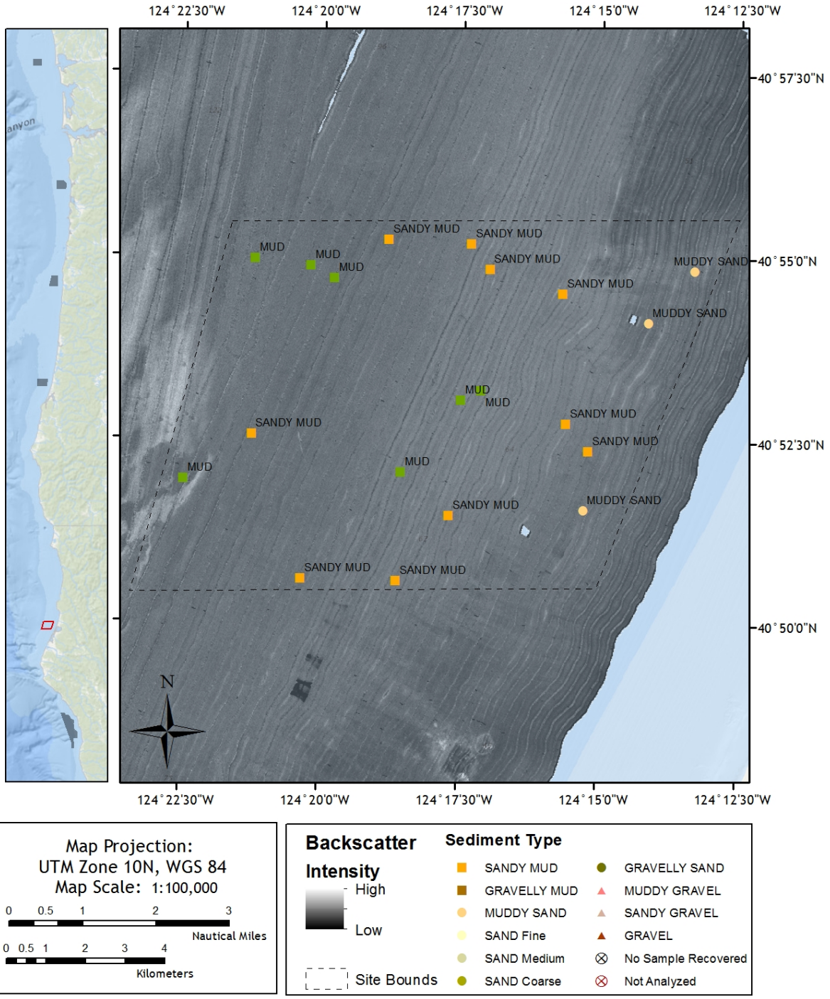
Figure 39. Multibeam backscatter data collected at Eureka, CA Sediment textural classifications plotted over the Kongsberg EM3000 (300 kHz) multibeam backscatter data.
