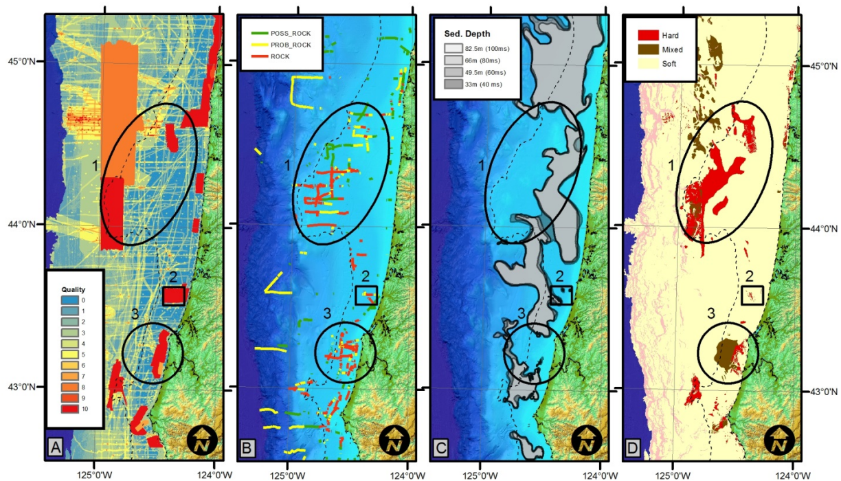
Figure 53. Map products reveal seabed character (hard or soft seabed)
