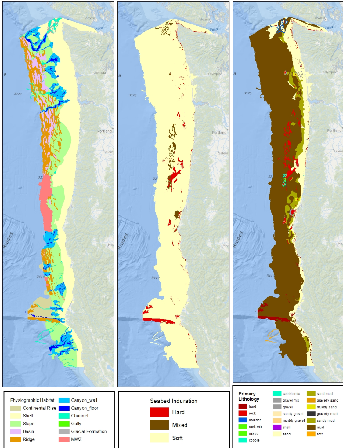
Figure 44. Version 4.0 Surficial Geologic Habitat maps for WA, OR, and northern California Each map panel is derived from the same underlying polygon feature class, but is symbolized according to a different map attribute with Physiographic Habitat (left), Seabed Induration (center), and Primary Lithology (right). MWZ = Mass wasting zone.
