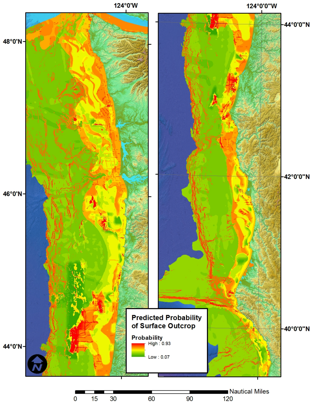
Figure 50. Maps showing modeled probability of rock outcrop of the continental shelf and slope from the Canadian border into central Oregon (left panel) and central Oregon to northern California (right panel)
