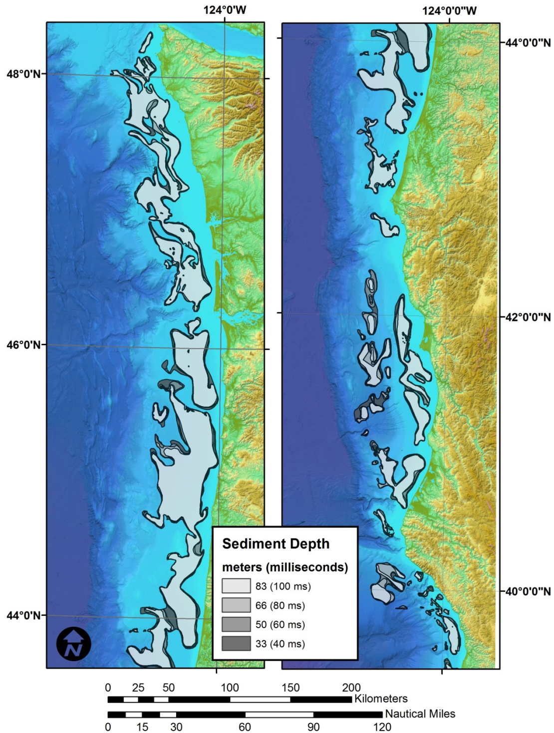
Figure 49. Isocore map showing vertical units of minimum sediment thickness in meters (and two-way travel time in milliseconds)
