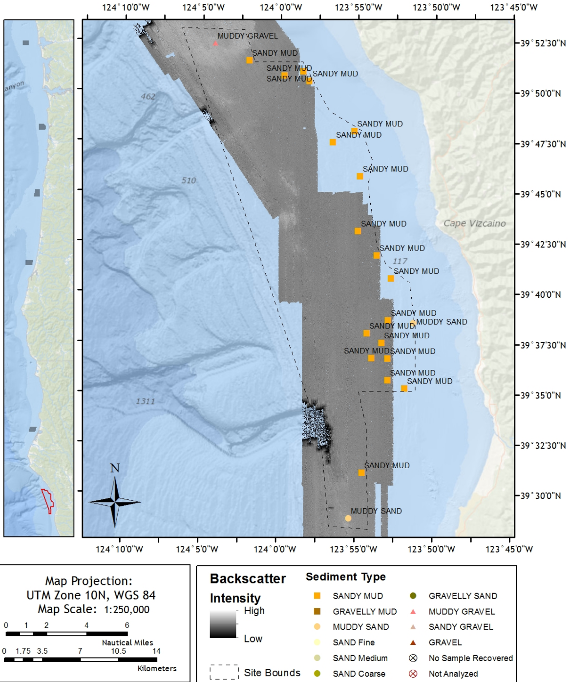
Figure 42. Multibeam backscatter data collected at Northern San Andreas Fault (NSAF), CA Sediment textural classifications are plotted over the Reson 8101 (240 kHz) multibeam data.
