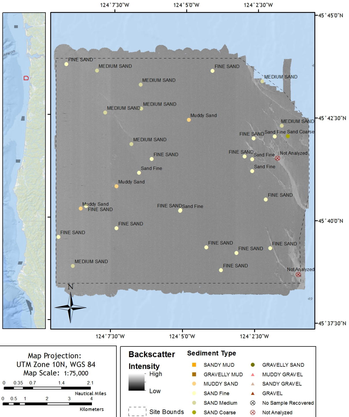
Figure 64. Multibeam backscatter data collected at Nehalem, OR Sediment textural classifications are plotted over the Reson 8101 (240 kHz) multibeam backscatter data.
