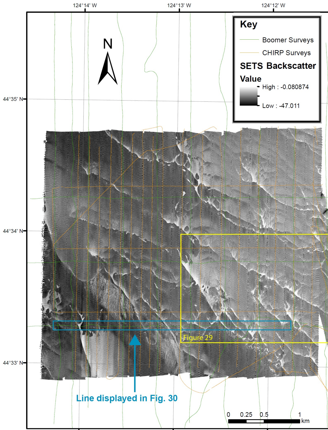
Figure 28. Backscatter data in the SETS test berth site overlain with boomer and CHIRP sub bottom profile tracklines
