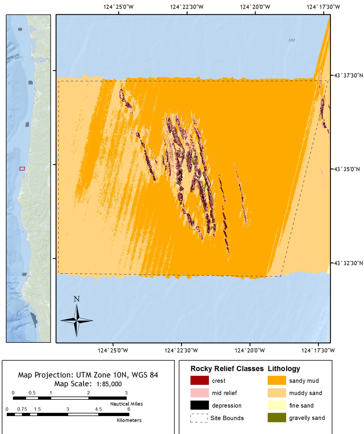
Figure 37. Seabed substrates at Siltcoos, OR
