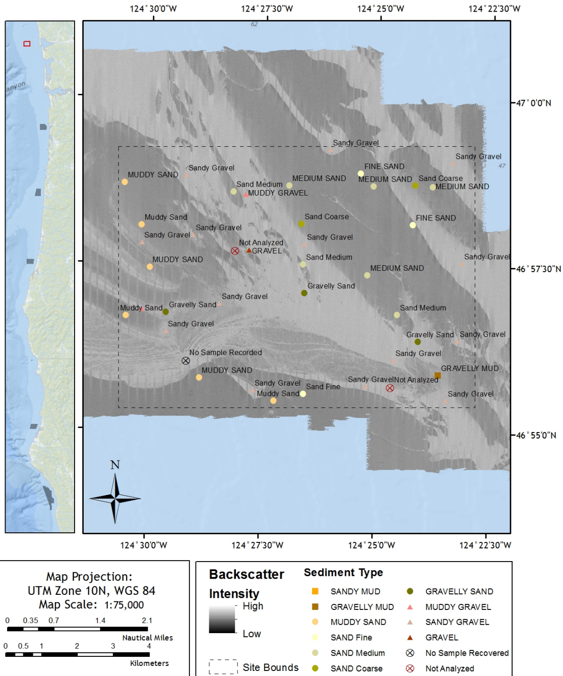
Figure 17. Multibeam backscatter data collected at Grays Bank, WA Sediment textural classifications are plotted over the Reson 8101 (240 kHz) backscatter data.
