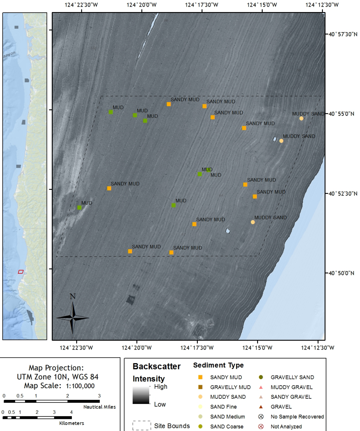
Figure 75. Multibeam backscatter data at Eureka, CA Sediment textural classifications plotted over the Kongsberg EM3000 (300 kHz) multibeam backscatter data.
