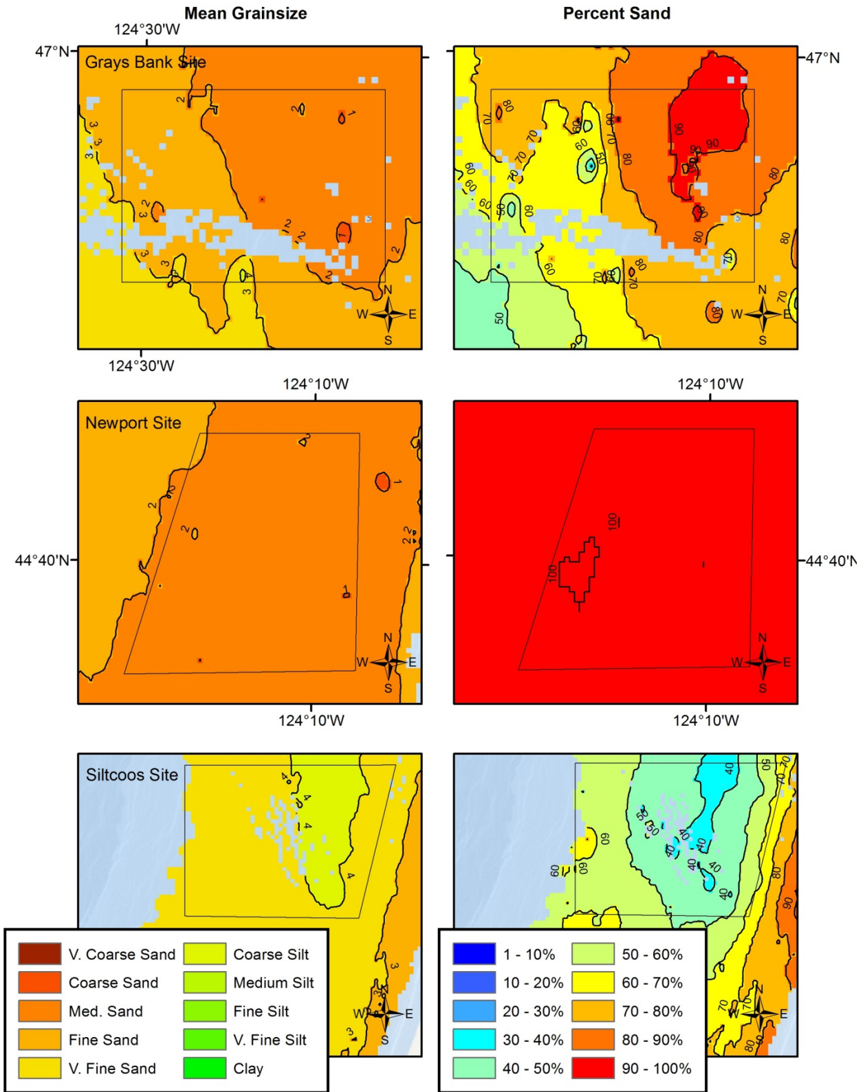
Figure 52. Grainsize and percent sand at local mapping sites Grays Bank, WA, and Newport & Siltcoos, OR.
