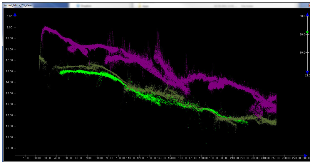
Figure 6. Vertical offset in repeat surveys at Redfish Rocks, Oregon
