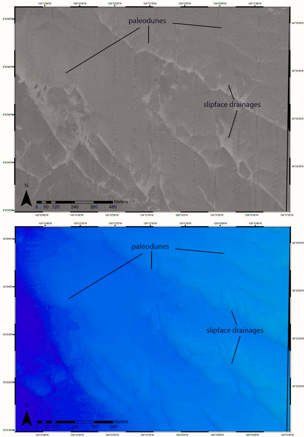
Figure 29. Backscatter (top) and shaded relief imagery of a part of the SETS test berth site NW trending asymmetric bathymetric features are shown in the seabed imagery. Steeper faces toward the SW. Scour depressions (high backscatter) form drainages, mostly on the steeper faces. Features are tentatively interpreted as subaerially formed paleo dunes.
