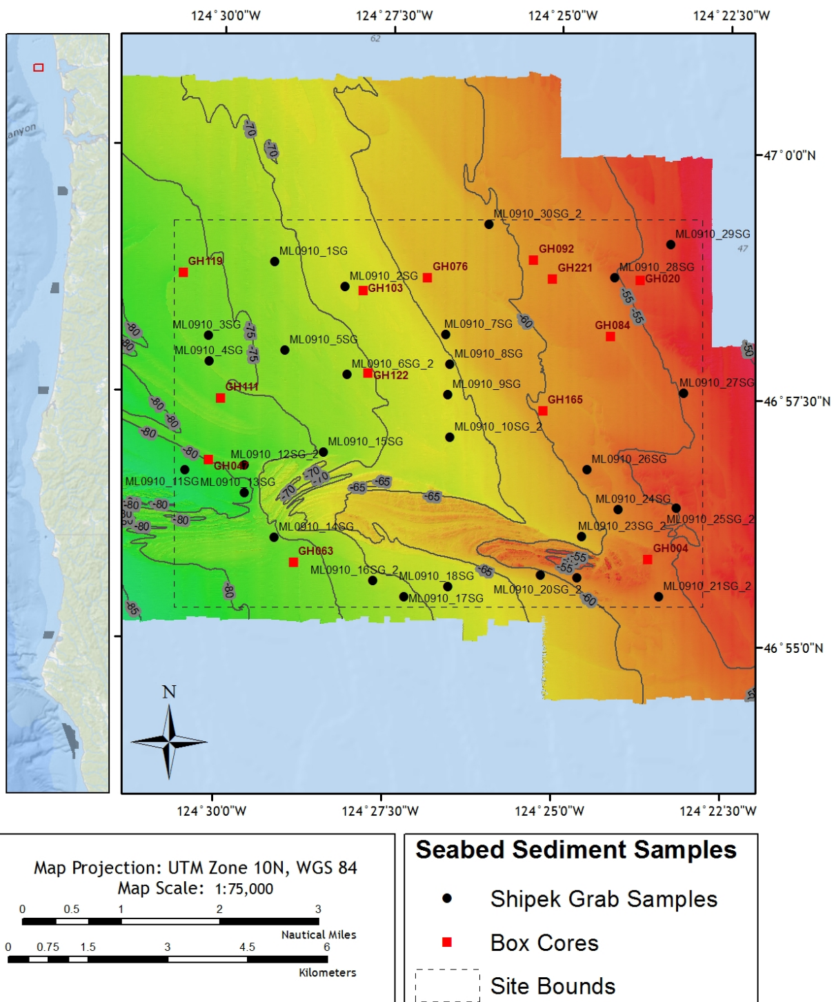
Figure 59. Color shaded-relief multibeam bathymetry data collected at Grays Bank, WA Sediment sample are plotted over the Reson 8101 (240 kHz) multibeam bathymetry data.
