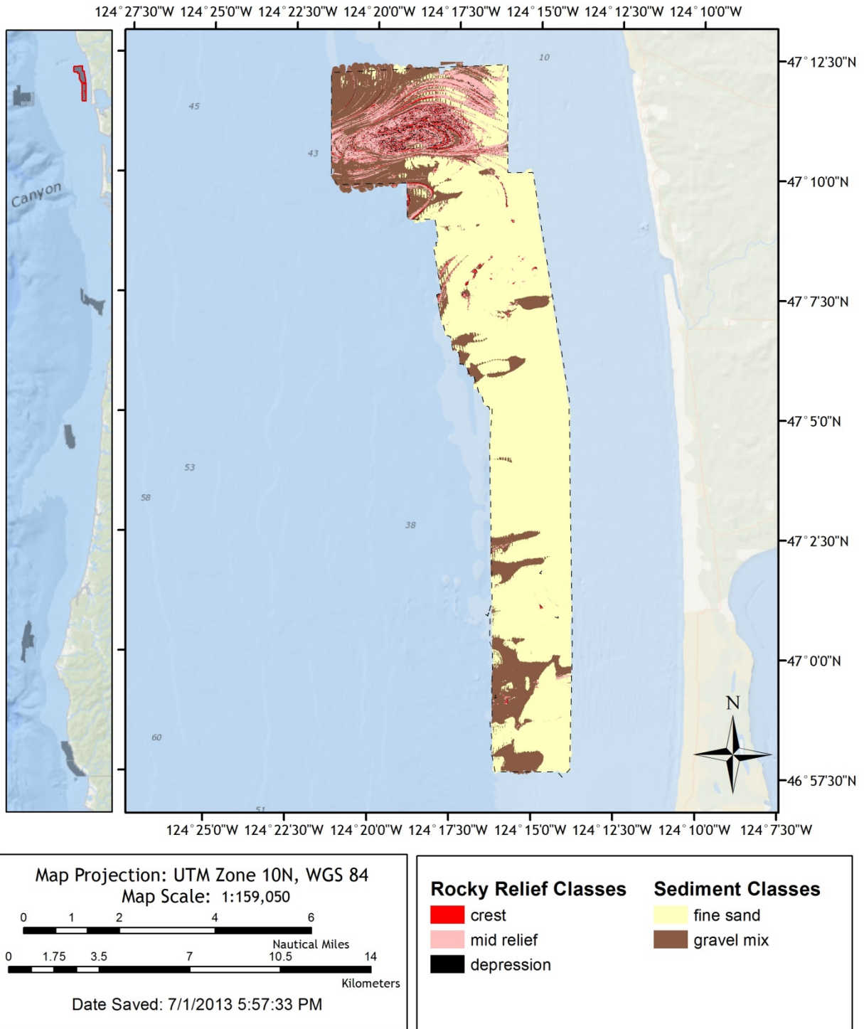
Figure 81. Seabed substrates at OOI Inshore Site, WA
