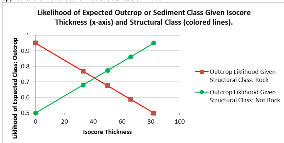
Figure 14. The relationship between Isocore Thickness, Structural Outcrop Class, and the likelihood of observing an outcrop or sediment class A linear relationship between data quality score and likelihood of habitat type is expertly defined and applied to the model at the ProbOfOutcropSGH node.
