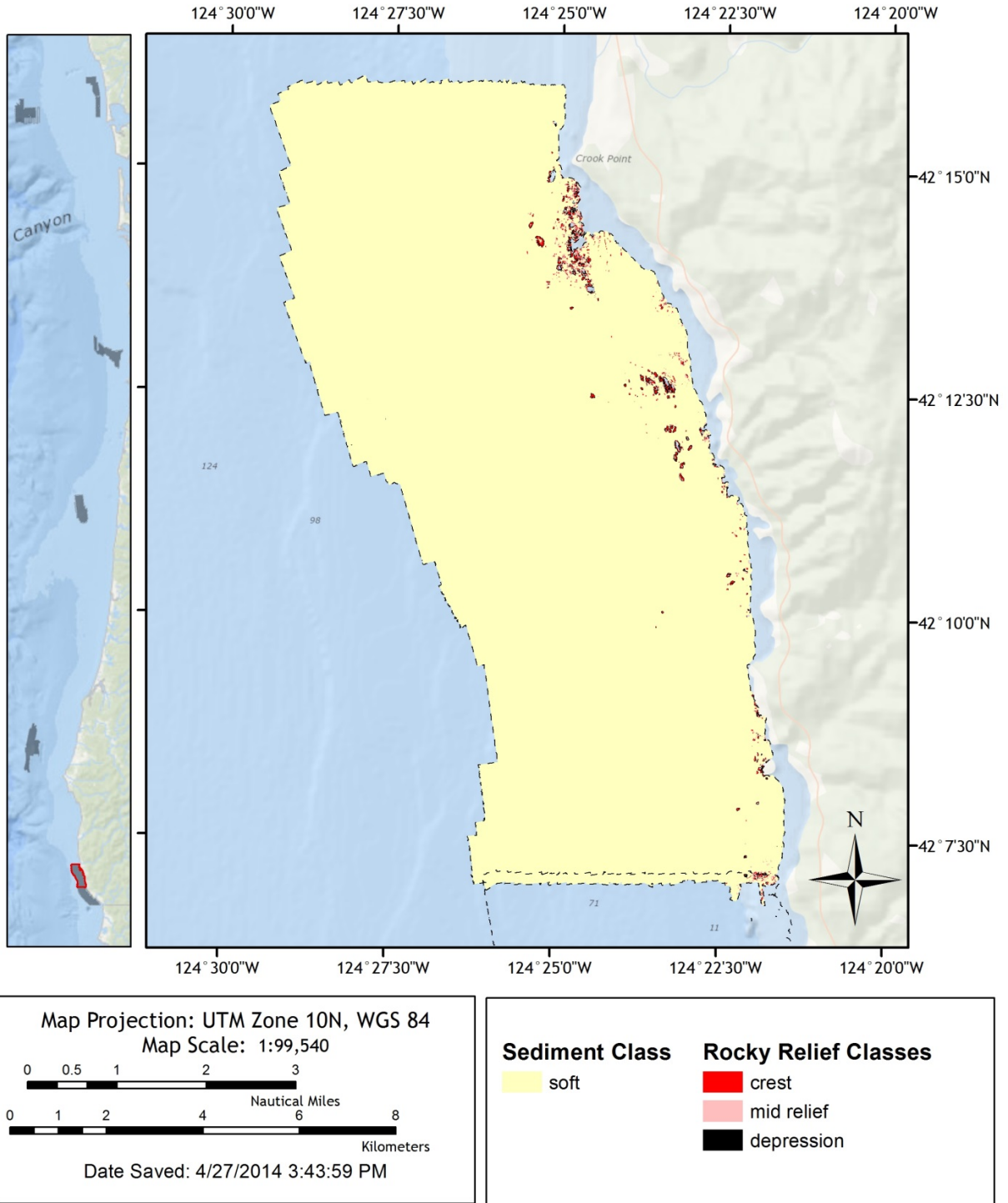
Figure 86. Seabed substrates at H12130 Survey Sheet, OR Sediment classes are not predicted due to lack of seabed samples. Rocky relief classes are predicted by analysis of bathymetric data.
