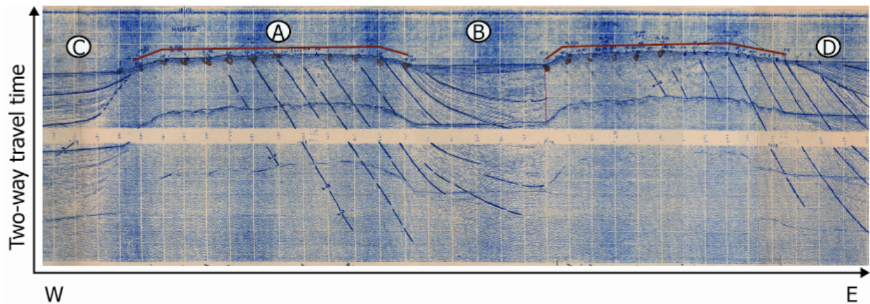
Figure 11. An industry two-dimensional seismic reflection profile over Nehalem Bank Areas in red (A) correspond to areas of predicted rock outcrop. Sedimentary stratigraphy is evident in the region between outcrops (B) and in the extreme eastern (D) and western (C) margins of the bank.
