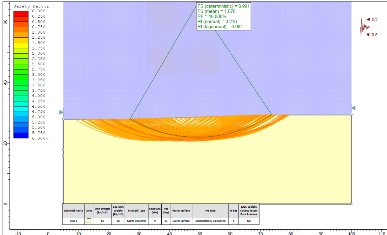
Figure 57. Slope stability model for a 2 degree slope Physical property values from nearby cores are shown in the data block.
