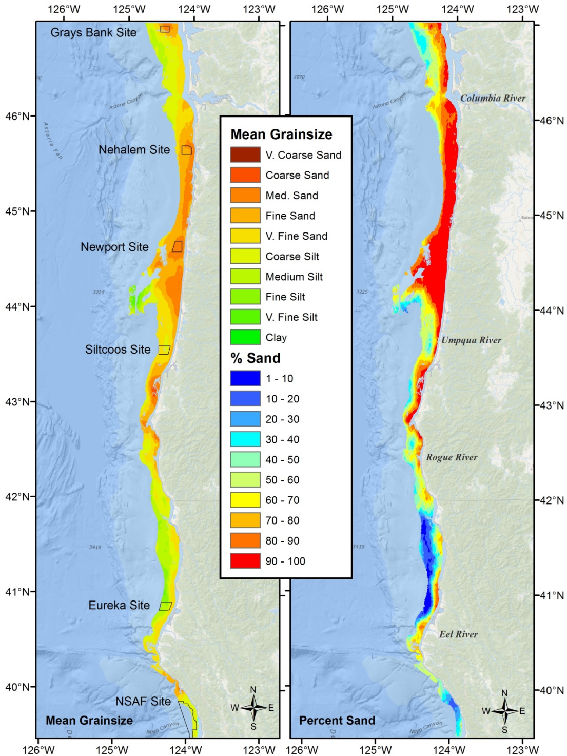
Figure 51. Mean grain size (left panel) and percent sand composition (right panel) models of the continental shelf margin out to 130 m depth and inshore to 20 m water depth
