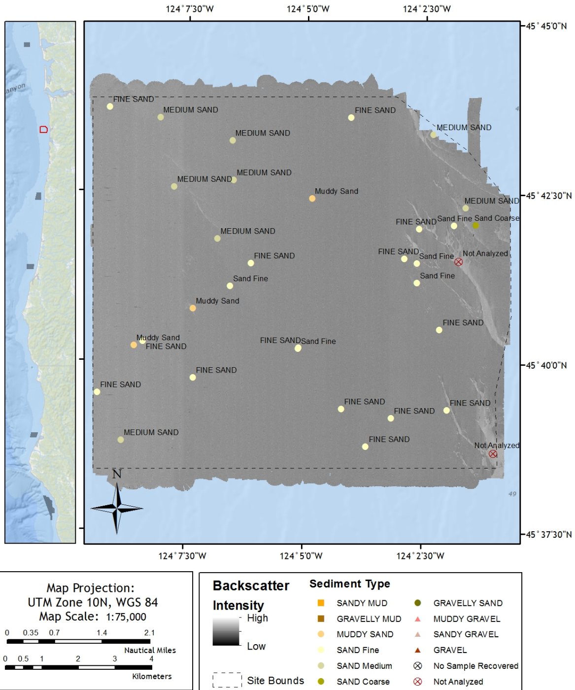
Figure 21. Multibeam backscatter data collected at Nehalem, OR Sediment textural classifications are plotted over the Reson 8101 (240 kHz) multibeam backscatter data.
