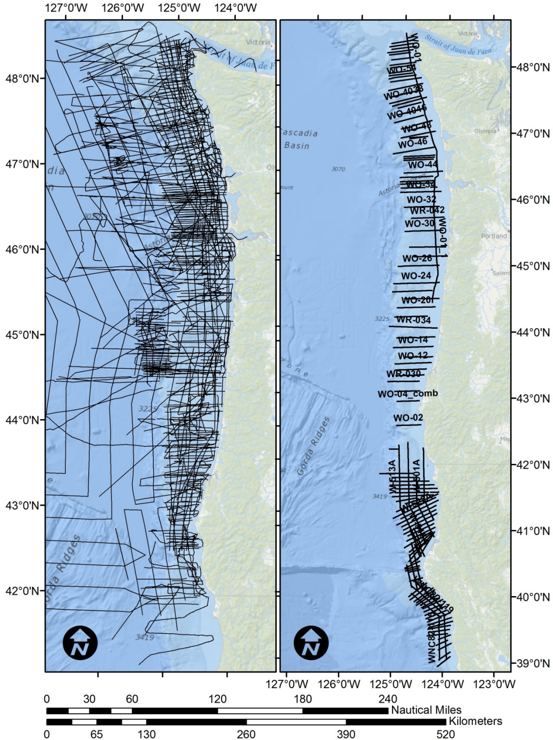
Figure 47. Seismic reflection trackline maps
