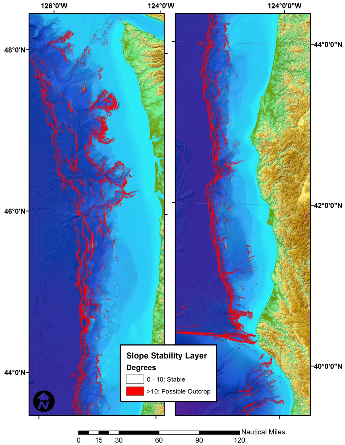
Figure 46. Slope stability derived predictive rock outcrop map for deep-water (continental slope and canyons)
