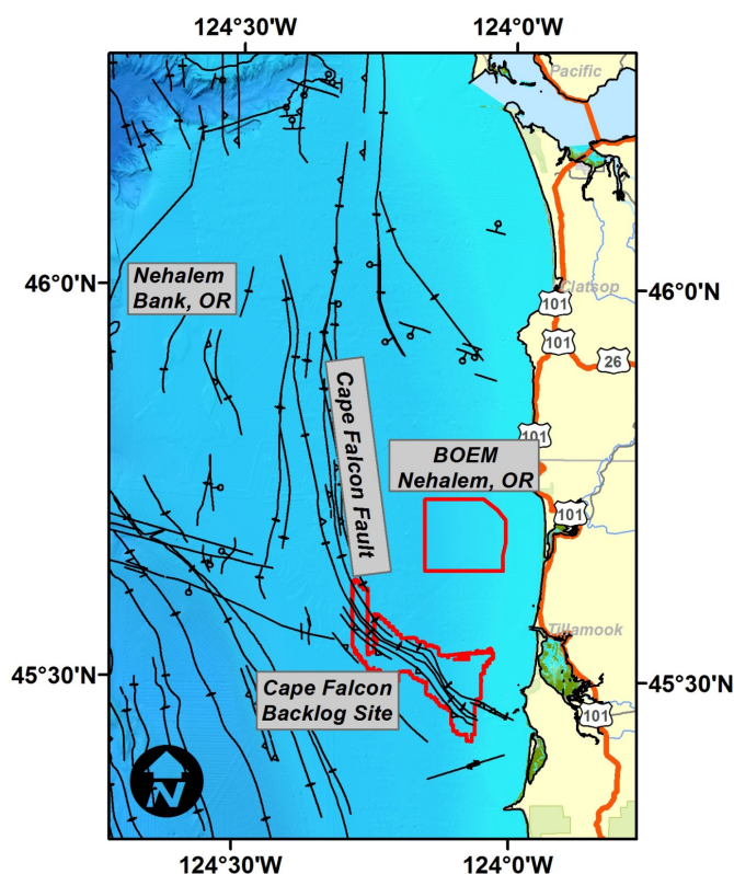
Figure 19. Oregon continental shelf in the vicinity of the Nehalem, OR BOEM study site
