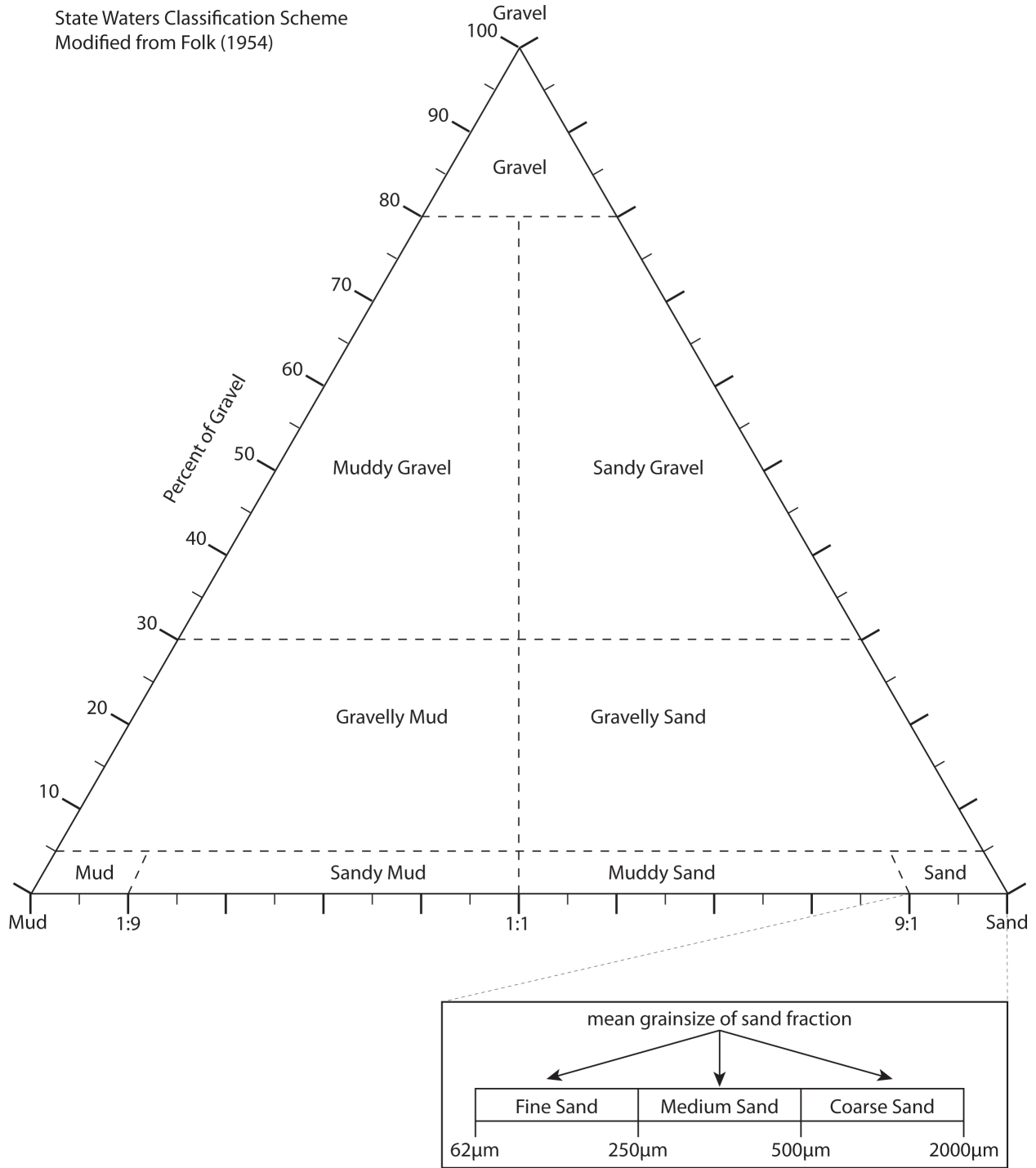
Ternary diagram showing basis for the textural classification of sediments used for the BOEM, “Backlog”, and ORSWMP local sites. Modified after Folk (1954)
