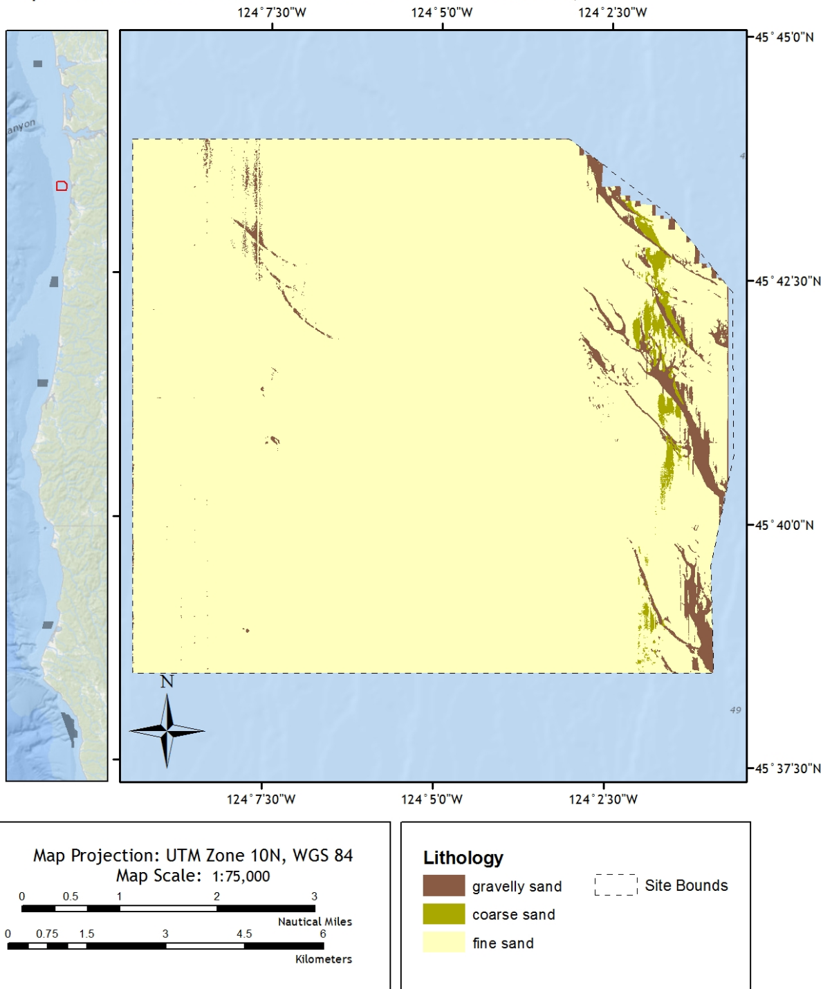
Figure 65. Seabed substrates at Nehalem, OR
