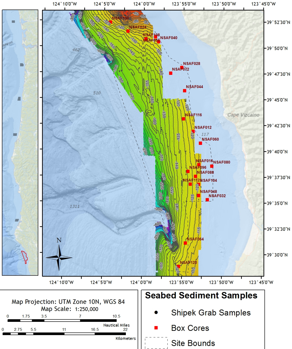
Figure 78. Color shaded-relief multibeam bathymetry data collected at Northern San Andreas Fault (NSAF), CA
