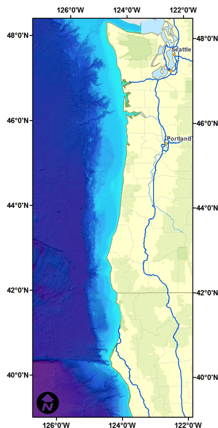
Figure 1. Project study area The study area included the continental margin of southern Washington, Oregon, and northern California.
