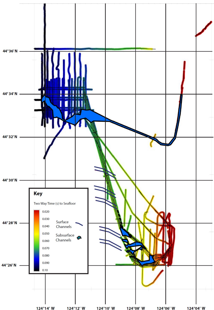
Figure 34. Two-way travel time to shallowest unconformity surface, SETS test site
