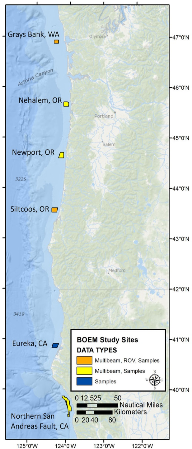
Figure 7. Distribution of BOEM study sites Colors indicate the type of data collected at each for the Survey of Benthic Communities near Potential Renewable Energy Sites Offshore the Pacific Northwest.
