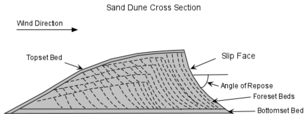
Figure 31. Typical subaerial dune cross section. http://www.tulane.edu/~sanelson/images/dune.gif
