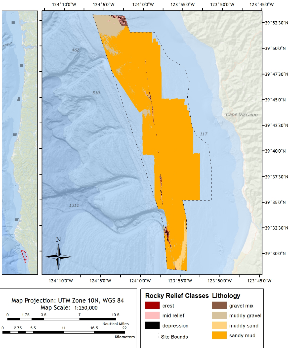
Figure 43. Seabed substrates at Northern San Andreas Fault (NSAF), CA
