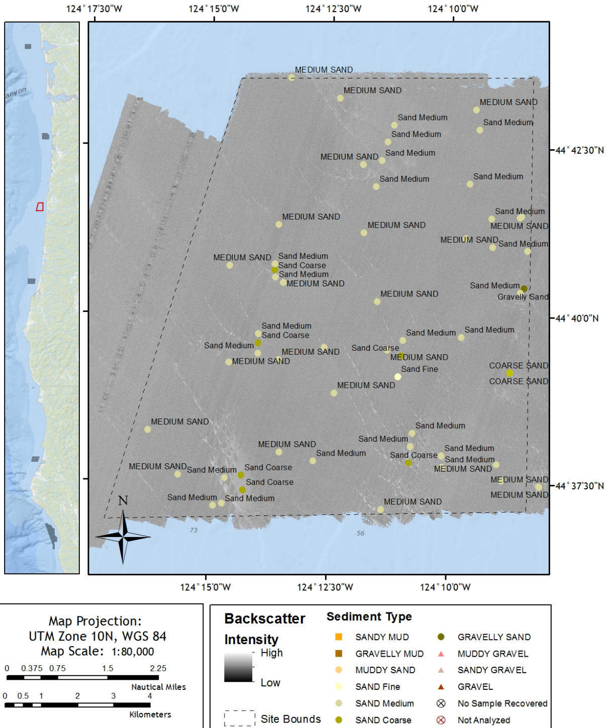
Figure 68. Multibeam backscatter data collected at Newport, OR Sediment textural classifications are plotted over the Reson 8101 (240 kHz) multibeam backscatter) data.
