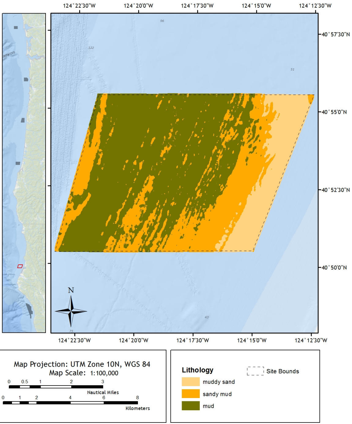
Figure 40. Seabed substrates at Eureka, CA
