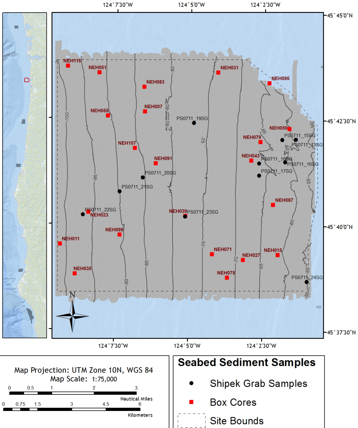
Figure 62. Shaded-relief multibeam bathymetry data collected at Nehalem, OR Sediment sample are plotted over the Reson 8101 (240 kHz) multibeam bathymetry data.
