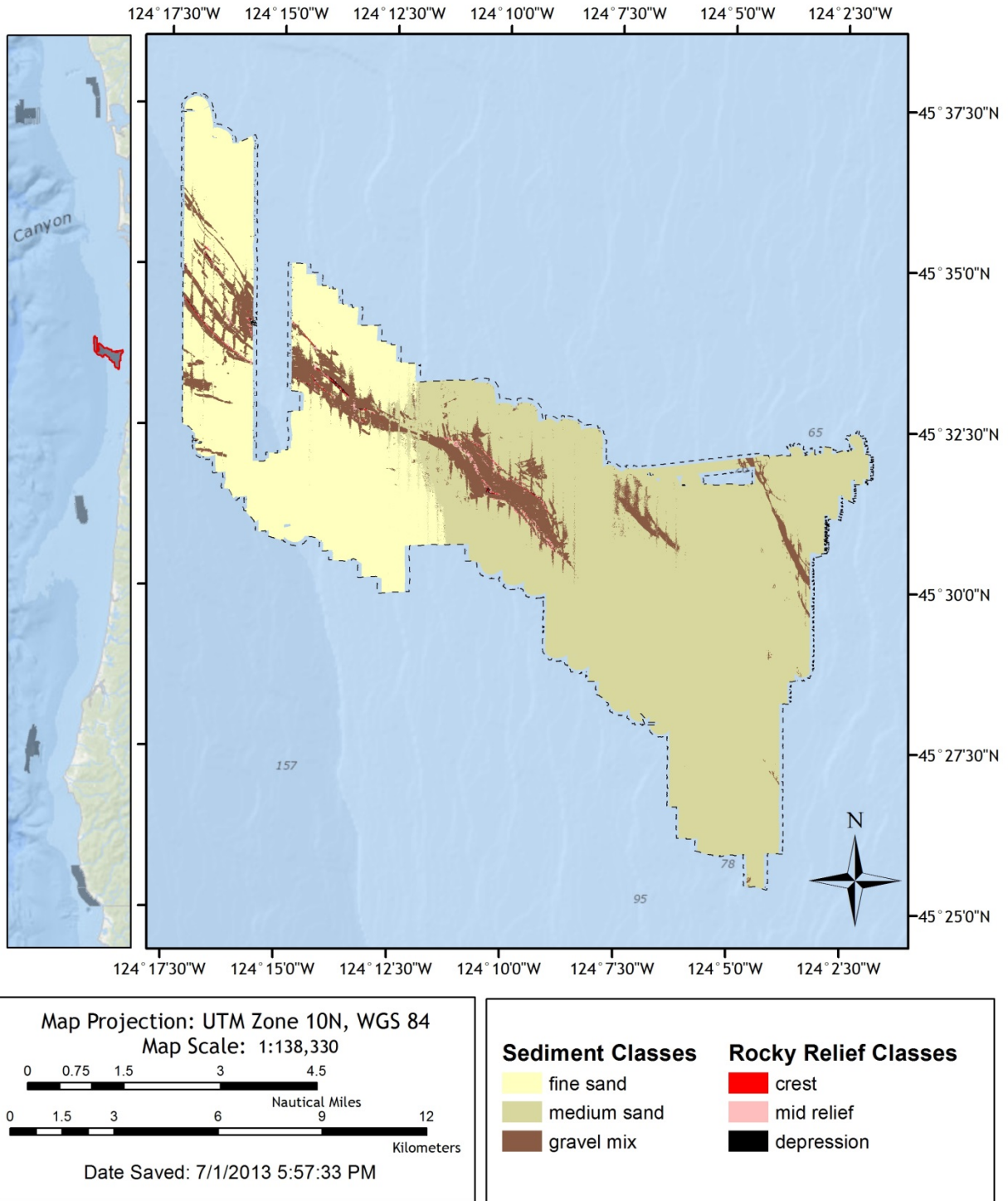
Figure 83. Seabed Substrates at Cape Falcon Fault, OR
