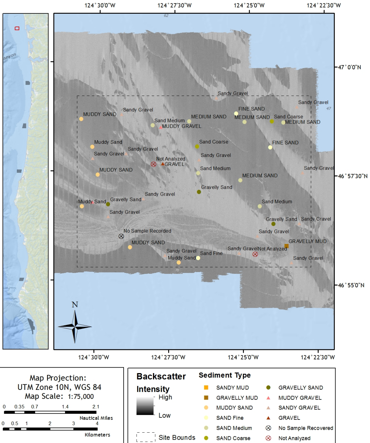
Figure 60. Multibeam backscatter data collected at Grays Bank, WA Sediment textural classifications are plotted over the Reson 8101 (240 kHz) backscatter data.
