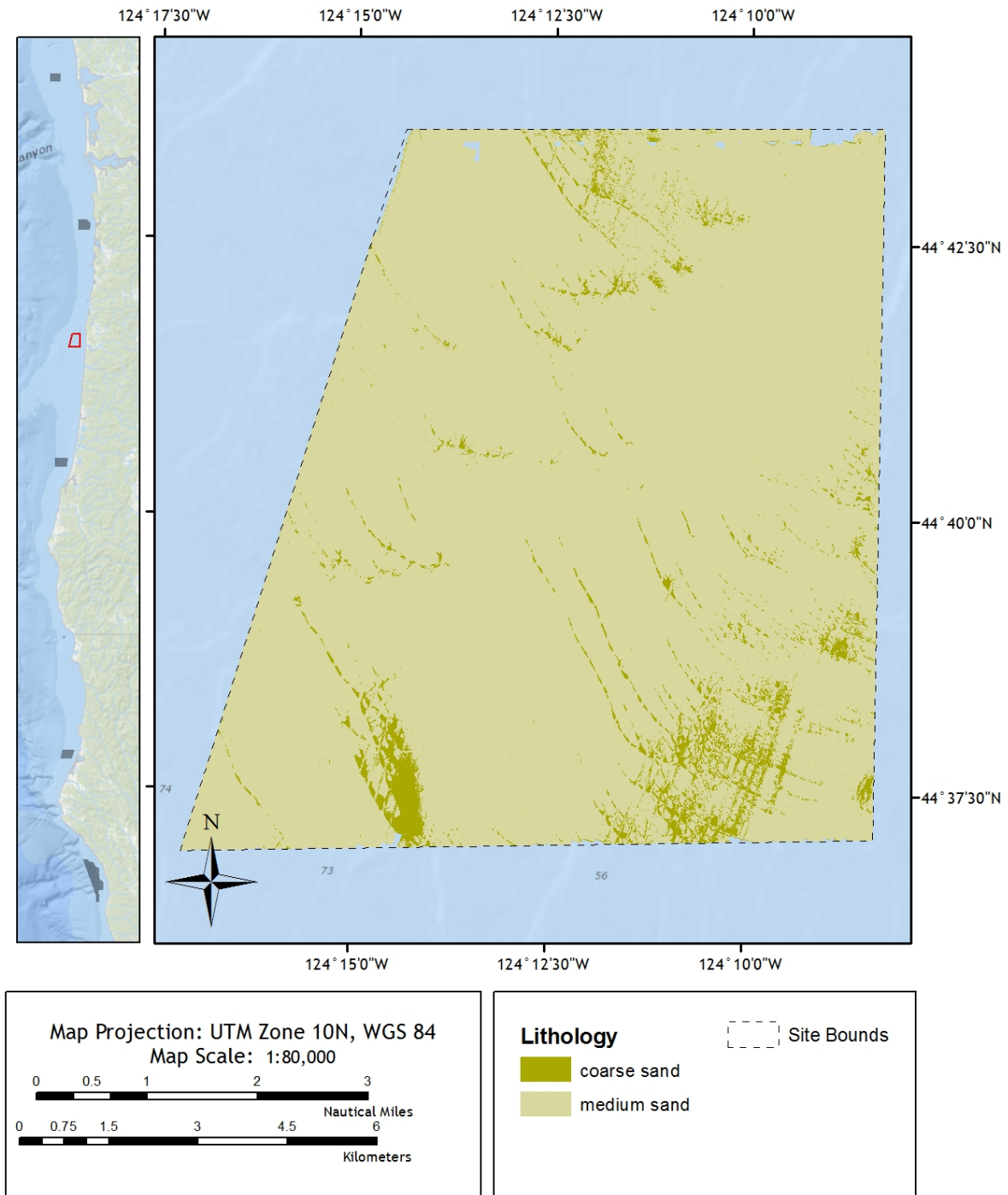
Figure 25. Seabed substrates at Newport, OR
