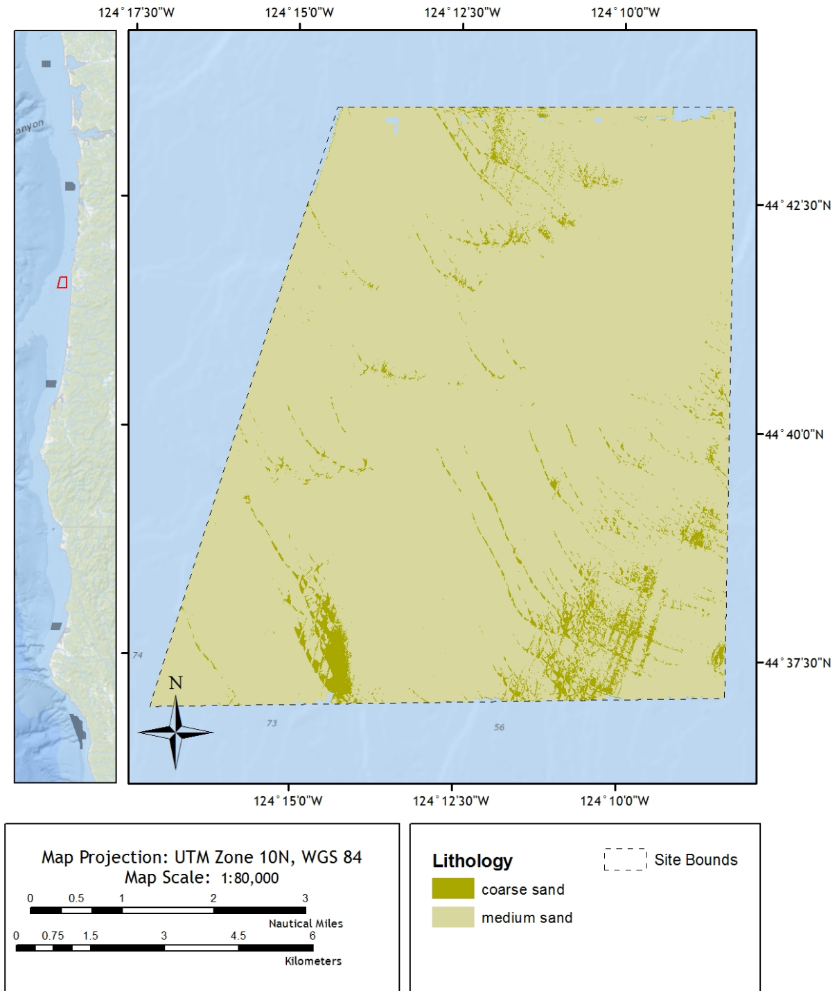
Figure 69. Seabed substrates at Newport, OR
