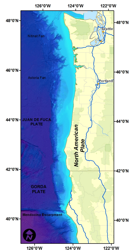
Figure 2. The tectonic setting of the Cascadia Subduction Zone
