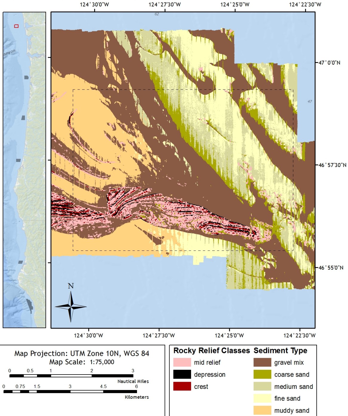
Figure 61. Seabed substrates at Grays Bank, WA
