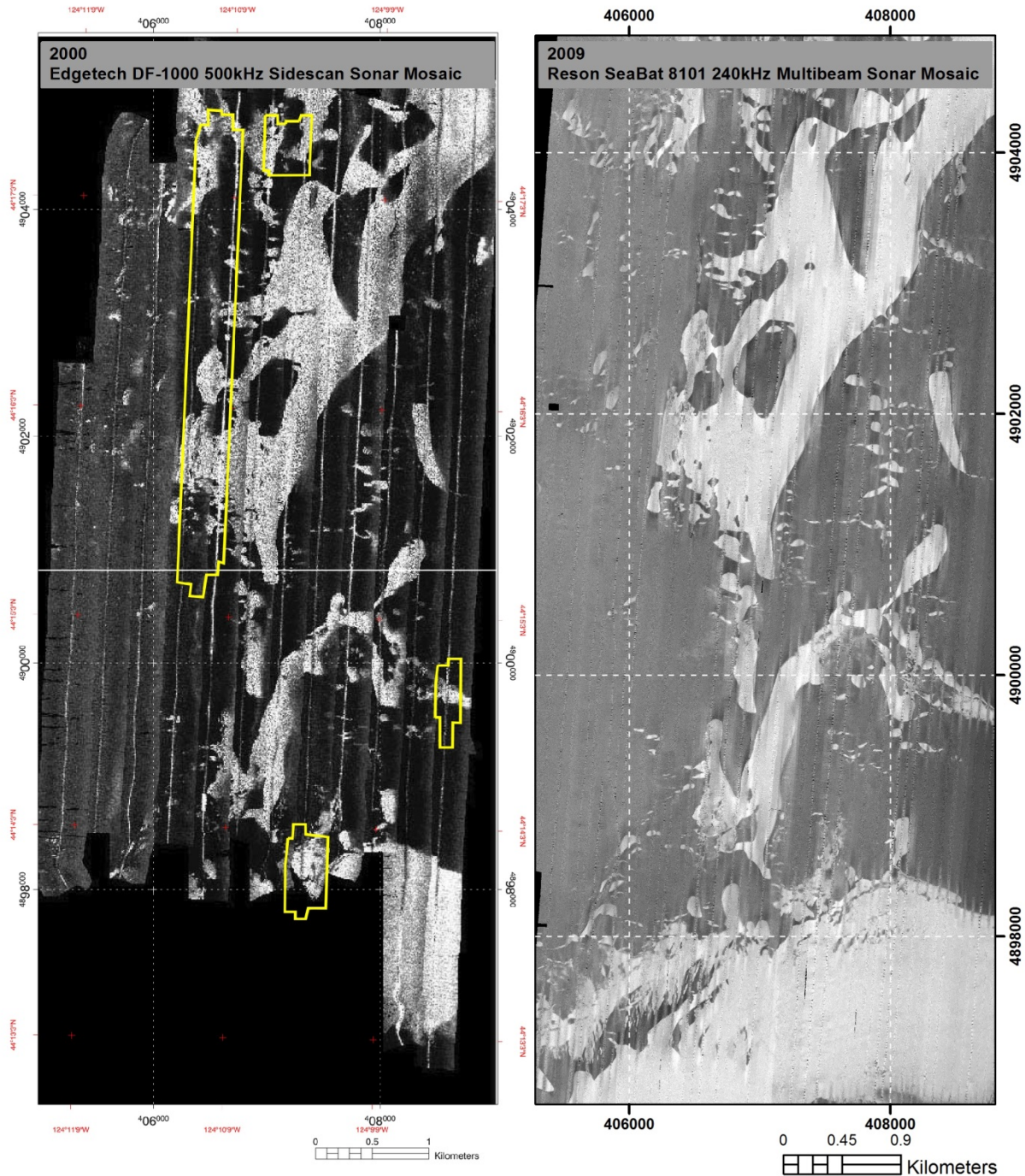
Figure 5. Repeat backscatter surveys (2000 left & 2009 right) at Cape Perpetua, Oregon Repeat surveys spanning nine years show little if any change in scour depression location. Bright backscatter intensity areas in the northern and central portions of the imagery are known to be scour depressions from bathymetry and ROV observation. Backscatter image on left from Fox et al. 2004.
