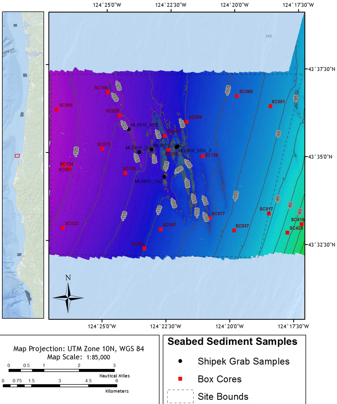
Figure 35. Color shaded-relief multibeam bathymetry data collected at Siltcoos, OR. Sediment samples are plotted over the Reson 8101 (240 kHz) multibeam data.
