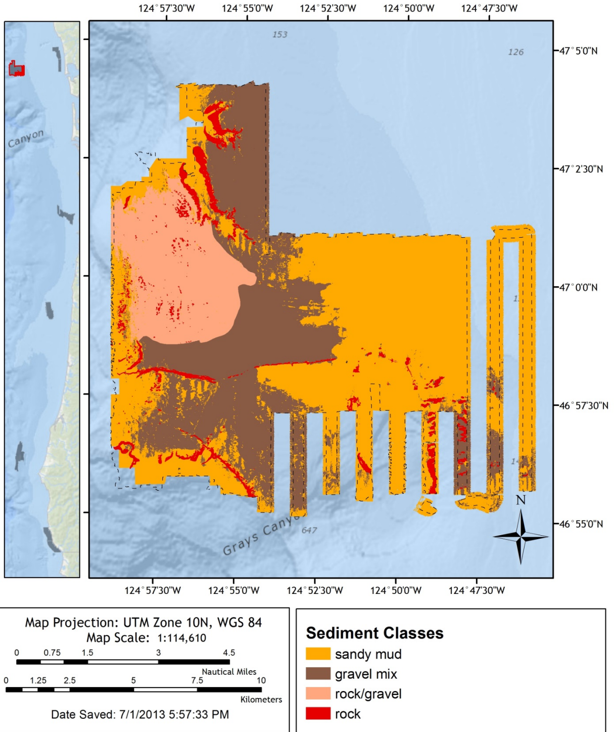
Figure 82. Seabed substrates at Sponge Reef Site, WA
