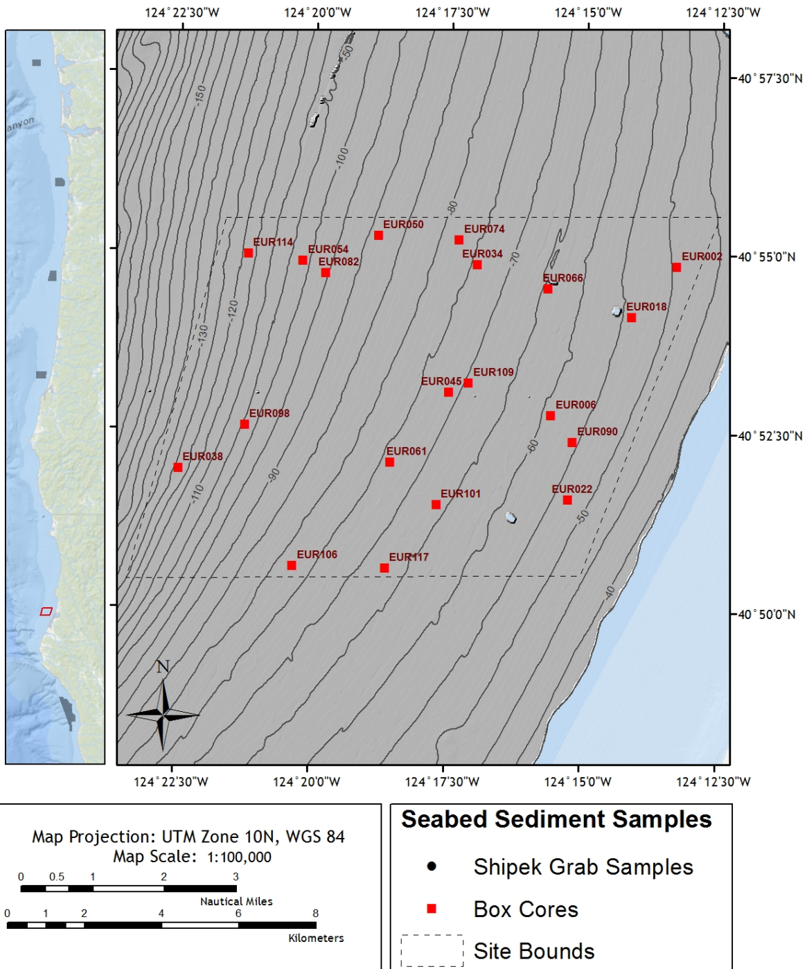
Figure 38. Multibeam bathymetry data collected at Eureka, CA Sediment sample stations plotted over the Reson 8101 (240 kHz) multibeam bathymetry data.
