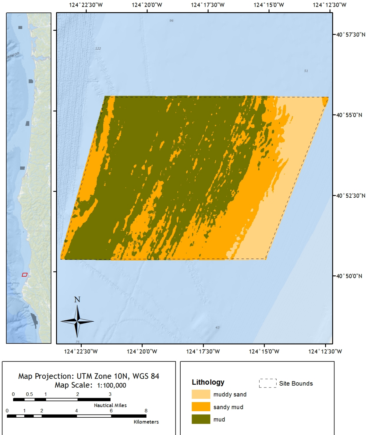
Figure 76. Seabed substrates at Eureka, OR
