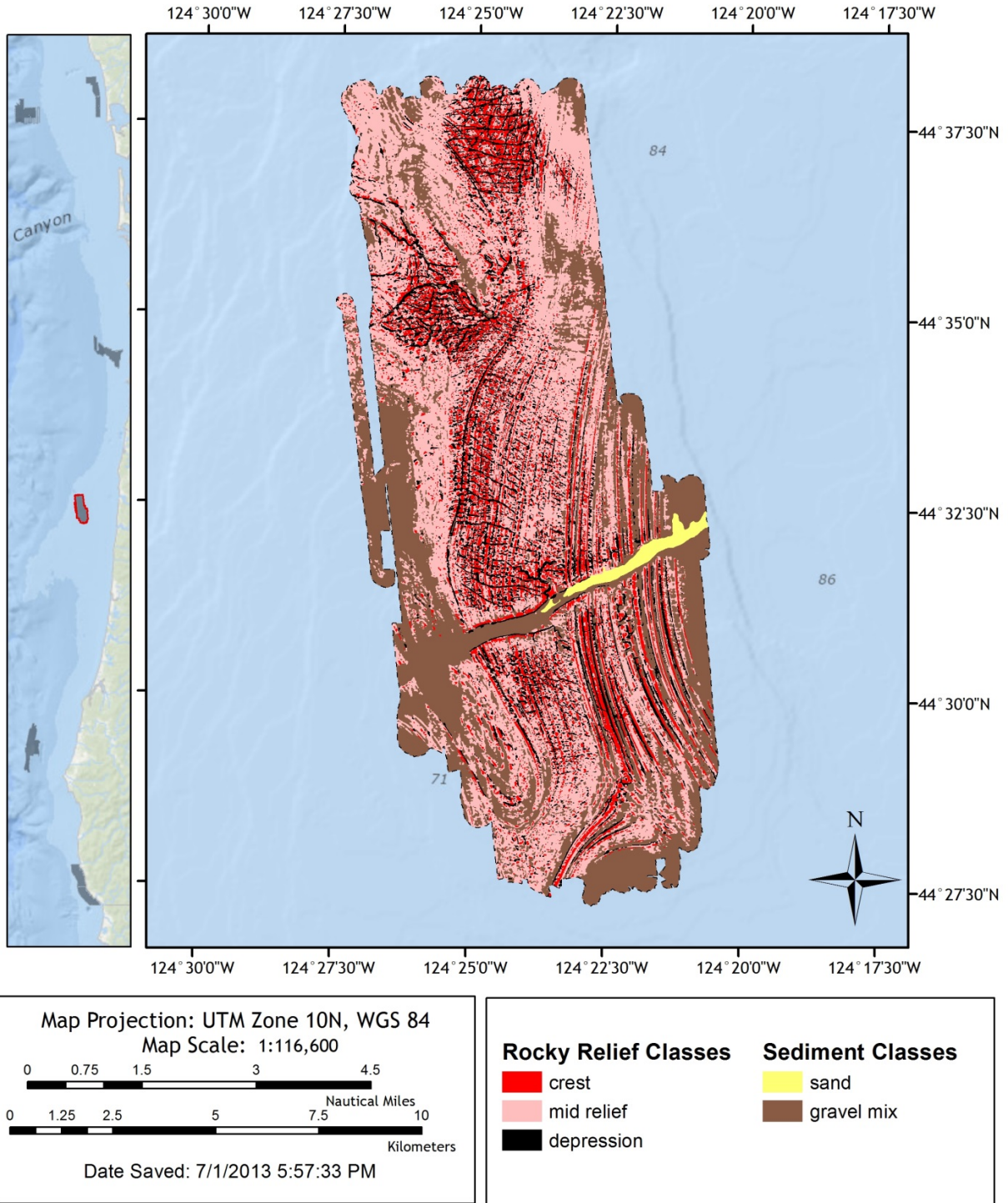
Figure 84. Seabed substrates at Stonewall Bank, OR
