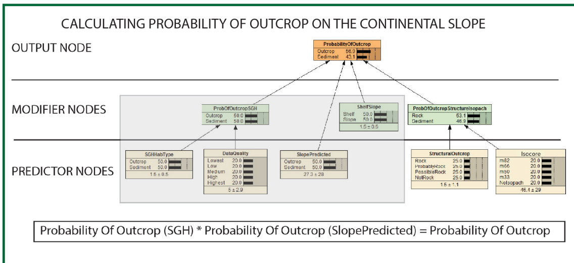
Figure 12. The Rock Outcrop Model Bayes net structure and differences between predicting outcrop on the continental shelf and slope
