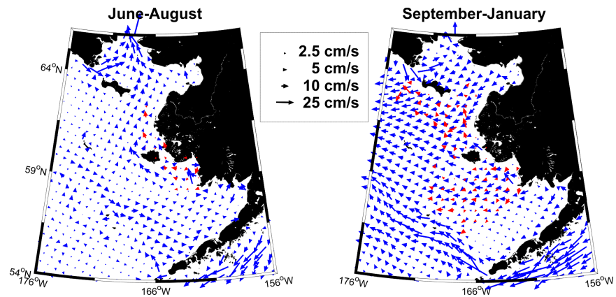
Figure 20: Comparison of model (blue) and drifter (red) velocities.
