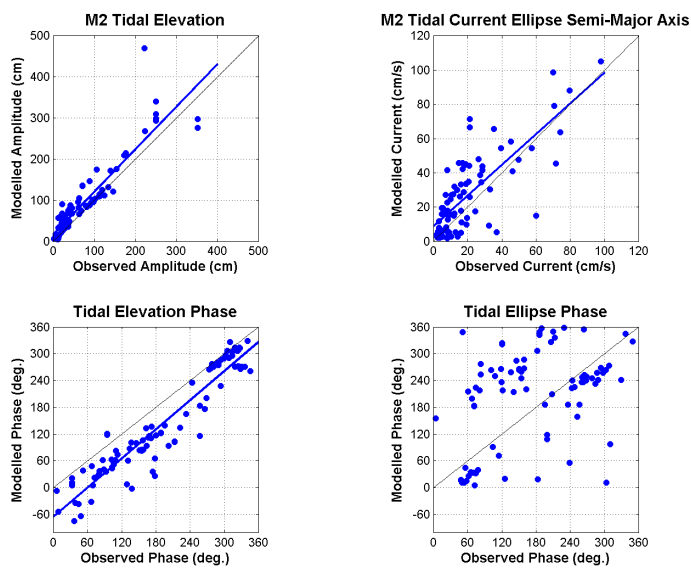
NEP5 Run35: Zeta and Vertical Average Currents vs. Observations
