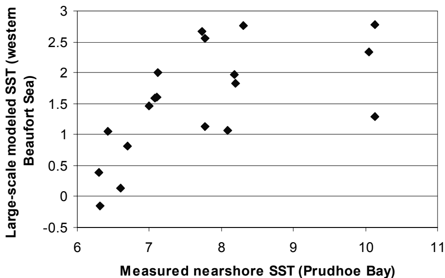
Figure 26. Comparison of measures sea-surface temperatures (SST) at Heald Point in Prudhoe Bay and large-scale model-based SST for the western Beaufort Sea.
