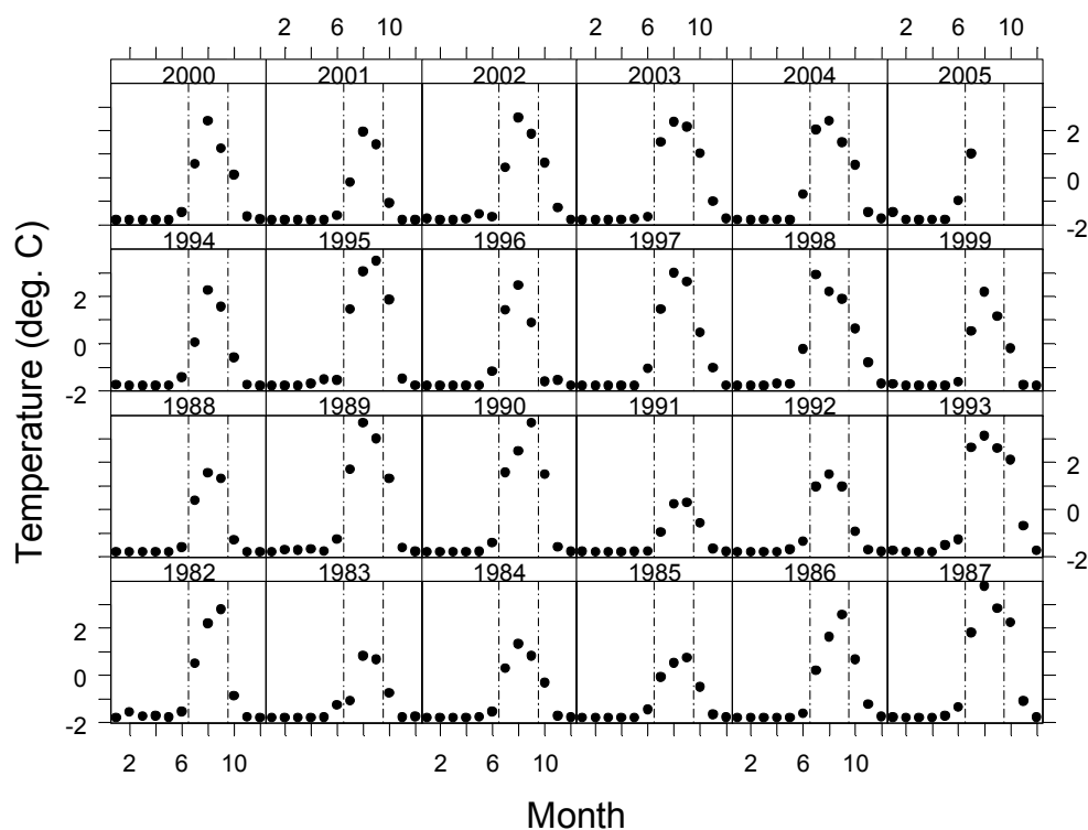
Figure 25. Average sea-surface temperature (Optimum Interpolation v.2 SST) off the Colville River / Prudhoe Bay region (70–71°N, 146–152°W) by month and year, 1982–2005.
