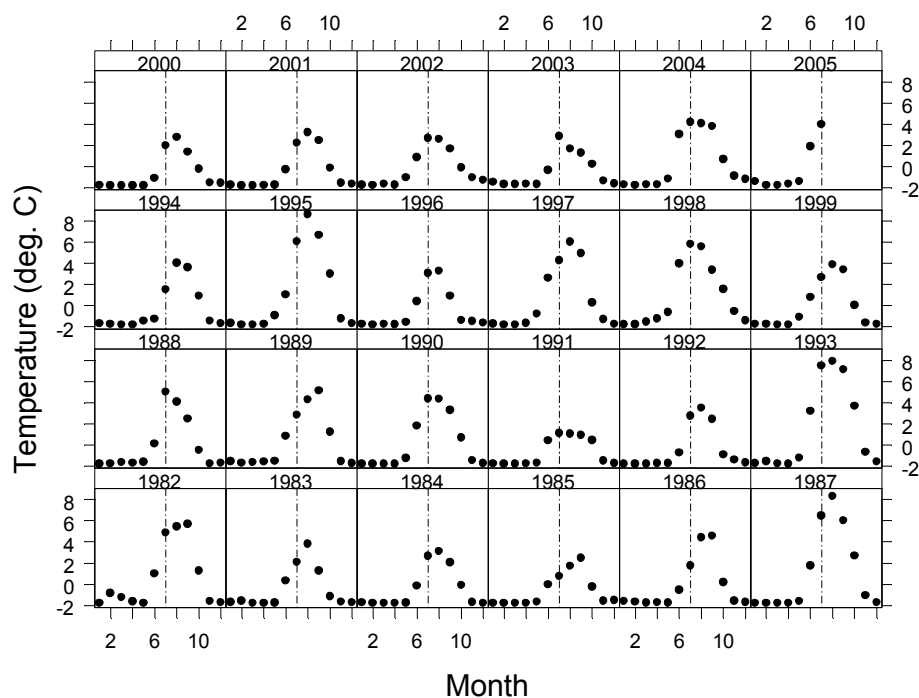
Figure 23. Average sea-surface temperature (Optimum Interpolation v.2 SST) off the mouth of the Mackenzie River (69–70°N, 136–142°W) by month and year, 1982–2005.
