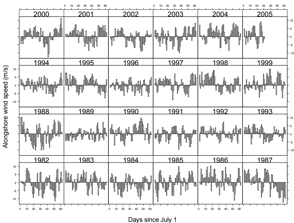
Figure 20. Daily average wind speeds along the Beaufort Sea coast as estimated by NCEP/NCAR for July and August of each year from 1982–2005. Positive winds denote alongshore wind component from ESE to WNW.
