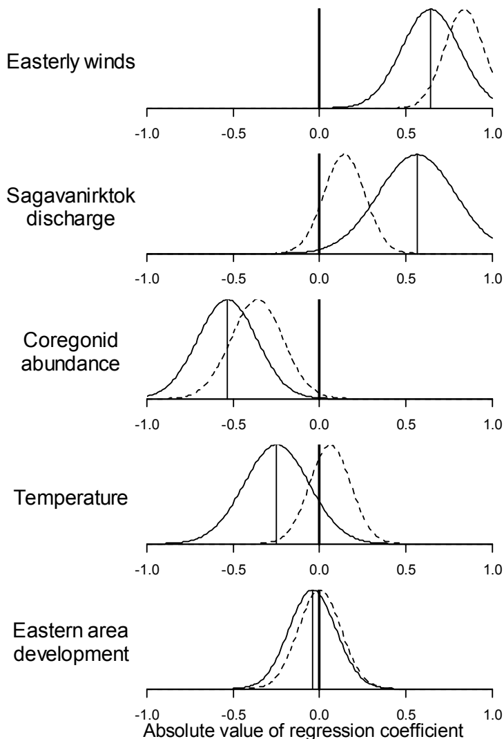
Figure 133. Sensitivity of Arctic cisco young-of-year recruitment to environmental indicators and one development indicator. Solid lines denote probability distribution (relative scale) of regression coefficients based on the “full” model (i.e. a multiple linear regression including all 5 variables), whereas dashed lines denote probability distributions based on a model that include the wind effect plus the variable specified on the left.
