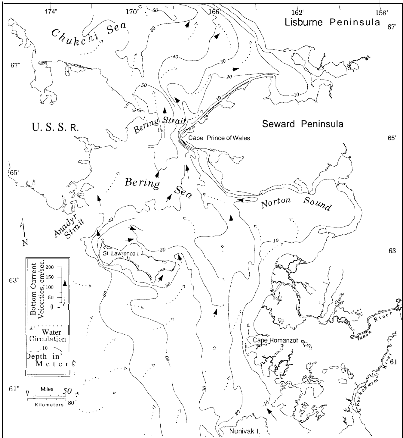
FIGURE 2. 12—Offshore water circulation and maximum bottom current velocities from measurements in the northern Bering Sea. (Adapted from Nelson et al. 1981.)
