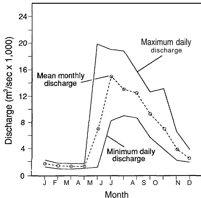
FIGURE 2.3—Annual hydrography of Yukon River discharge at Pilot Station, 1975–86. Dashed line represents 10-year averages of monthly mean discharge estimates. Solid lines represent 1-day extreme discharges for each month. (Adapted from McDowell et al. 1987.)
