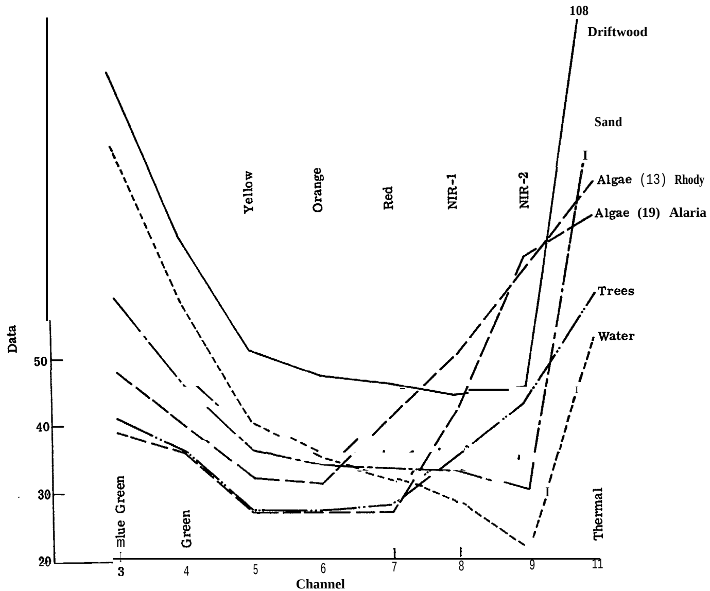
FIGURE 29. REPRESENTATIVE SPECTRAL SIGNATURES USED IN THE UNSUPERVISED CLASSIFICATION OF CAPE YAKATAGA.
