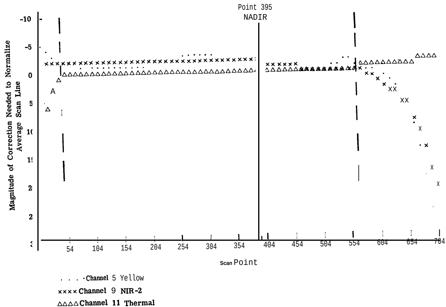
FIGURE 4. SHAPE OF THE AVERAGE SCAN LINE OVER WATER FOR SELECTED CHANNELS.
