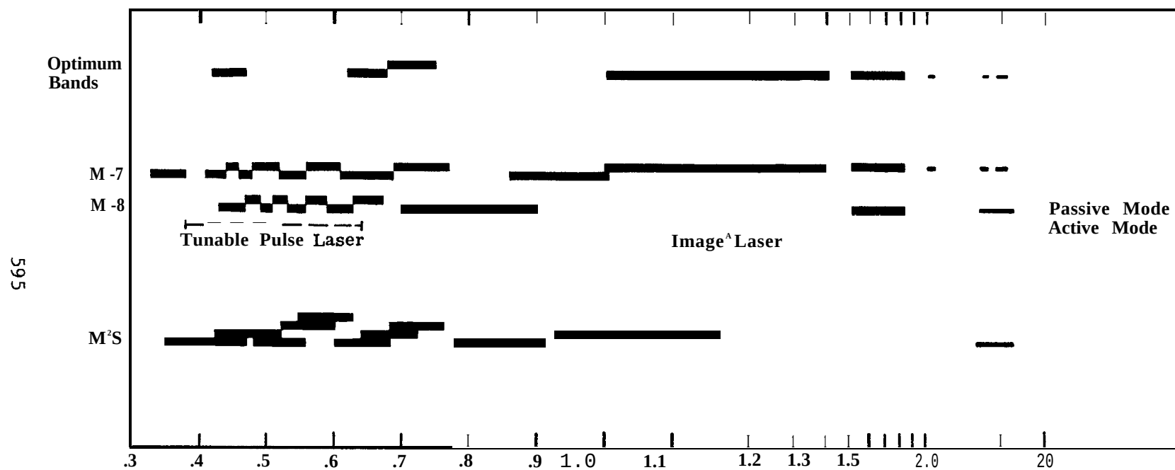
FIGURE 27. COMPARISON OF OPTIMUM SPECTRAL BANDS FOR VEGETATION ANALYSIS WITH THOSE OF THE M -7, M -8, AND M 2 S SCANNERS.
