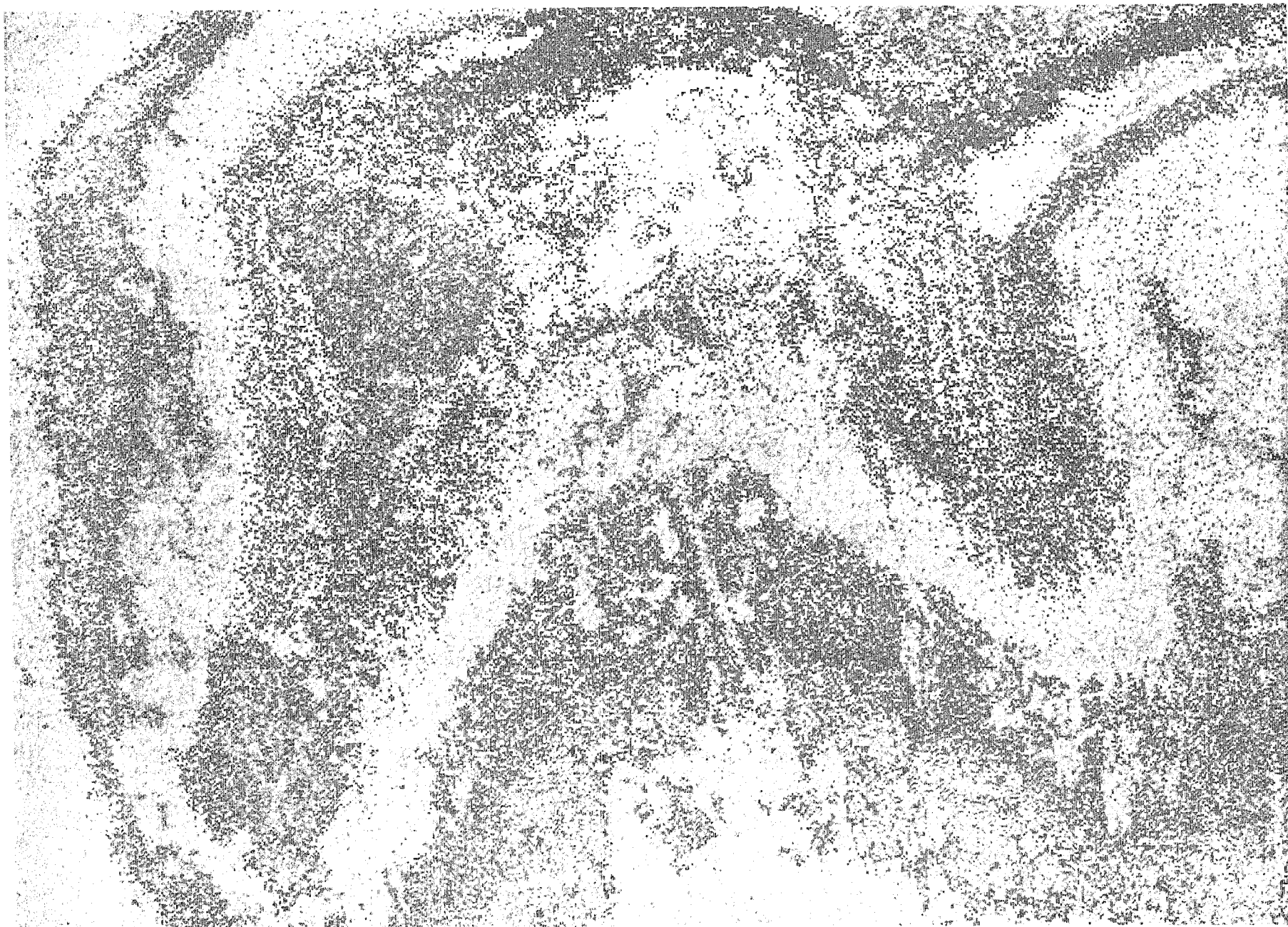
FIGURE 15. SUPERVISED RECOGNITION MAP OF LATOUCHE ISLAND: 4 CHANNELS OF REFLECTED RADIATION/INTERACTIVE MODE/MIDAS COMPUTER
