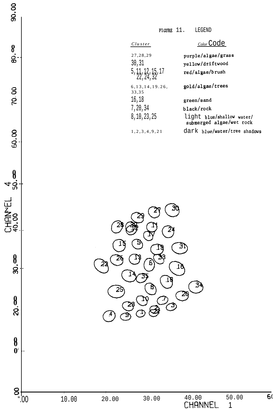
FIGURE 11. EPLLOT OF CLUSTERINGDERIVED TRAINING SETS USED IN UNSUPERVISED RECOGNITION PROCESSING OF THE ZAIKOF BAY DATA SET.
