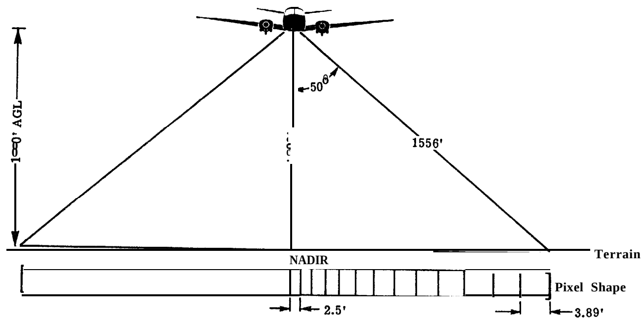
FIGURE 30. SCAN ANGLE GEOMETRY OF AIRCRAFT MSS DATA.
