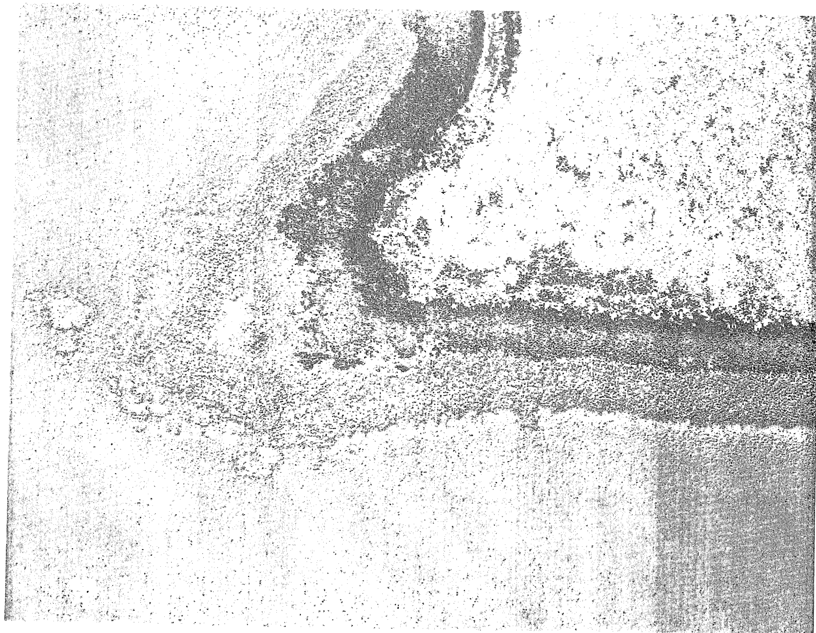
FIGURE 8. SUPERVISED RECOGNITION MAP OF ZAIKOF BAY: 9 CHANNELS OF REFLECTED RADIATION/NO GROUND TRUTH/7094 COMPUTER
