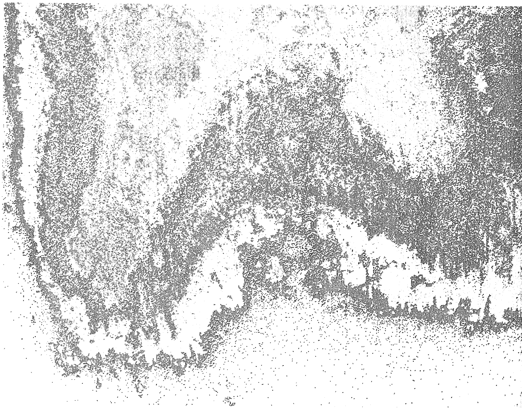
FIGURE 14. SUPERVISED RECOGNITION MAP OF LATOUCHE ISLAND: 9 CHANNELS OF REFLECTED RADIATION/NO GROUND TRUTH/7094 COMPUTER
