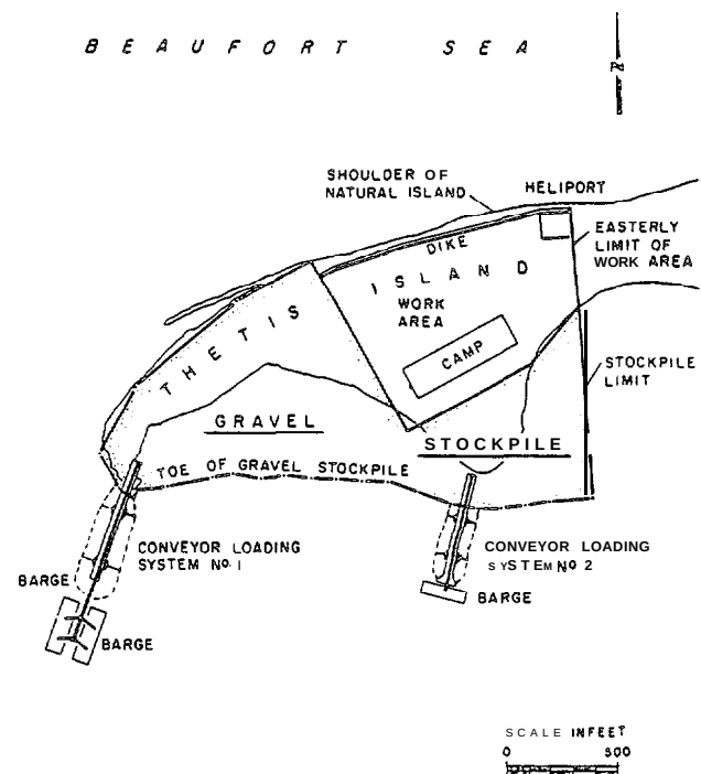
Fig. 4—Layout of Thetis Island work area
