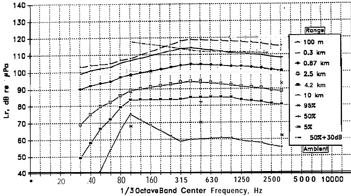
FIG. E. 15 TWIN OUTDRIVE (20KT) OPE RATING IN NORTON BASIN Surface Layer Conditions
