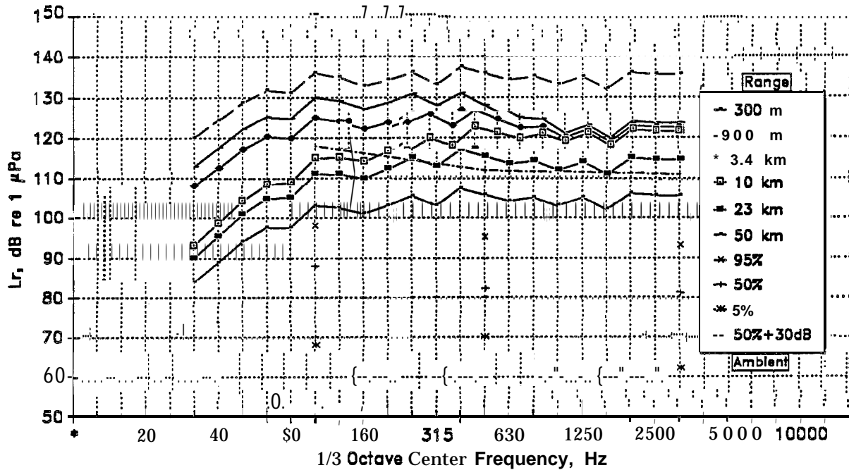
FIG. E 16 ICEBREAKER OPERATING IN NORTH ALEUTIAN BASIN Neutral Gradient Conditions
