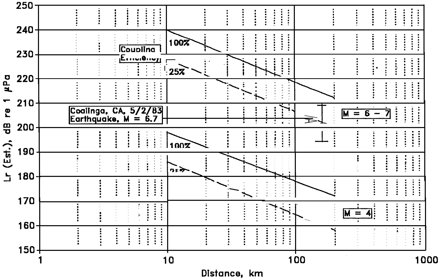
FIG. 3.8 EST MATED OVERALL SOUND LEVEL FOR SHORT TERM EARTHQUAKE EVENTS ALONG THE ALASKA PENINSULA
