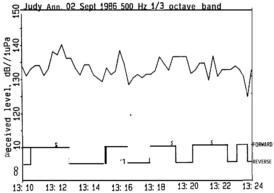
C. 500 Hz 1/3 Octave Band
