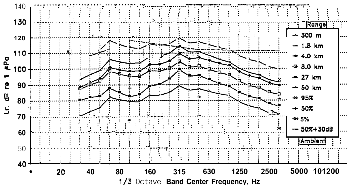
FIG. E.19 DRILLSHIP (EXPLORER II) OPERATING IN NORTH ALEUTIAN BASIN Surface Layer Conditions
