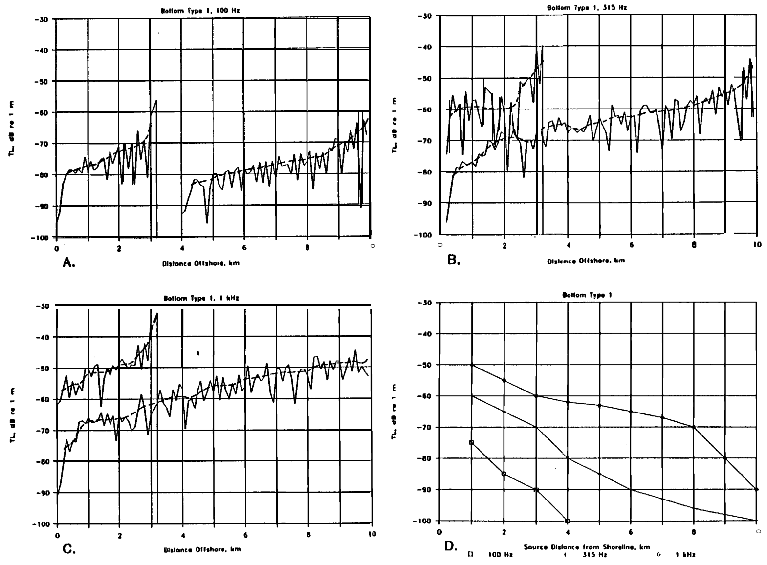
Figure 4.5. Offshore Transmission Loss for Sloping Bottom vs Distance Offshore A. Bottom Type 1, 100 Hz; B. Bottom Type 1, 315 Hz; C. Bottom Type 1, 1 kHz; D. Bottom Type 1, TL vs Source Range Offshore.
