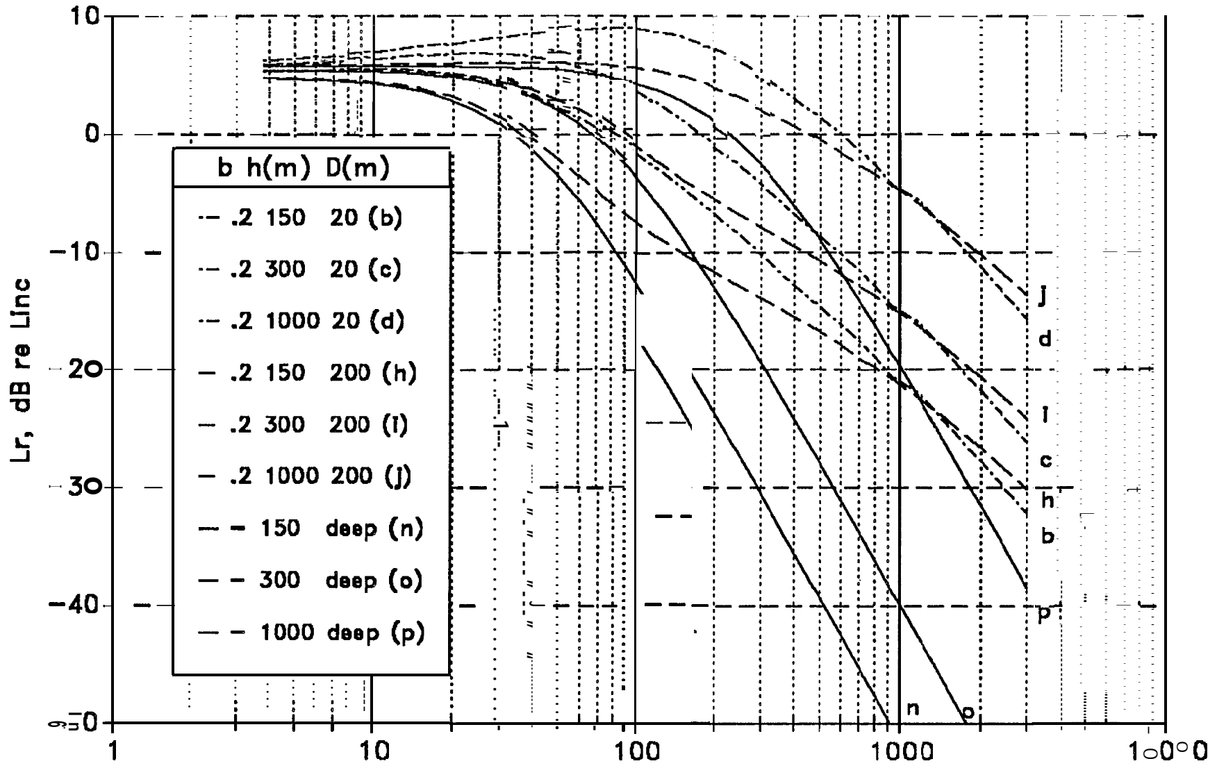
FIG. 4.10 AIR TO SHALLOW WATER Receiver depth 5
