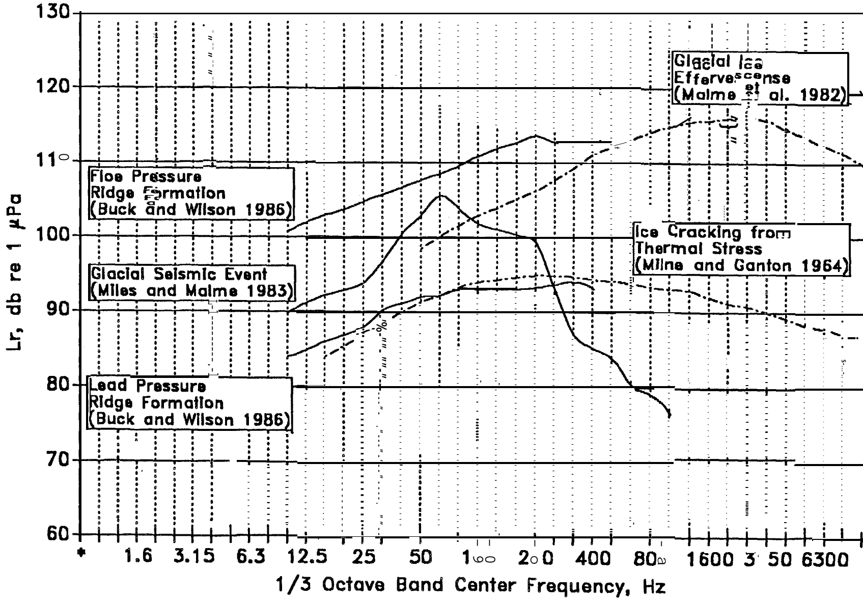
FIG. 3.9 UNDERWATER NOISE SPECTRA FROM CE-RELATED SOURCES
