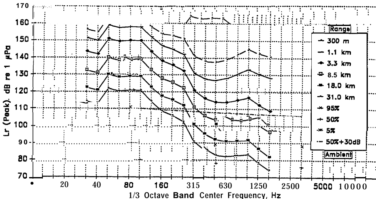
FIG. E.4 AIRGUN ARRAY (WESTERN POLARIS) OPERATING IN THE CHUKCHI SEA Summer, 50% Ice Cover
