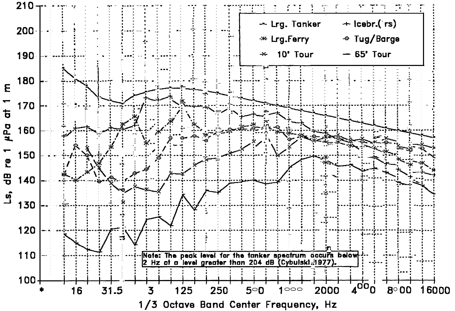
FIG. 3.14 REPRESENTATIVE SHIPS AND BOATS
