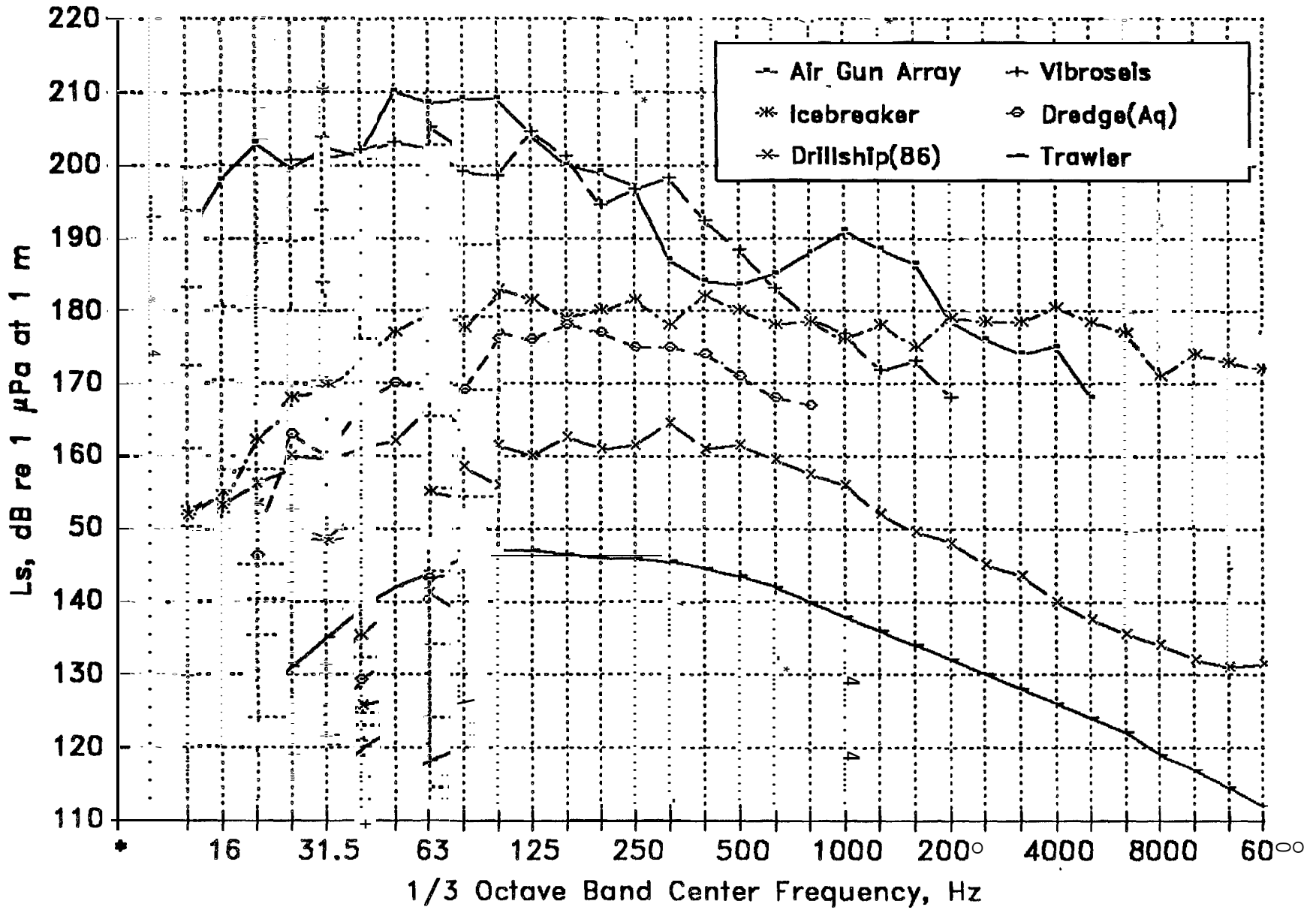
F G. 3. 3 REPRESENTATIVE INDUSTRIAL NOISE SOURCES
