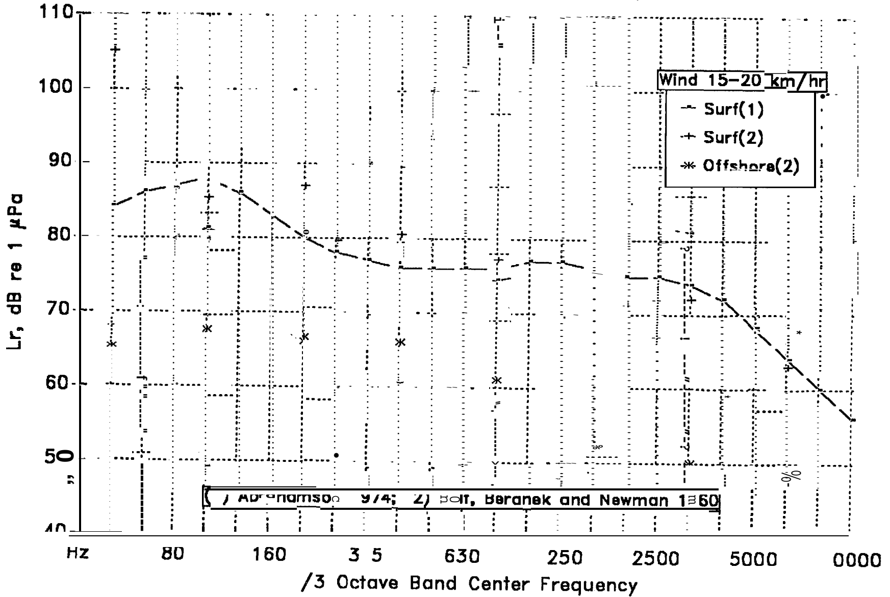
FIG. 3.1° AIRBORNE AMBIENT NOISE SPECTRA N COASTAL AREA (From Malme and Smith 1988)
