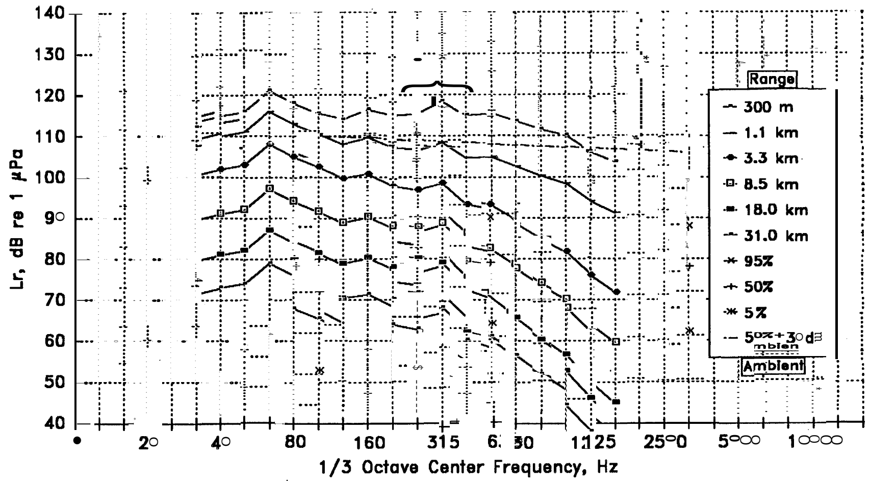
F G. 5.7 DRILLSHIP (EXPLORER II) OPERATING IN THE CHUKCH SEA Summer, 50% Ice Cover
