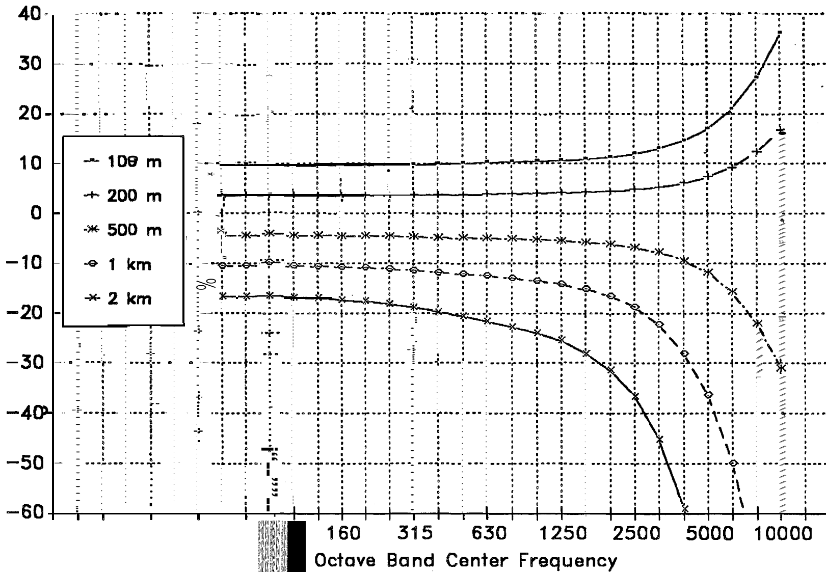
FIG. 4.1 CORRECTION TO 300 M REFERENCE SPECTRA FOR AIRCRAFT FLYOVER AT OTHER ALTITUDES (Standard Day Conditions)
