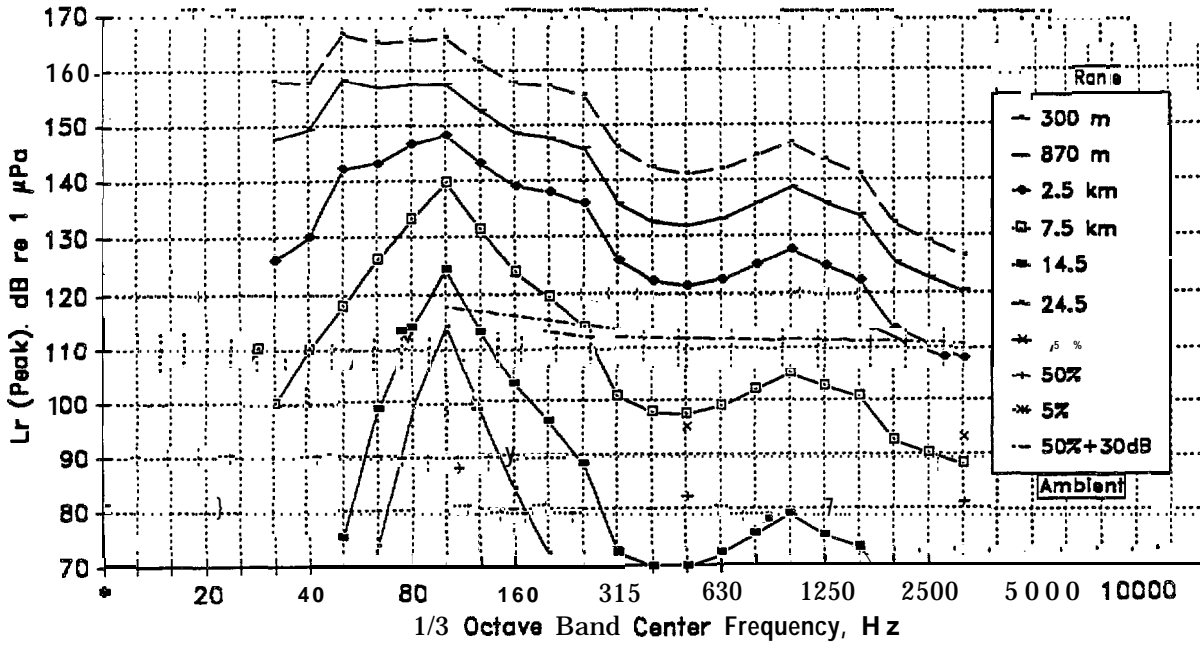
FIG. E.11 AIR GUN ARRAY (WESTERN POLARIS) OPERATING IN NORTON BASIN Surface Layer Conditions
