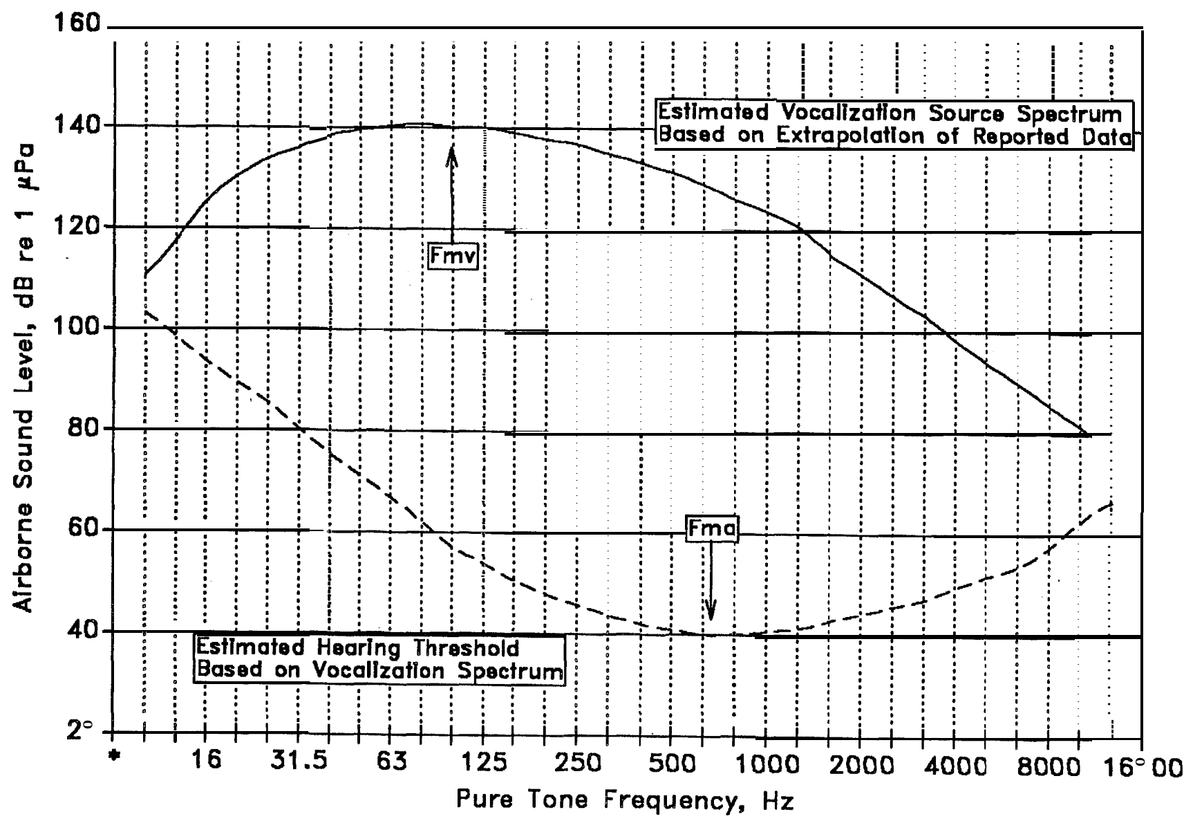
FIG. D.2 ESTIMATED GRAY WHALE VOCALIZATION AND AUDITION CHARACTERISTICS
