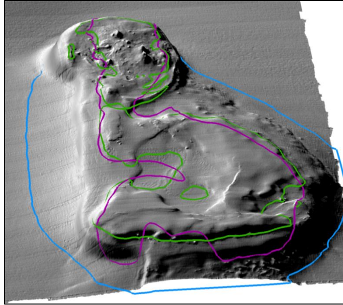
Figure 1. Example of a multibeam sonar-derived bathymetry dataset (gray) depicting the relief of a topographic feature. The different colored lines illustrate different hypothetical boundaries that could be drawn based on varying source bathymetry.
