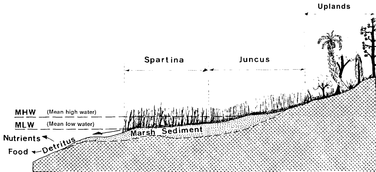
Figure 21. Zonation in Florida salt marsh dominated by Spartina alterniflora and Juncus roemerianus (from Darovec et al. 1975).
