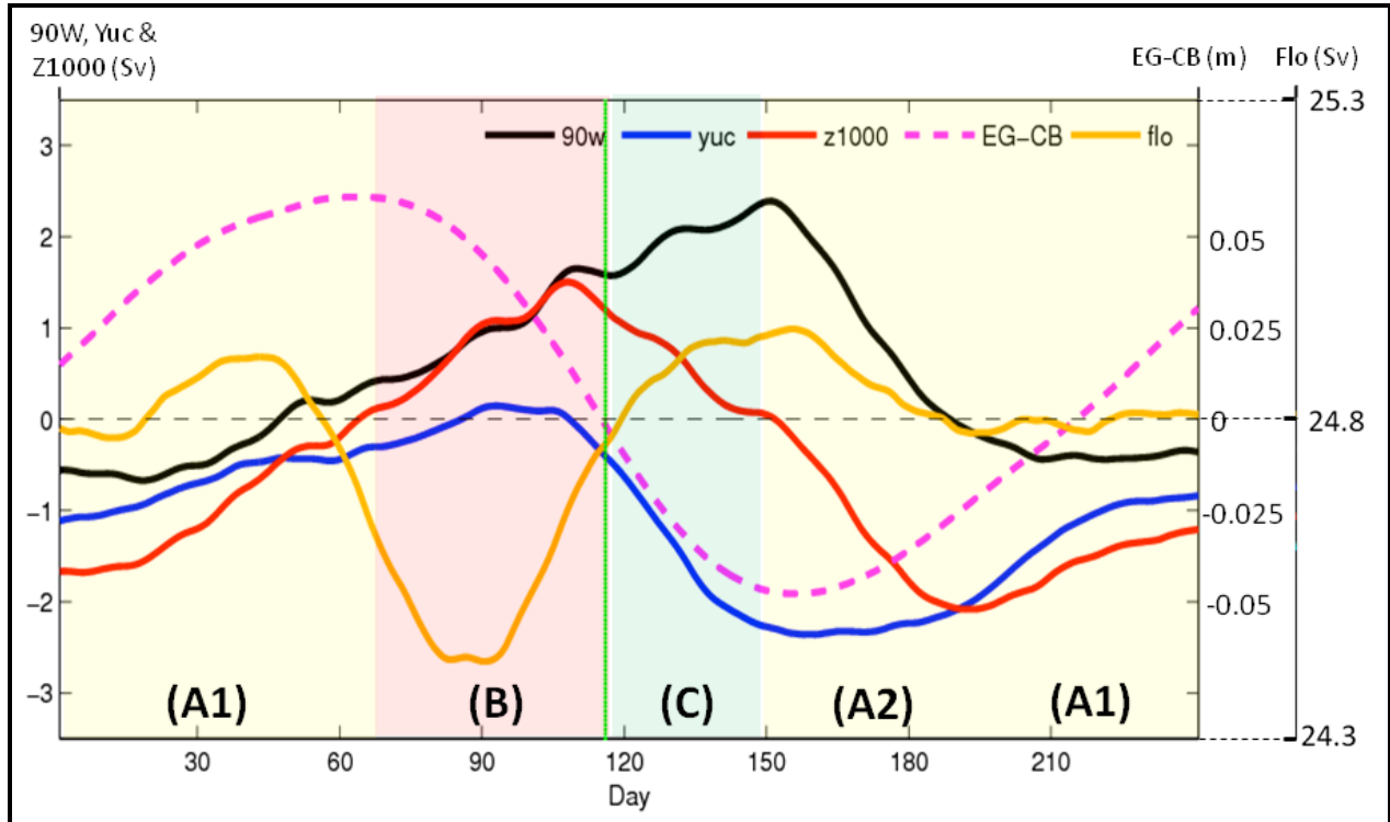
Figure 3.1. Ensemble averaged time-series of transports across the boundaries of the deep eastern Gulf control volume (see text) across 90^\circ\text{W} (black), Yucatan Channel (blue), and z = 1000 m horizontal plane (red)). Also plotted are the Florida transport (gold curve) and the difference between the area-mean SSH in the eastern Gulf and the Caribbean Sea (dashed). The time-axis is over the Loop Current Cycle of 240 days with Stages A, B and C as discussed in text (see also Chang and Oey, 2011). To show more clearly the relationship between the different variables during a Loop Current Cycle, a 30-day running-average has been applied to all the time series.
