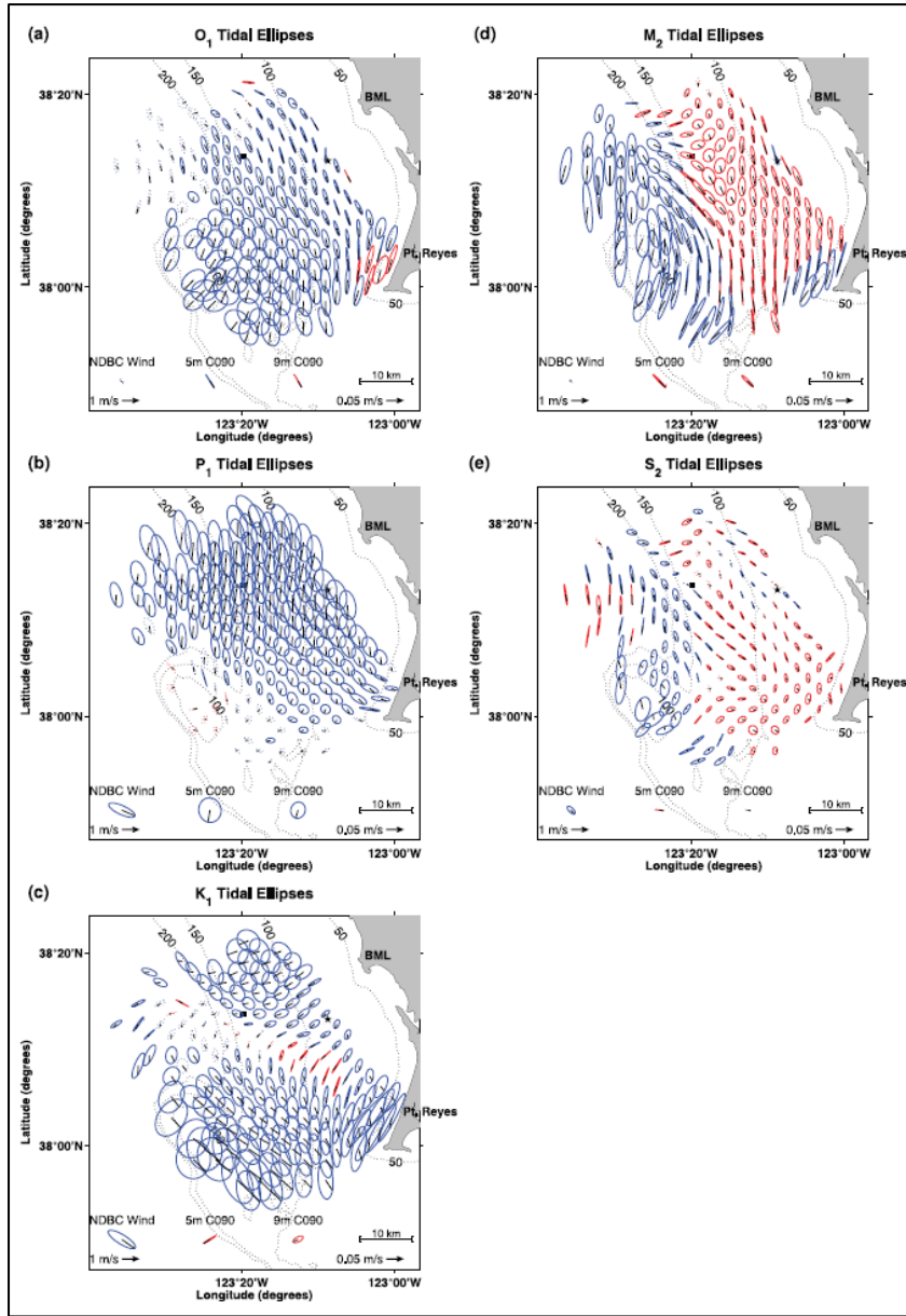
Figure 1.39. Tidal ellipses at (a) O_1 , (b) P_1 , (c) K_1 , (d) M_2 , and (e) S_2 frequencies. Clockwise rotation ellipses are shown in blue, and counterclockwise ellipses are in red.
