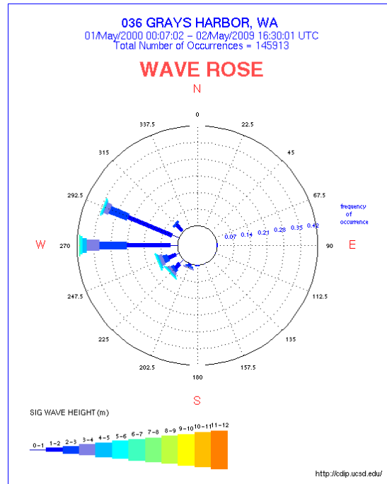
Figure 1.49. Significant wave height wave rose for CDIP buoy 036 Grays Harbor, Washington.
