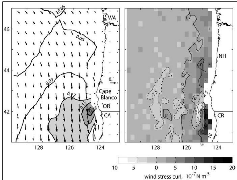
Figure 1.23. QuikSCAT mean July wind stress (left) and wind stress curl (right), 2002-2003. (left) Wind stress vectors and vector magnitudes ( \text{N/m}^2 ). Every second vector of the 0.25-degree grid is shown.
