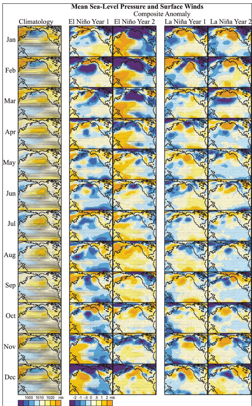
Figure 1.16. Mean sea level pressure with surface wind vectors climatology and composite-anomaly maps for El Niño and La Niña years.
