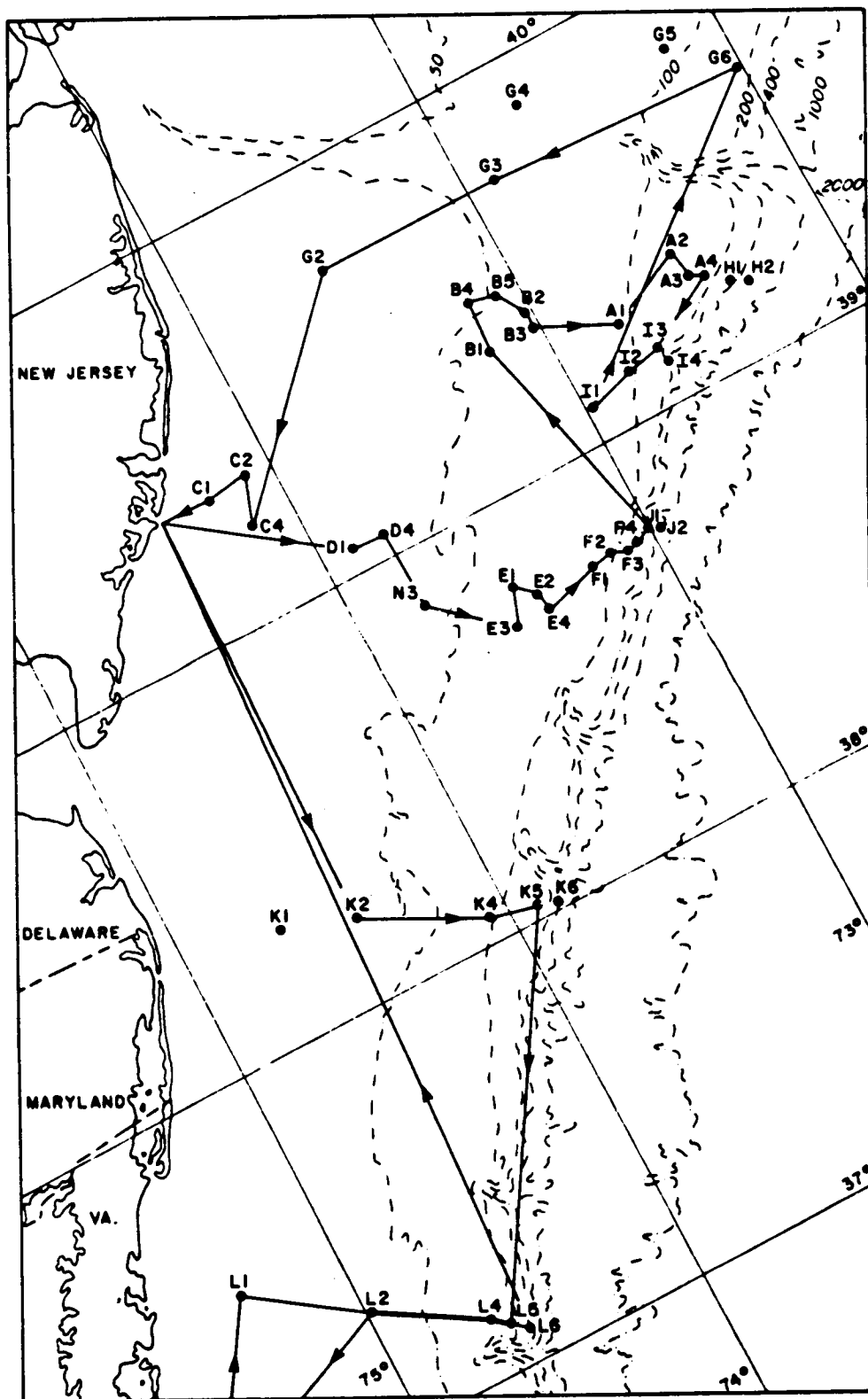
Figure 2-34. Cruise track, R/V H. J. W. Fay, BLM06B, Leg 1, 4-17 February 1977.
