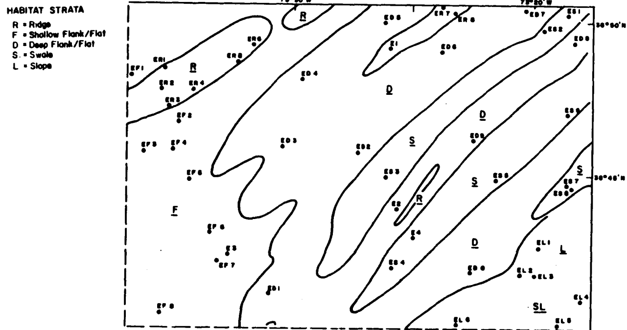
Figure 2-24. BLM05B, Benthic habitat delineation stations, Area E.
