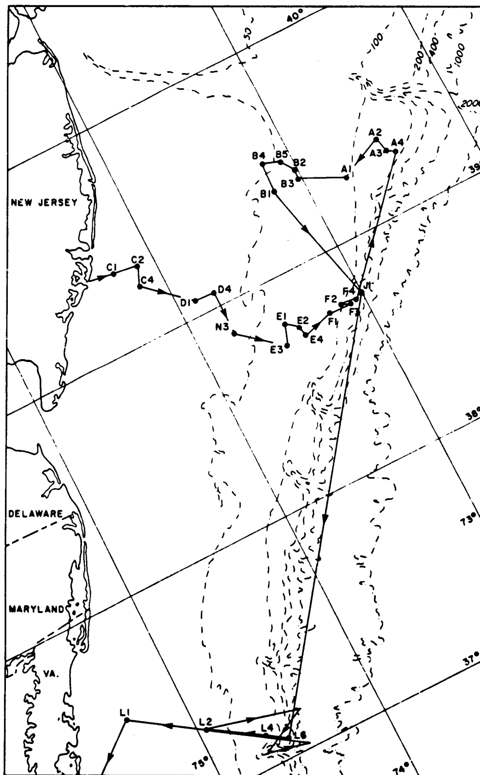
Figure 2-38. Cruise track, R/V H. J. W. Fay , BLM07B, 30 May-5 June 1977.
