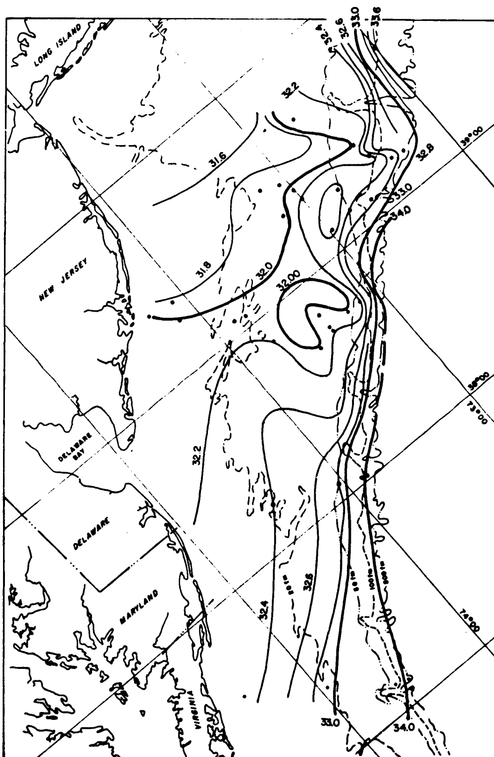
Figure 3-69b. Surface salinity (ppt) distribution in the Middle Atlantic Bight during the period 4-16 August 1977 (Cruise BLM08B).
