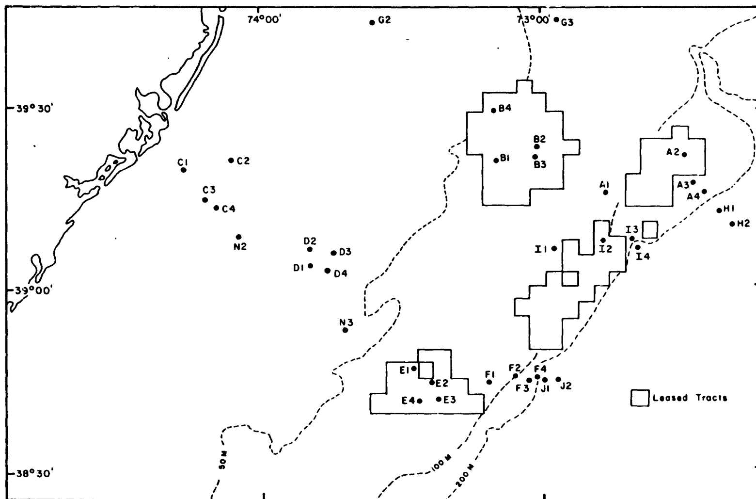
Figure 2-1. Stations in the central study area and tracts leased for oil and gas development in BLM Sale 40.
