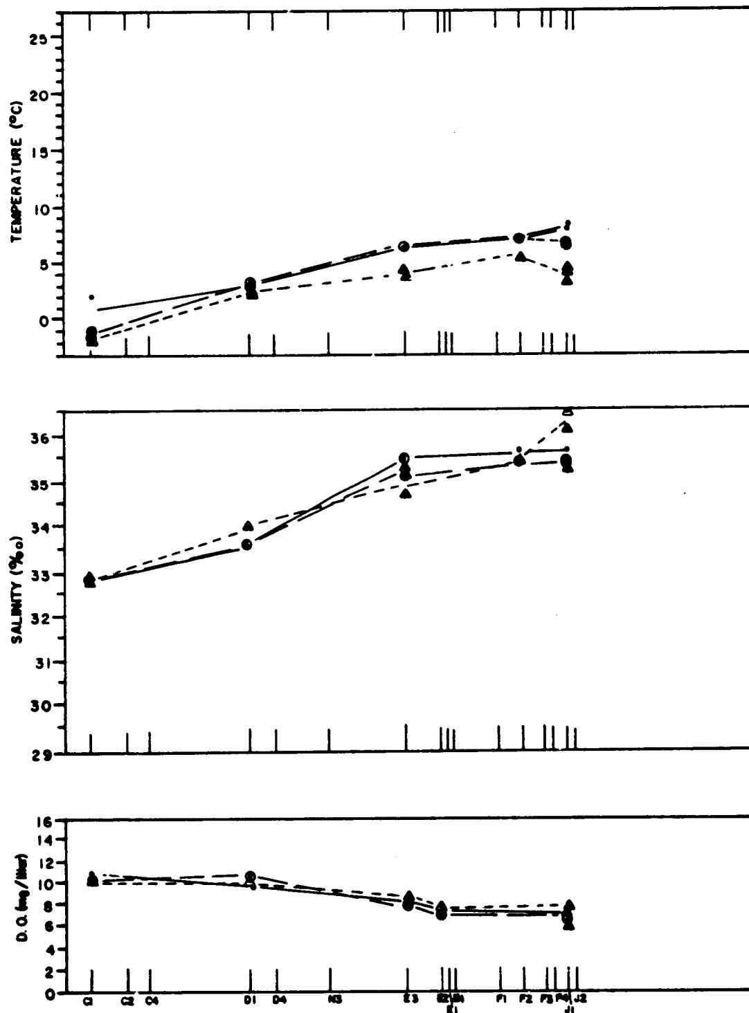
Figure 3-43. Surface (•), mid-depth (◐), and bottom (▲) values of temperature, salinity, and dissolved oxygen measured along section III (Figure 3-6) during cruise BLMO6W.
