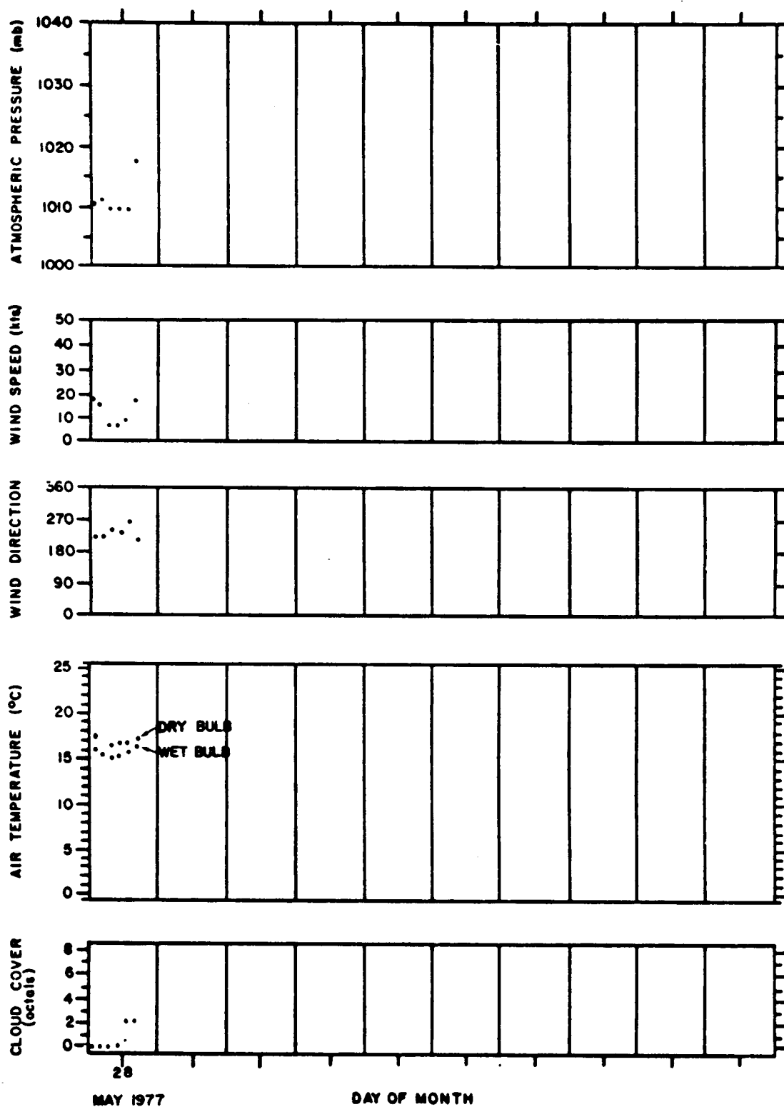
Figure 3-60b. Meteorological data collected during cruise BLM07W on 28 May 1977.
