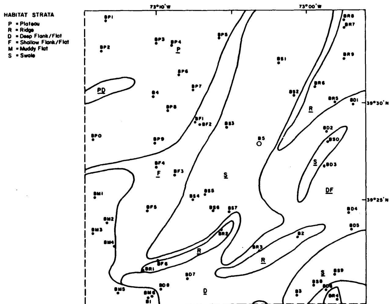
Figure 2-26. BLM05B, Benthic habitat delineation stations, Area B.
