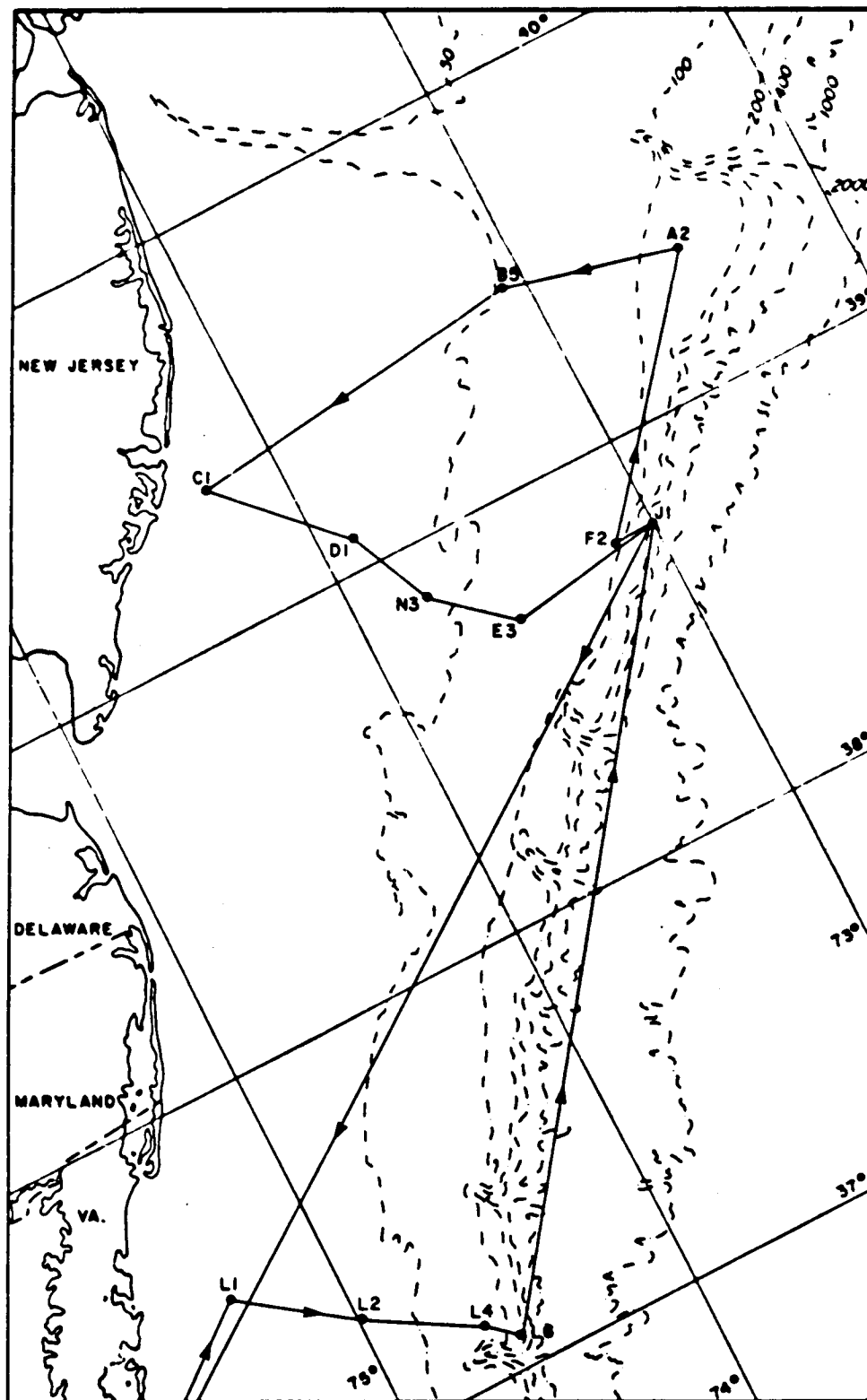
Figure 2-43. Cruise track, R/V H. J. W. Fay , BLM08W, 19-30 August 1977.
