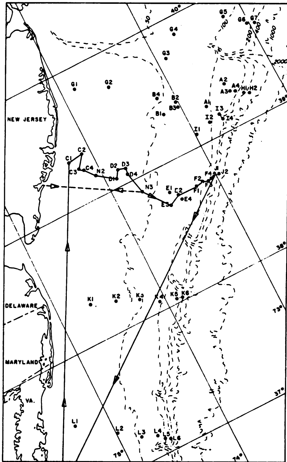
Figure 2-14. Cruise track, R/V G. W. Pierce , BLM02B, Benthos Leg 1, 19-26 February 1976.
