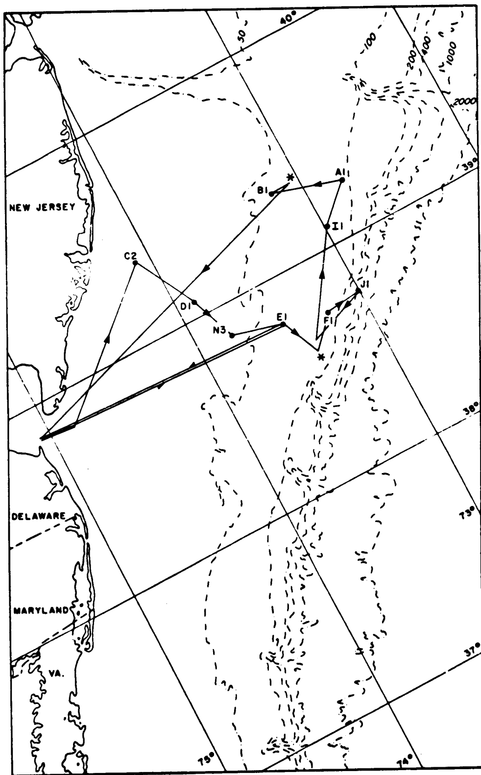
Figure 2-33. Cruise track, R/V Cape Henlopen , BLM05T, 8-18 November 1976. *See Figures 2-25 and 2-27 for megabenthic habitat delineation sites.
