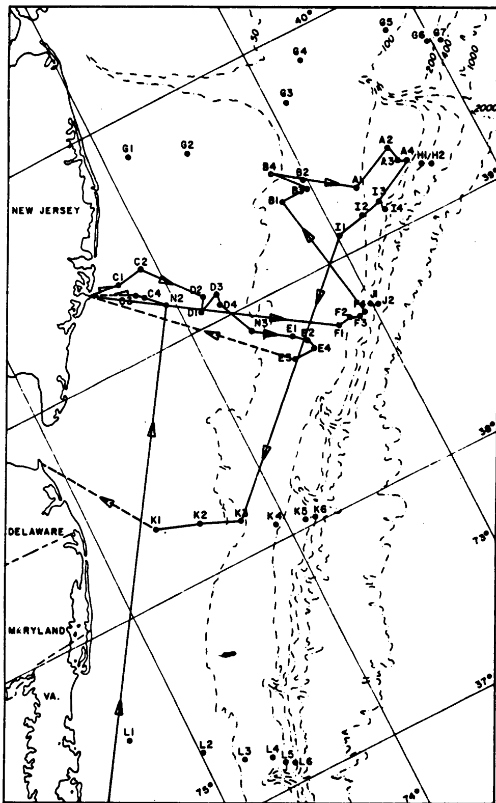
Figure 2-19. Cruise track, R/V G. W. Pierce , BLM04B, Leg 1, 14-24 August 1976.
