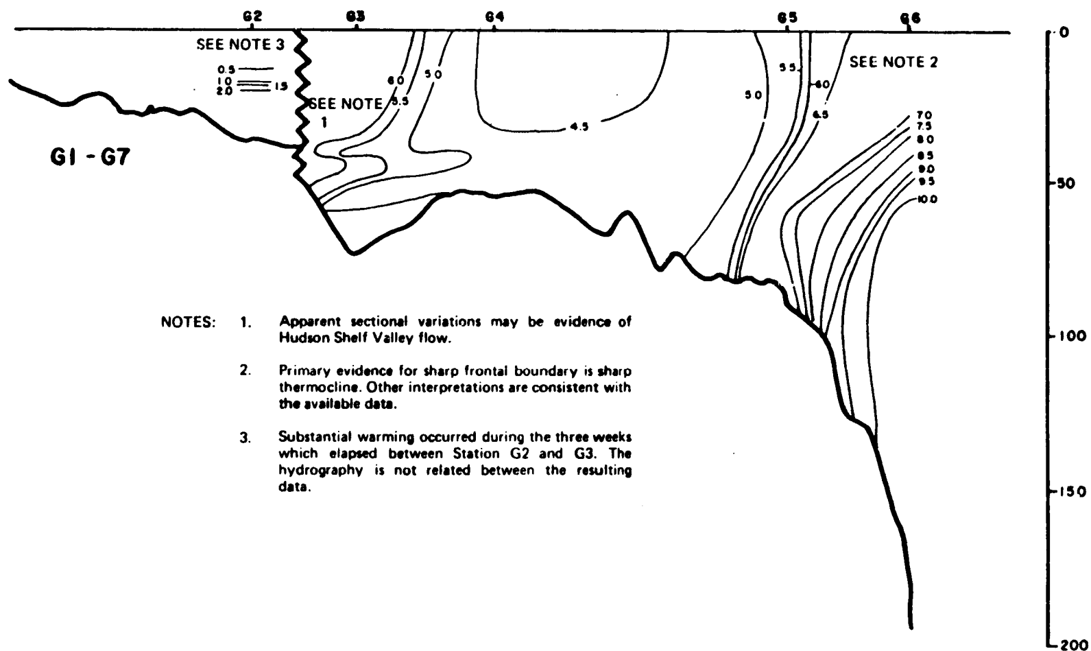
Figure 3-28a. Temperature (°C) contours for section I (Figure 3-6) during cruise BLM06B. Station locations on the section and designations are indicated at the top of the section. Depths are in meters.
