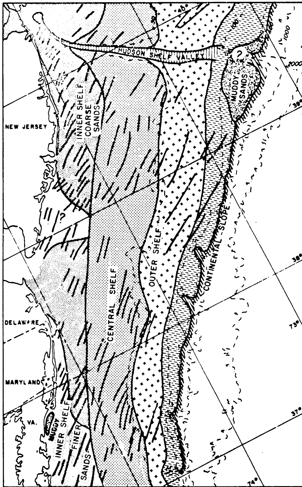
Figure 22. Schematic zonation of macrobenthic biotopes in the middle portion of the Middle Atlantic Bight. Major ridge fields are indicated.
