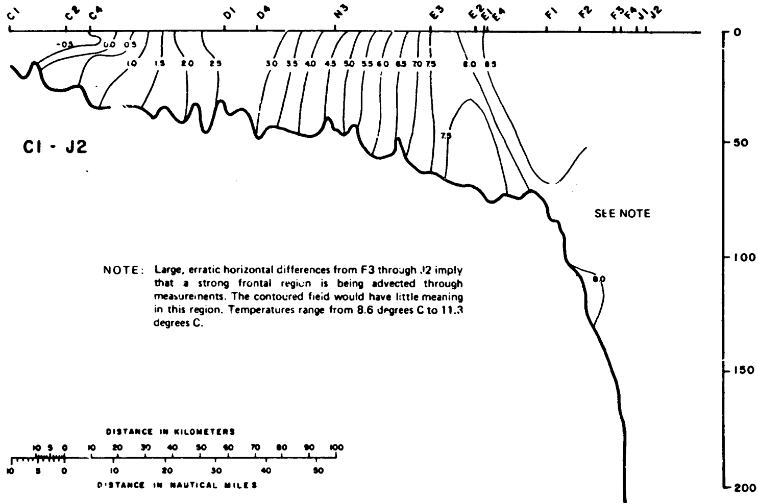
Figure 10. Temperature ( ^{\circ}\text{C} ) contours for section III (Figure 3-6) during cruise RLM06B. Station locations on the section and designations are indicated at the top of the section. Depths are in meters.
