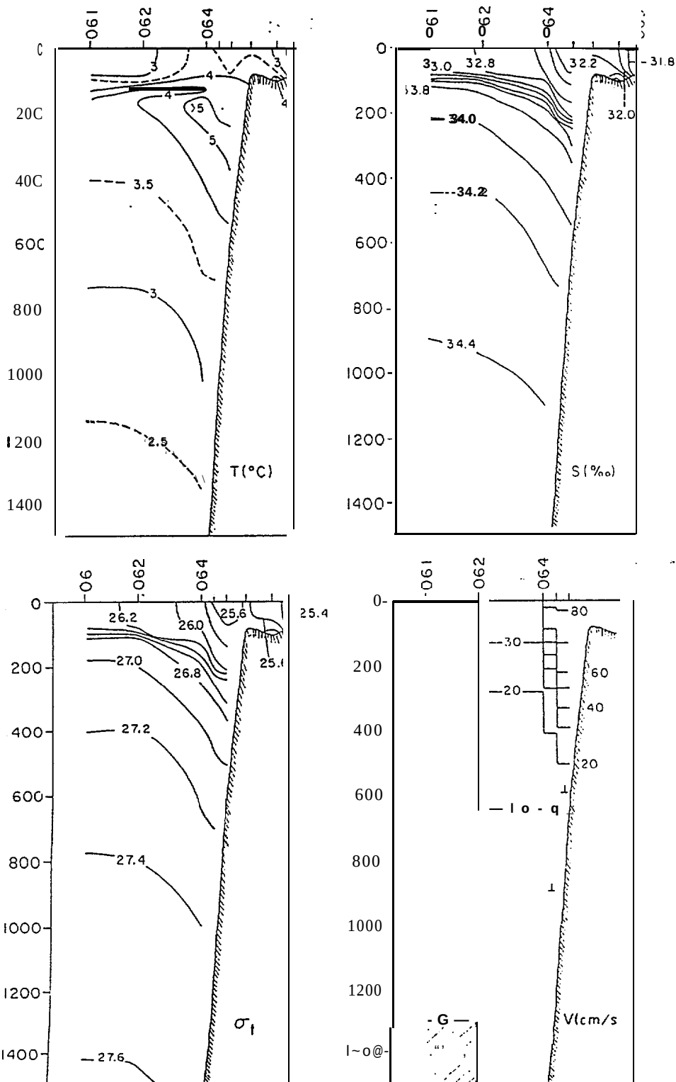
Figure 4F-4. Vertical sections of temperature ( ^{\circ}\text{C} ), salinity (ppt), Sigma t density, and geostrophic flow (cm/see, referred to 1500 db) across the Alaska Stream at approximately 16.4^{\circ}\text{W} , 24-25 February, 1980 (from Reed and Schumacher 1986).
