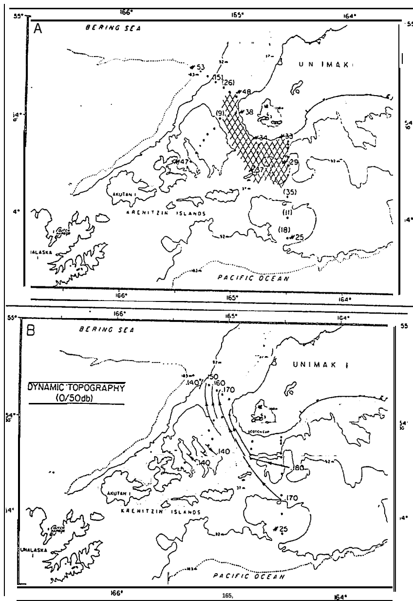
Figure 4F-8. Hydrographic data for September 1981 presented as (a) areal extent of waters with salinity \leq 31.75 m/kg in the upper 50 m (or bottom) where the numbers in parentheses are depths of the low salinity bank for z < 50 m and (b) dynamic topography (0/50db) with a 0.01 dyn m contour interval. CTD station numbers are indicated by the number sign (from Pearson et al. 1980).
